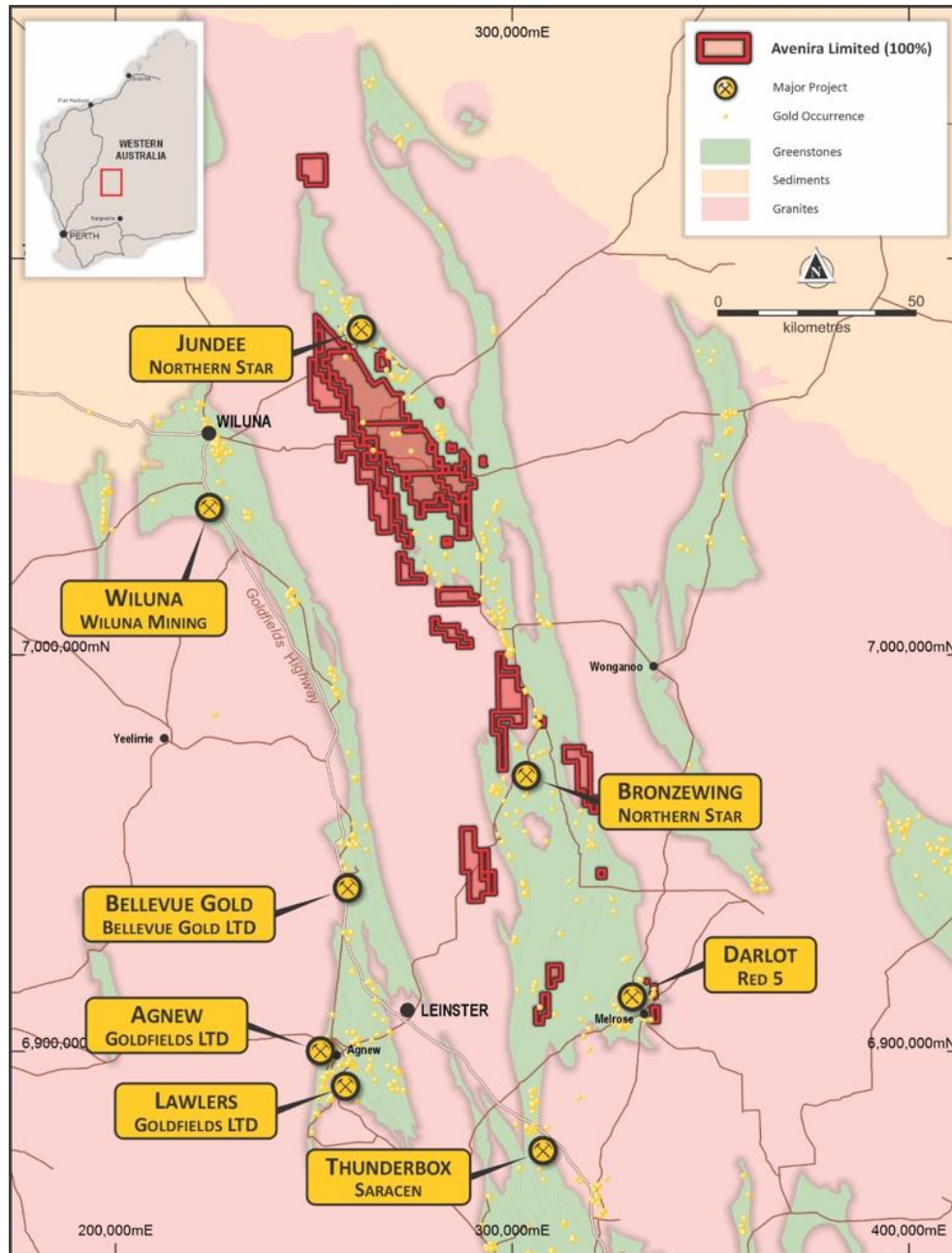
FIGURE 3: Location map of Mineral Titles of the Jundee South Project
