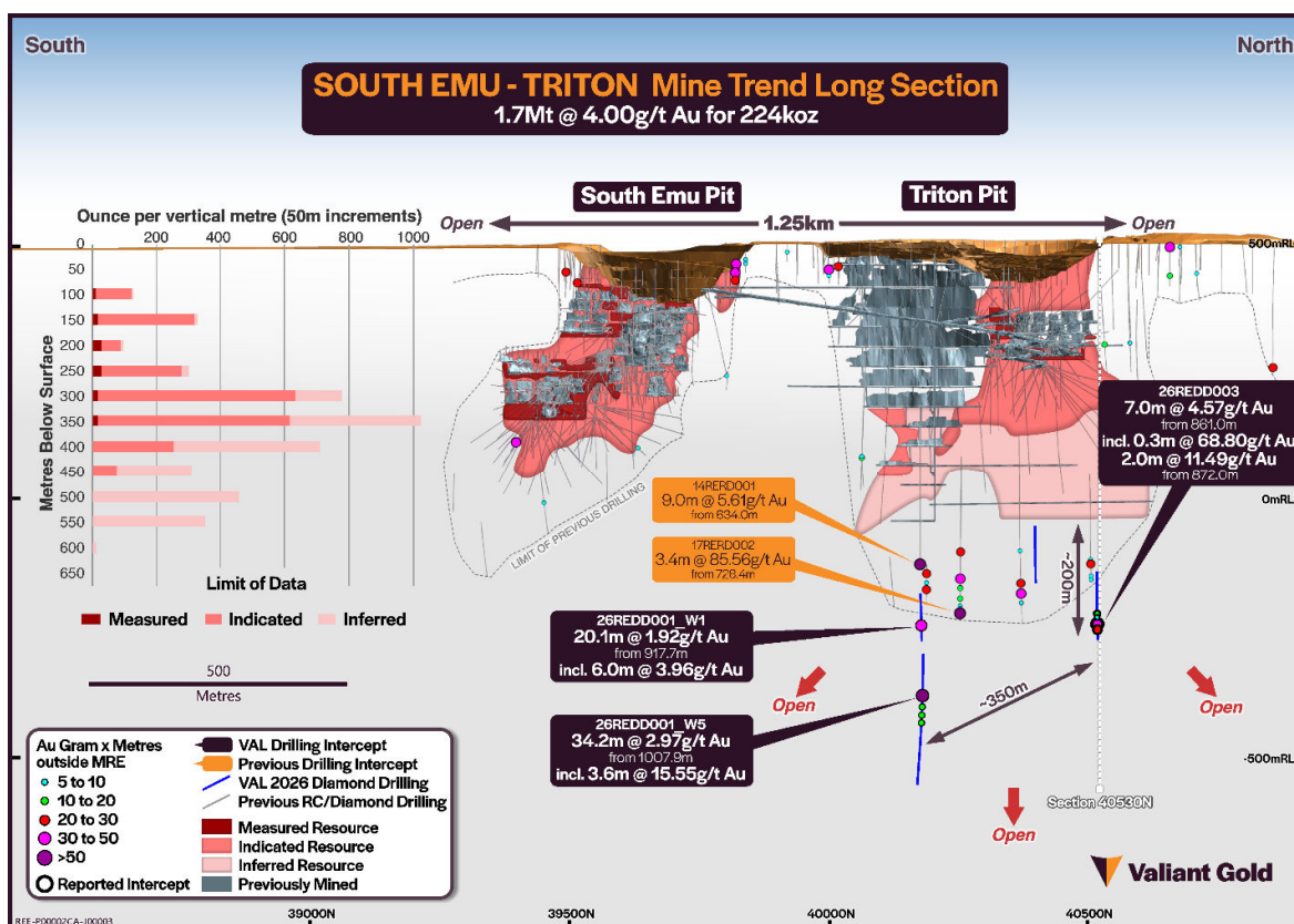
Figure 5. South Emu-Triton schematic long section, facing west, displaying the Mineral Resource Estimate ('MRE') with previously mined volumes and drill intercepts, including results received after 30 June 2026 1
