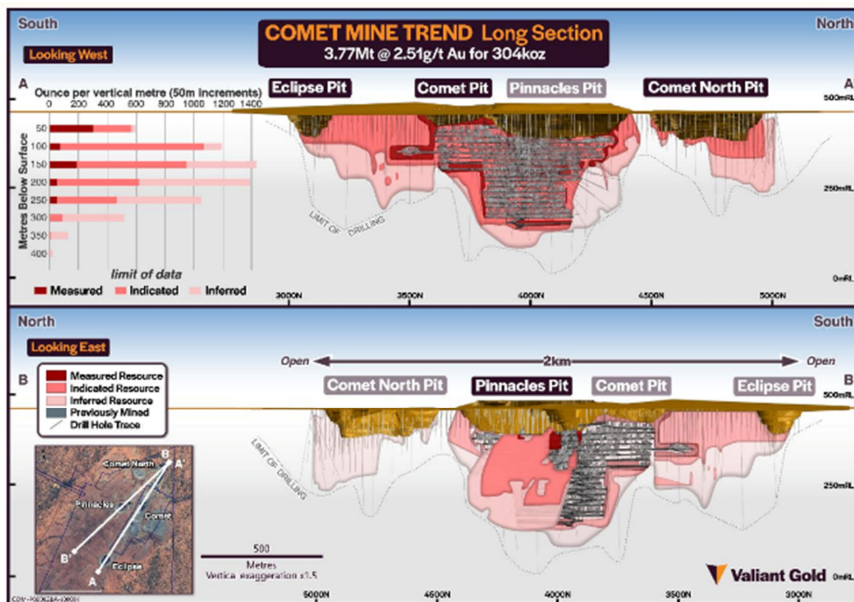
Figure 3. Comet Mine Trend schematic long section, looking west (top) and east (bottom), showing the Mineral Resource Estimate, ounce-per-vertical metre distribution and previously mined volumes 1
