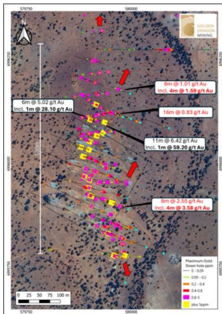
Figure 3 Previous high-grade downhole gold intersections at the Coodardy Prospect, with intersections >5 g/t Au highlighted in yellow. Previously reported intersections within the interpreted northeast-trending high-grade shoot have been resampled and re-assayed at 1m intervals (black text). Significant gold intersections from most recent drilling are shown in red text, with drill collars shown in light blue.
