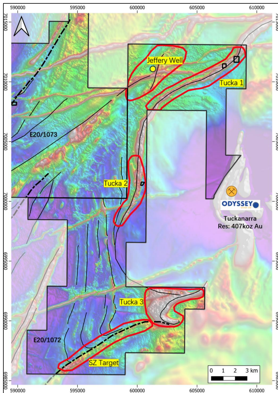
Figure 6 Newly granted E20/1072 highlighting the five regional-scale targets and the Jeffery well Prospect
