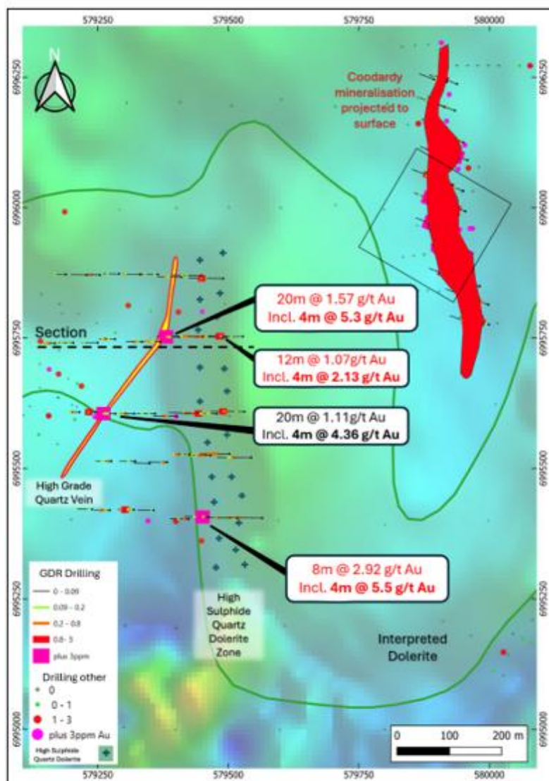
Figure 4 Highlighting significant intersections from inaugural drilling (black text) and second phase drilling (red text).
