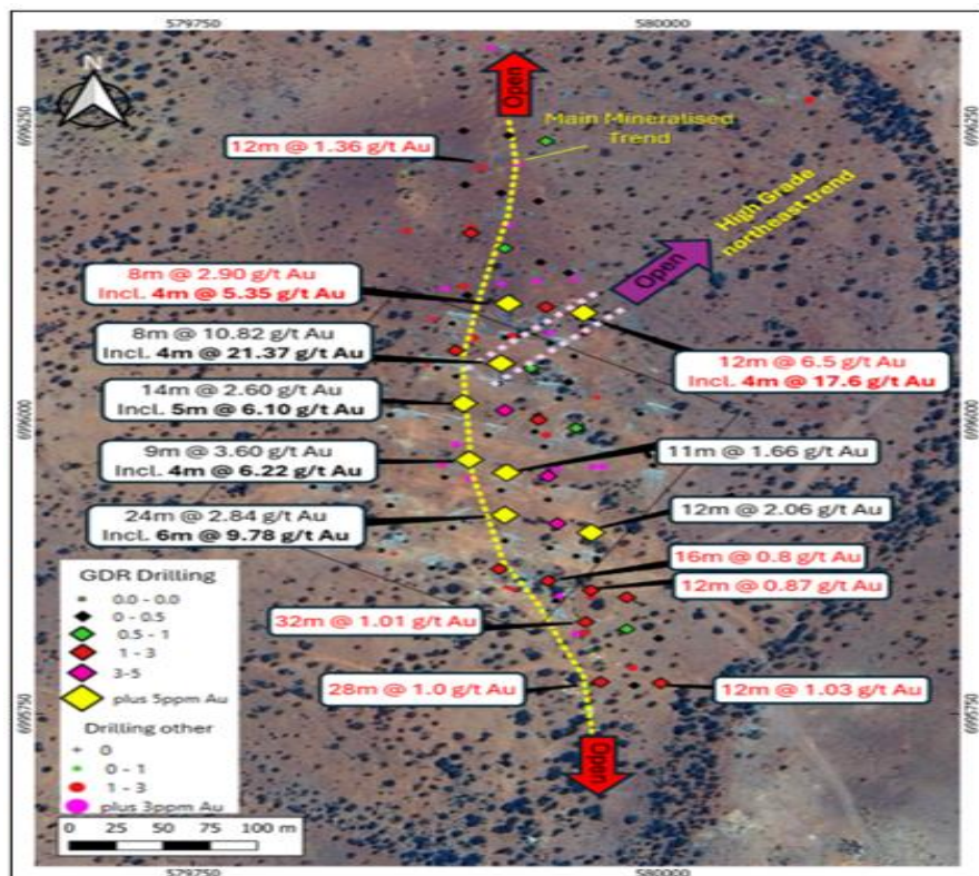
Figure 2 Plan view showing new significant drill intersections GDR drilling phase one (black text) phase 2 (red text) highlighting the north south mineralised trend and the newly identified northeast orientation
