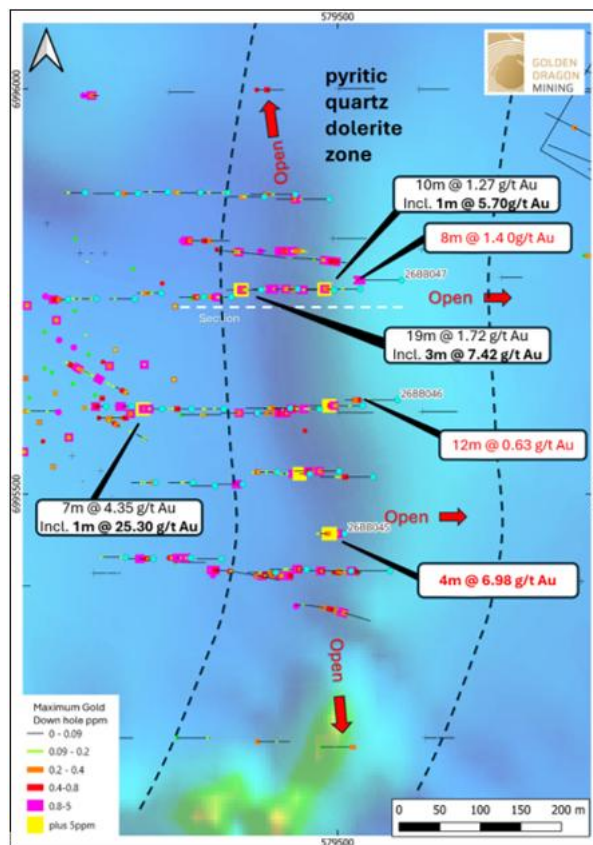
Figure 5 High-grade downhole gold intersections at the Behring Bore Prospect, with intersections >5 g/t Au highlighted in yellow. Previously reported high-grade intervals have been resampled and re-assayed at 1m intervals (black text). Significant gold intersections from recent drilling are shown in red text, with drill collars shown in light blue. (TMI magnetics image background).
