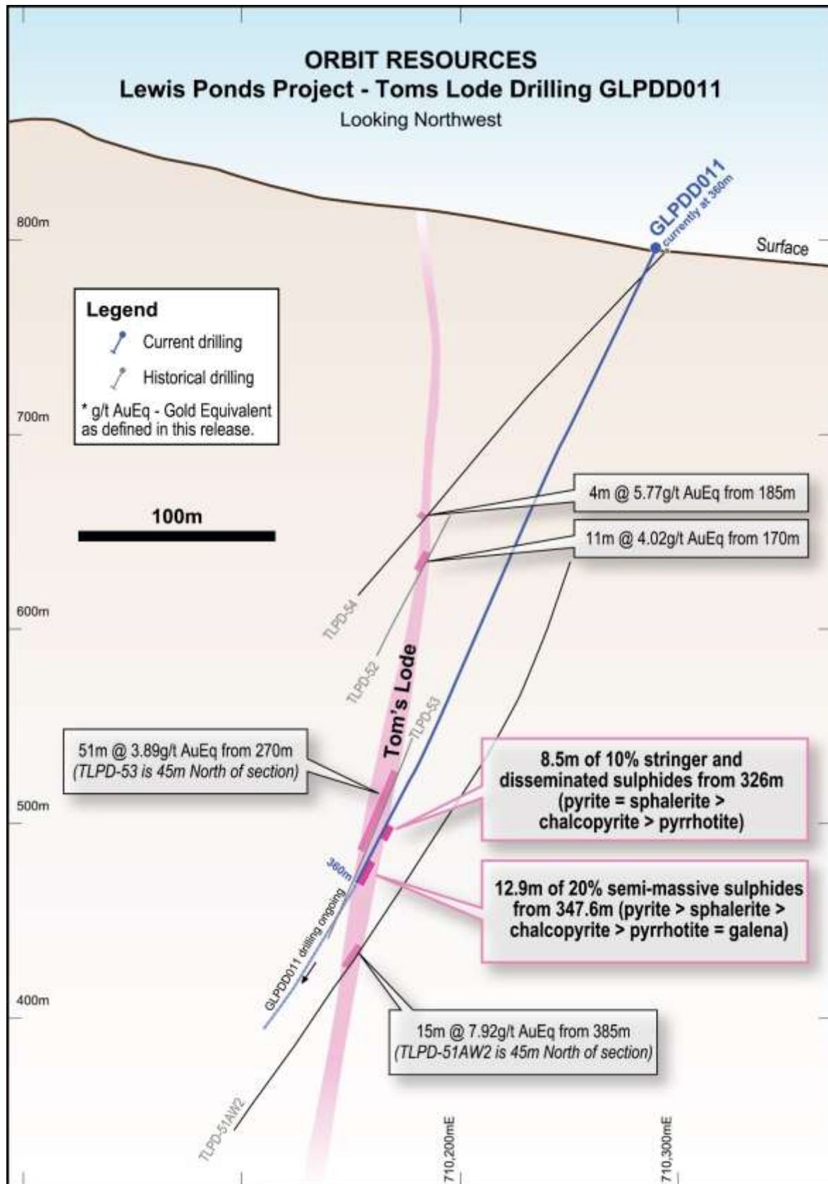
Figure 2: Cross section showing the visual sulphide abundances of Tom's Lode orebody encountered in GLPDD011. GLPDD011 is currently at 360m and will be continued to 50m beyond the mineralised envelope. Also shown are historical drill intercepts within Tom's Lode.
