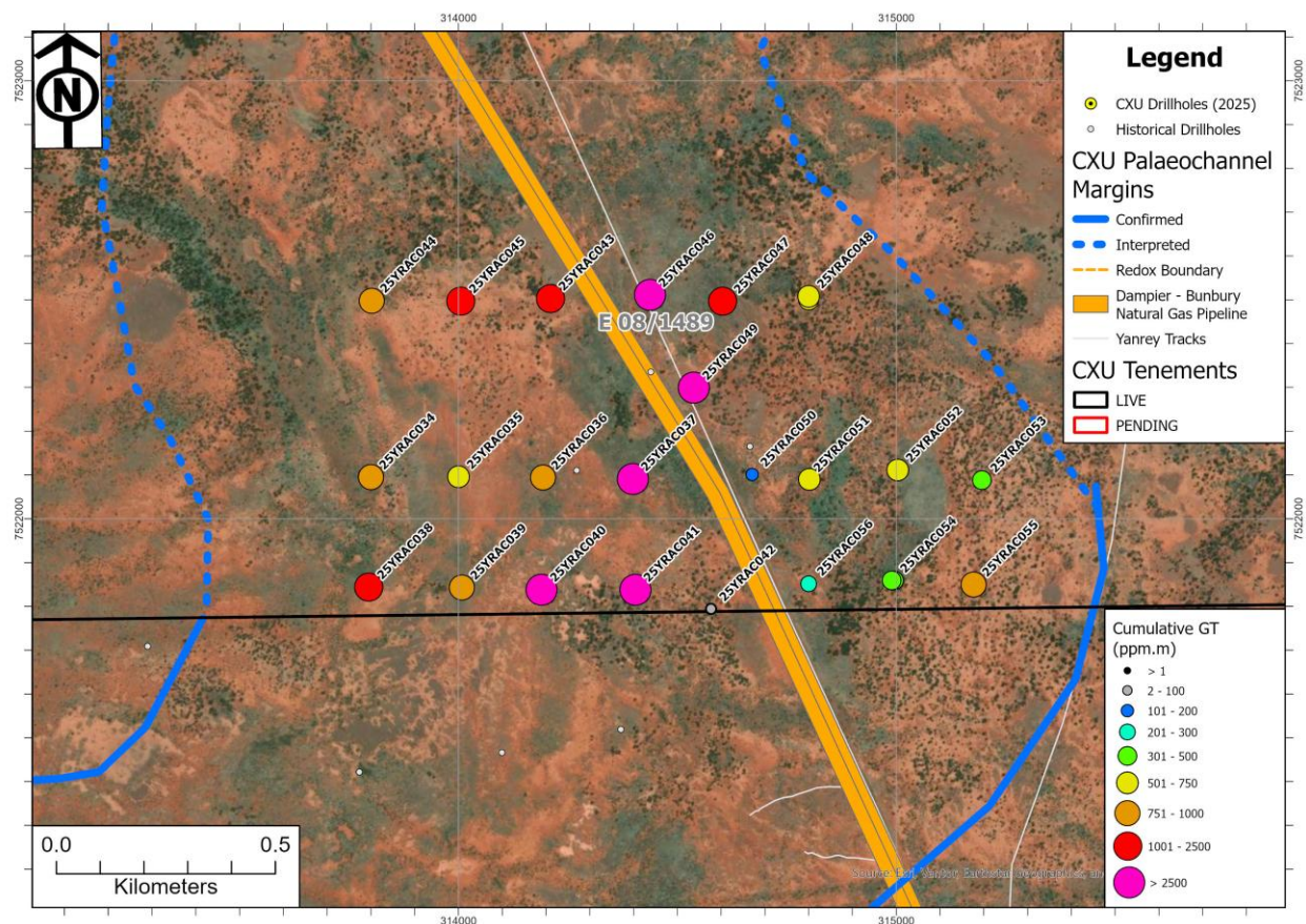
Figure 5: Manyingee North Cumulative GT (ppm*m) map.
