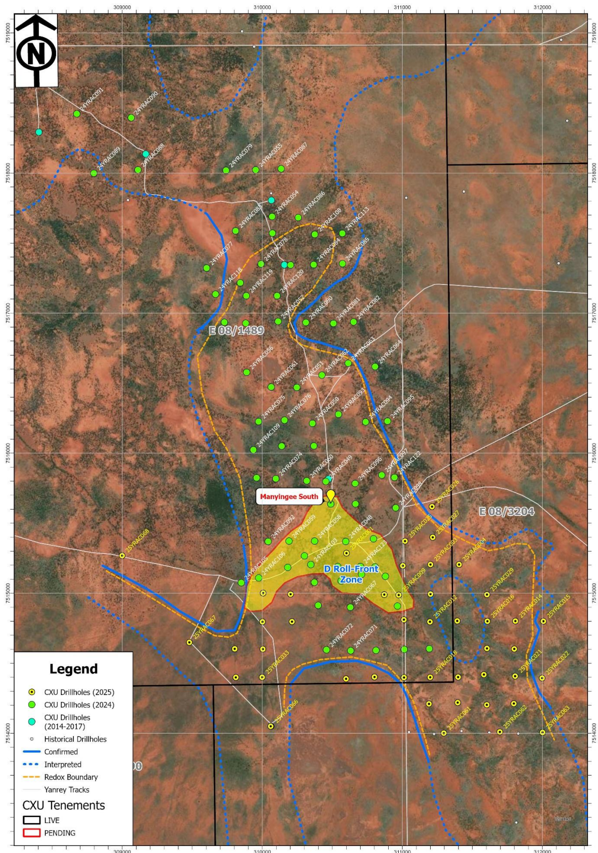
Figure 3. Manyingee South drillhole locations showing the location of the high-grade zone.
