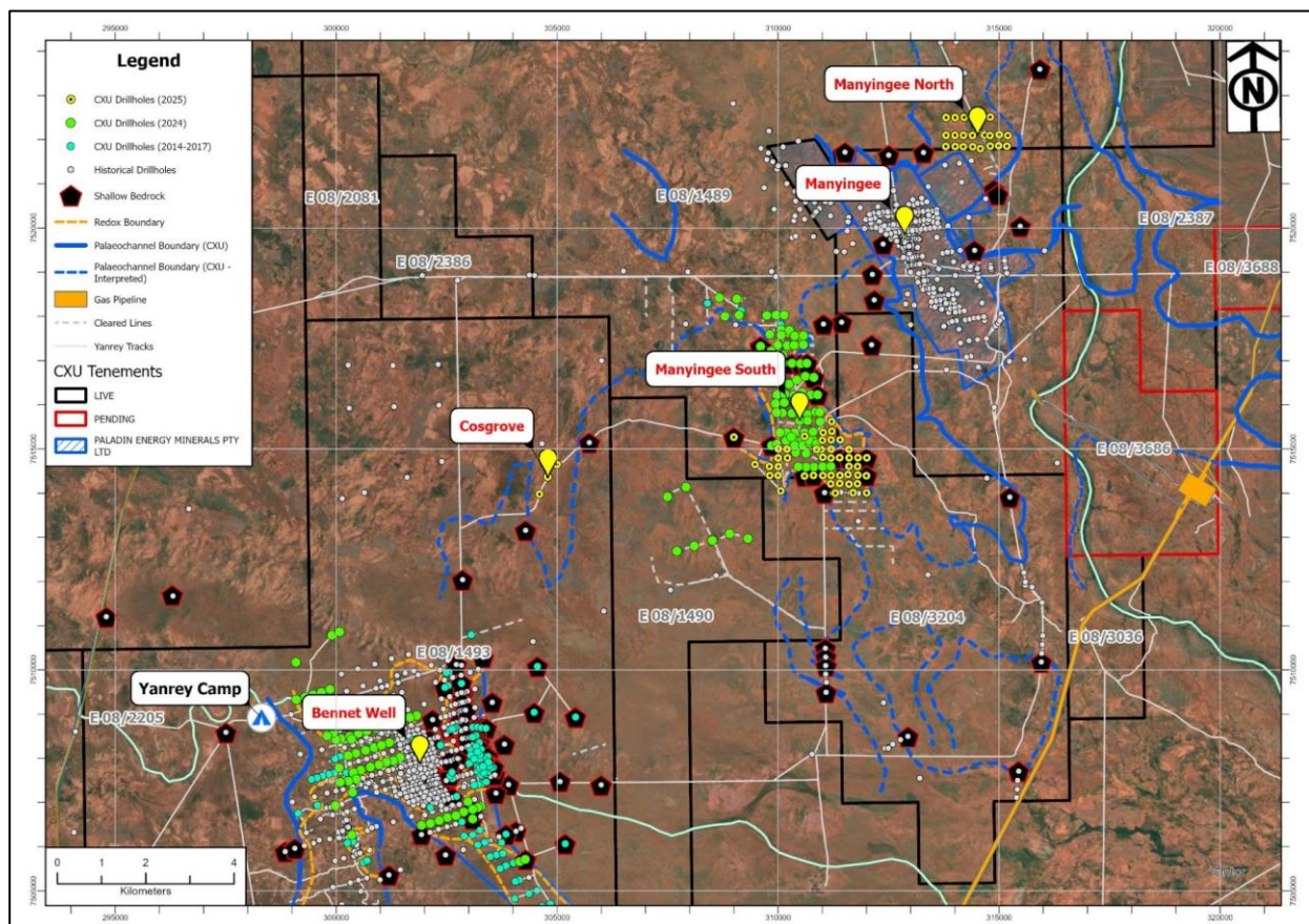
Figure 2: Map of the Yanrey Uranium Province showing uranium deposits and recent and historical drilling within the interpreted early cretaceous palaeo-drainage network
