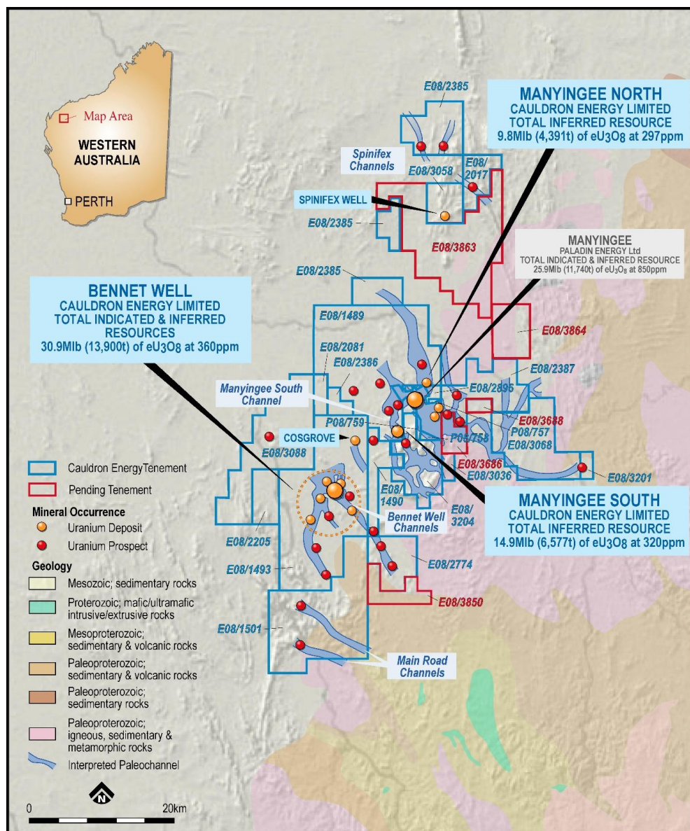
Figure 1: Yanrey Uranium Project Location showing regional geology
