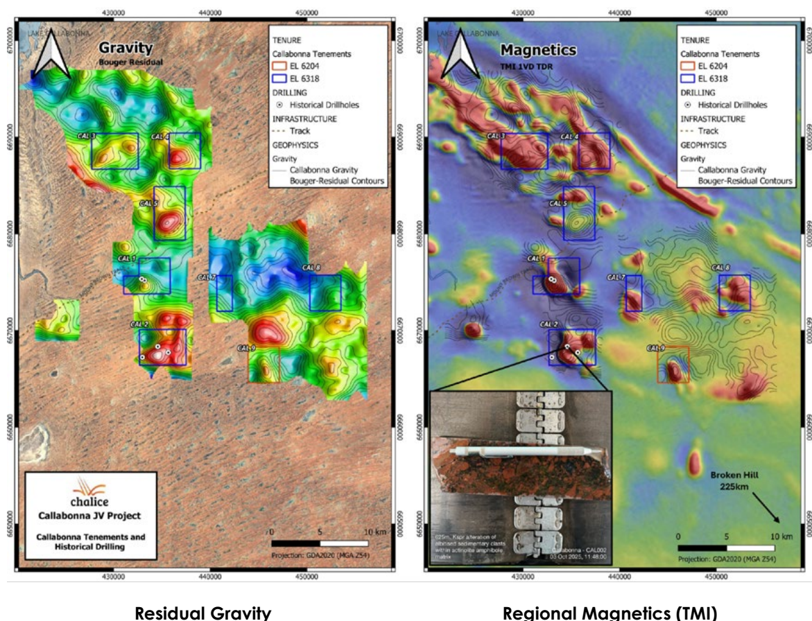
Figure 11. Callabonna regional residual gravity (LHS) and magnetics (TMI, RHS).
