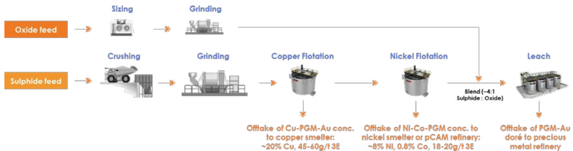
Figure 3. Gonneville Project Process Flowsheet (simplified).
