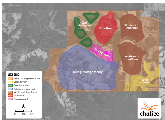
Figure 4. Gonneville MDA preliminary site layout.
