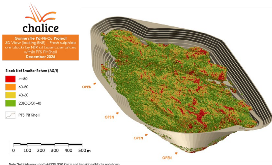
Figure 2. 3D view (looking ENE) of the fresh sulphide ore blocks by NSR within the modelled pit.
