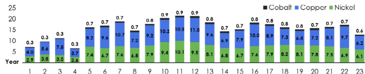
Figure 6. Gonneville base metal production profile (kt, recovered).
