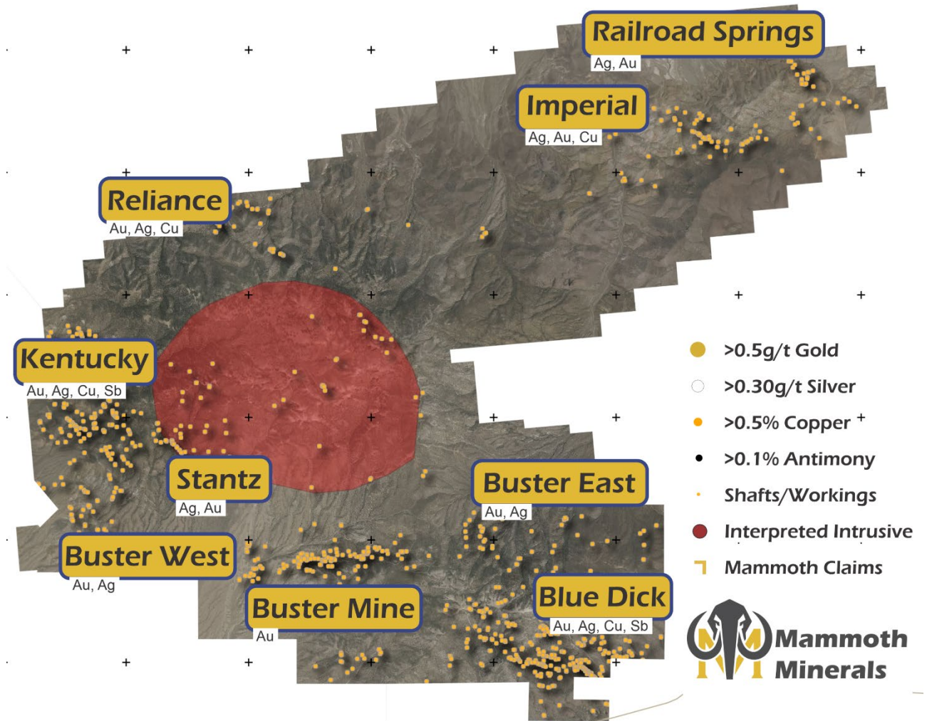
Figure 1: Excelsior Springs overview Map showing prospect zones
