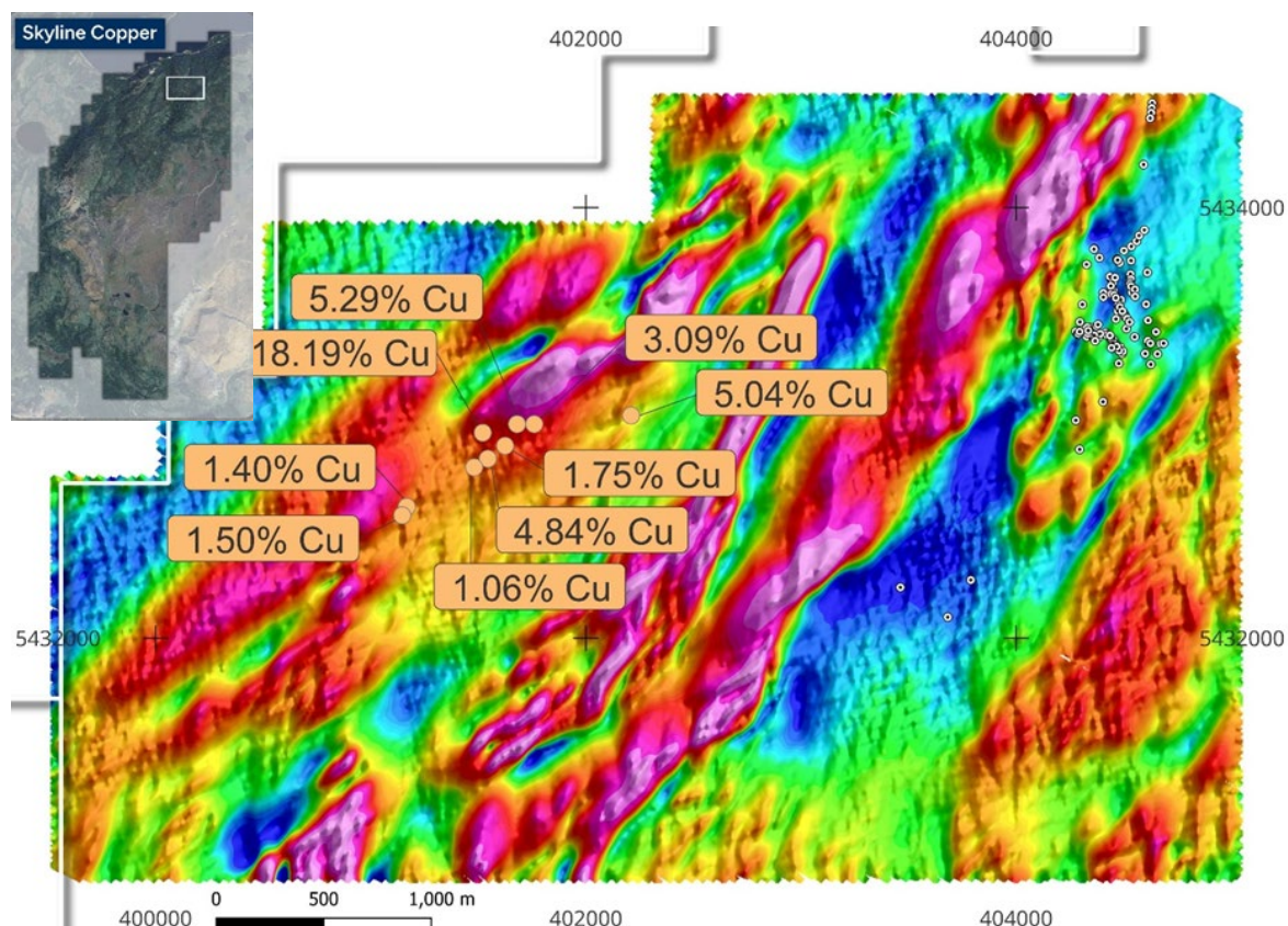
Figure 8: High-resolution magnetics over northern Skyline Tenure with prospecting copper results.
