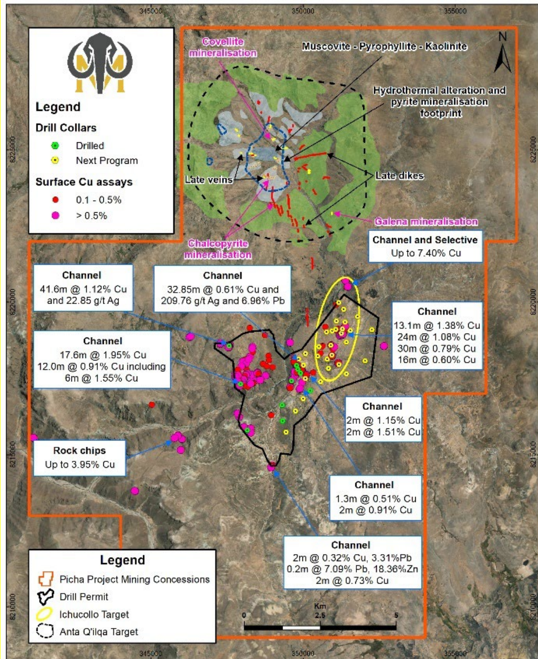
Figure 11: Mapping, Rock chips and channel samples across Picha Project
