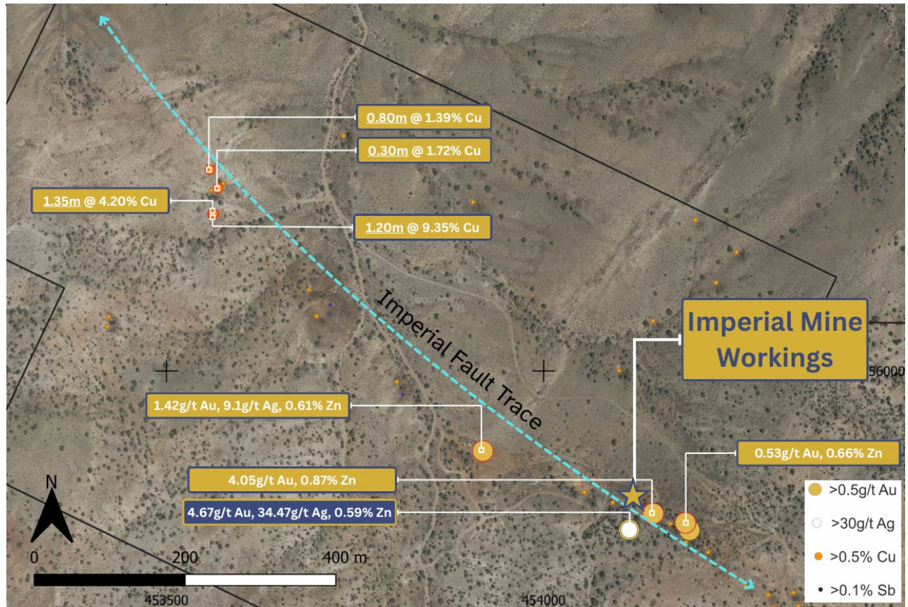
Figure 4: Results of sampling along strike of Imperial Fault, which hosts historical Imperial Mine
