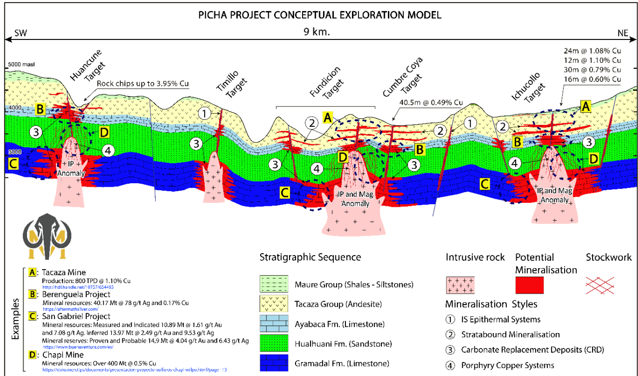
Figure 10: Conceptual cross-section of the Picha Project showing potential mineralisation styles and host stratigraphy
