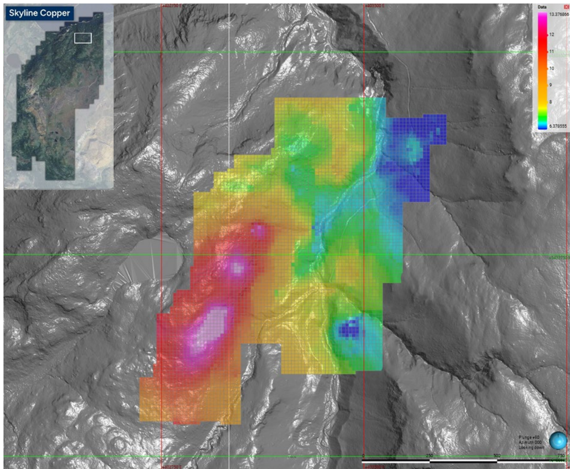
Figure 9: Induced Polarisation results over LiDAR topography across Governor's Target, Skyline Project.
