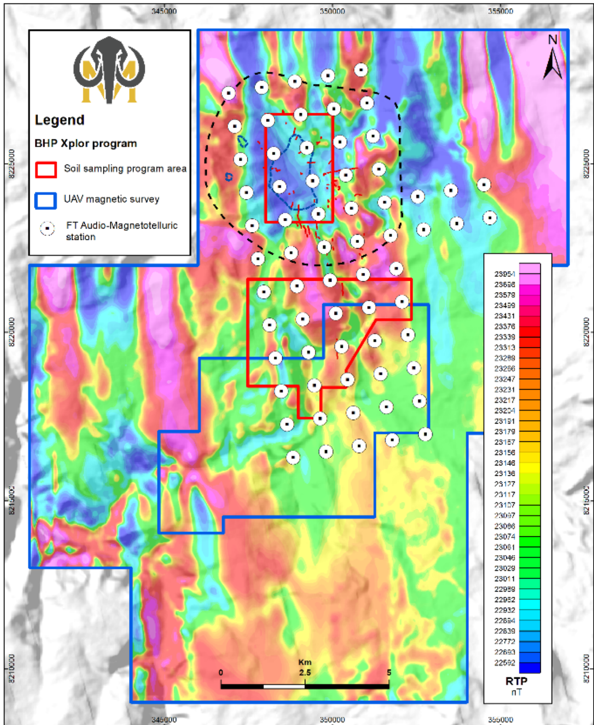
Figure 12: UAV magnetics showing Low magnetics across target areas and lines/stations of MT survey
