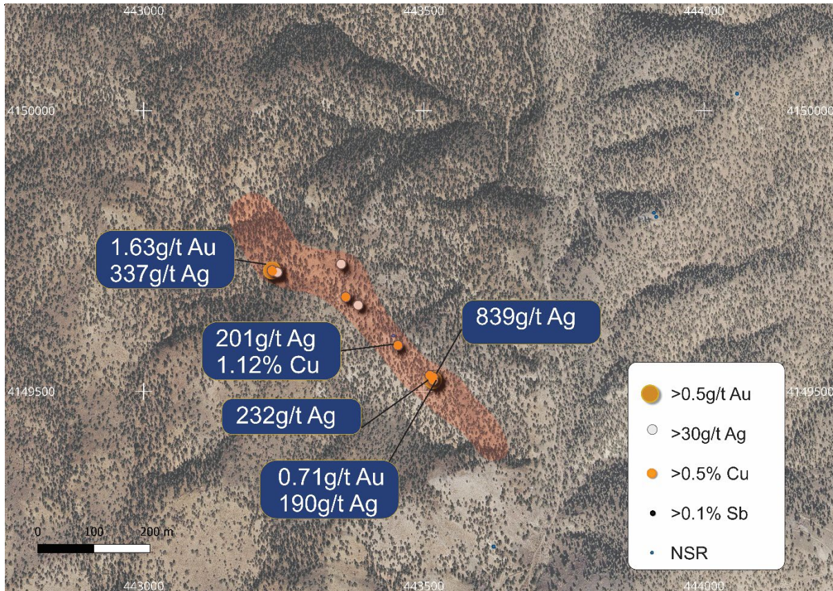
Figure 6: Rock chip sampling along the Stantz Trend.
