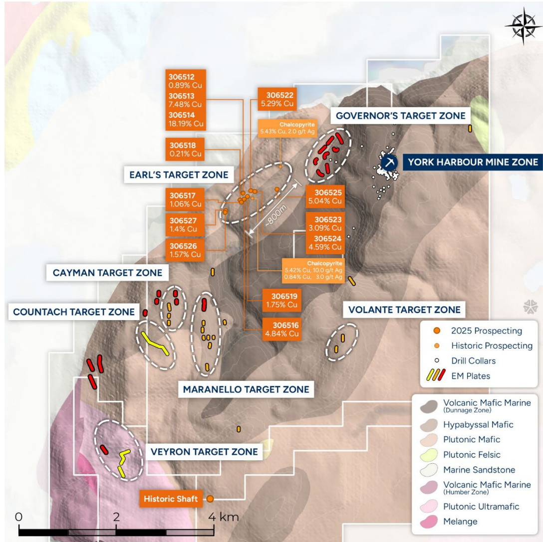
Figure 7: EM and Geochem targets across northern Skyline Property
