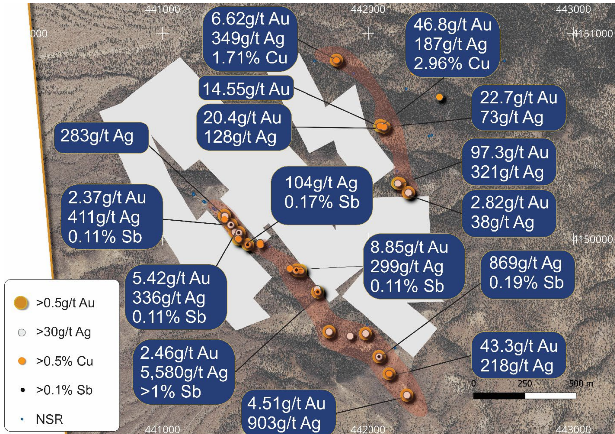
Figure 5: Rock chip sample results from the Kentucky Prospect highlighting multiple trends
