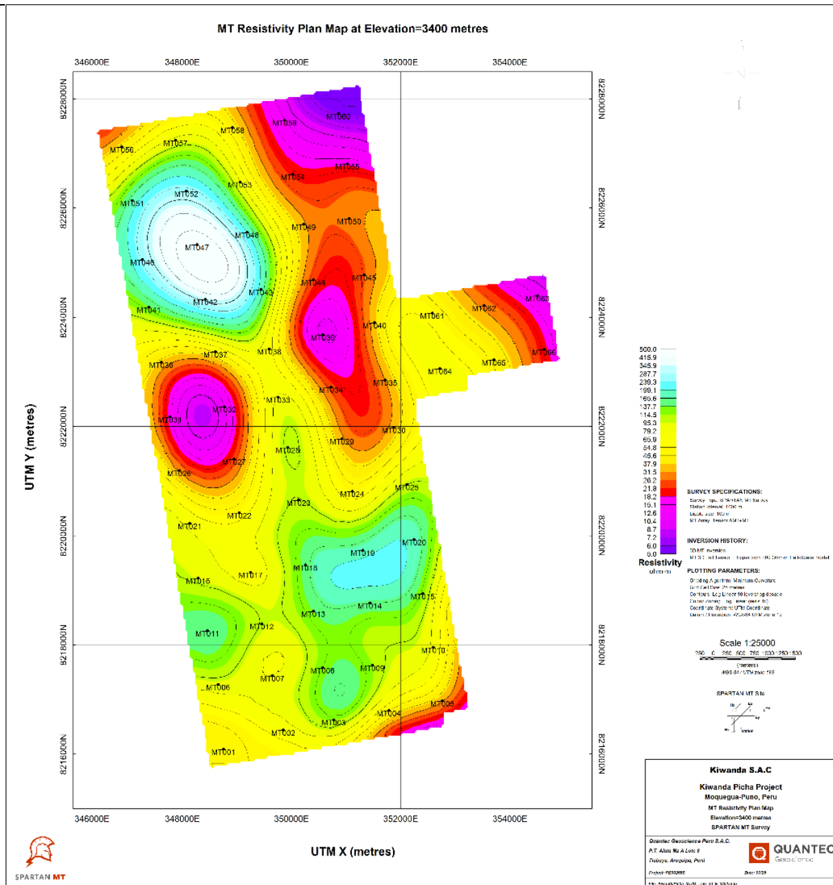
Figure 13: MT survey results showing resistivity highs across the Anta Q'ilqa and Ichucollo targets
