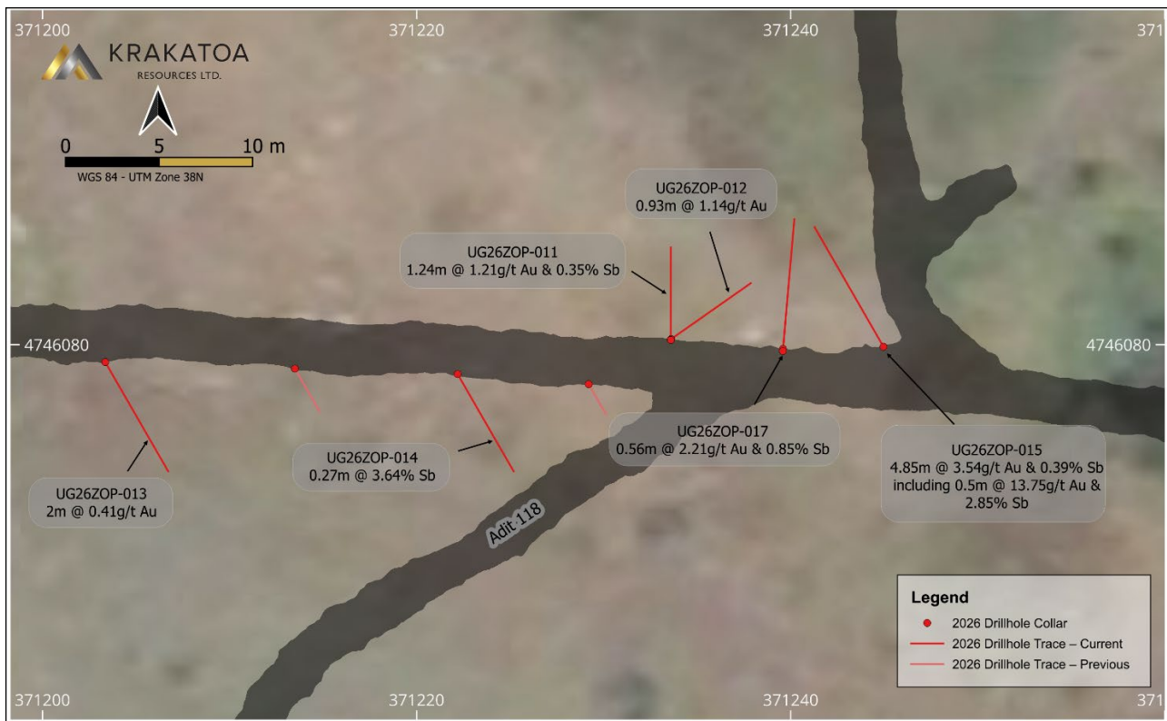
Figure 2 Map of UG drill holes with significant grades – adit 118 V50 zone
