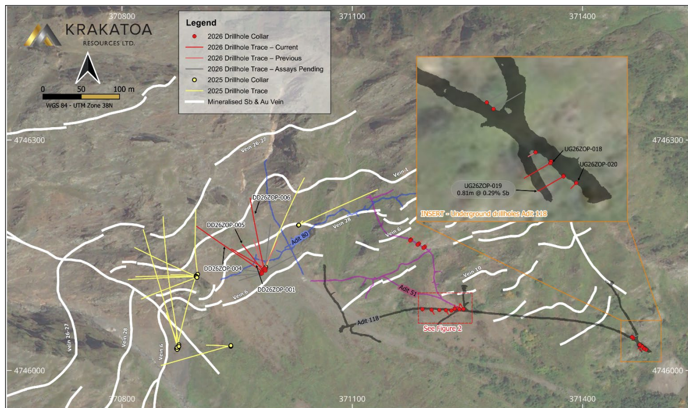
Figure 1 Map of all drillhole locations with adit (LiDAR survey) wireframes.
