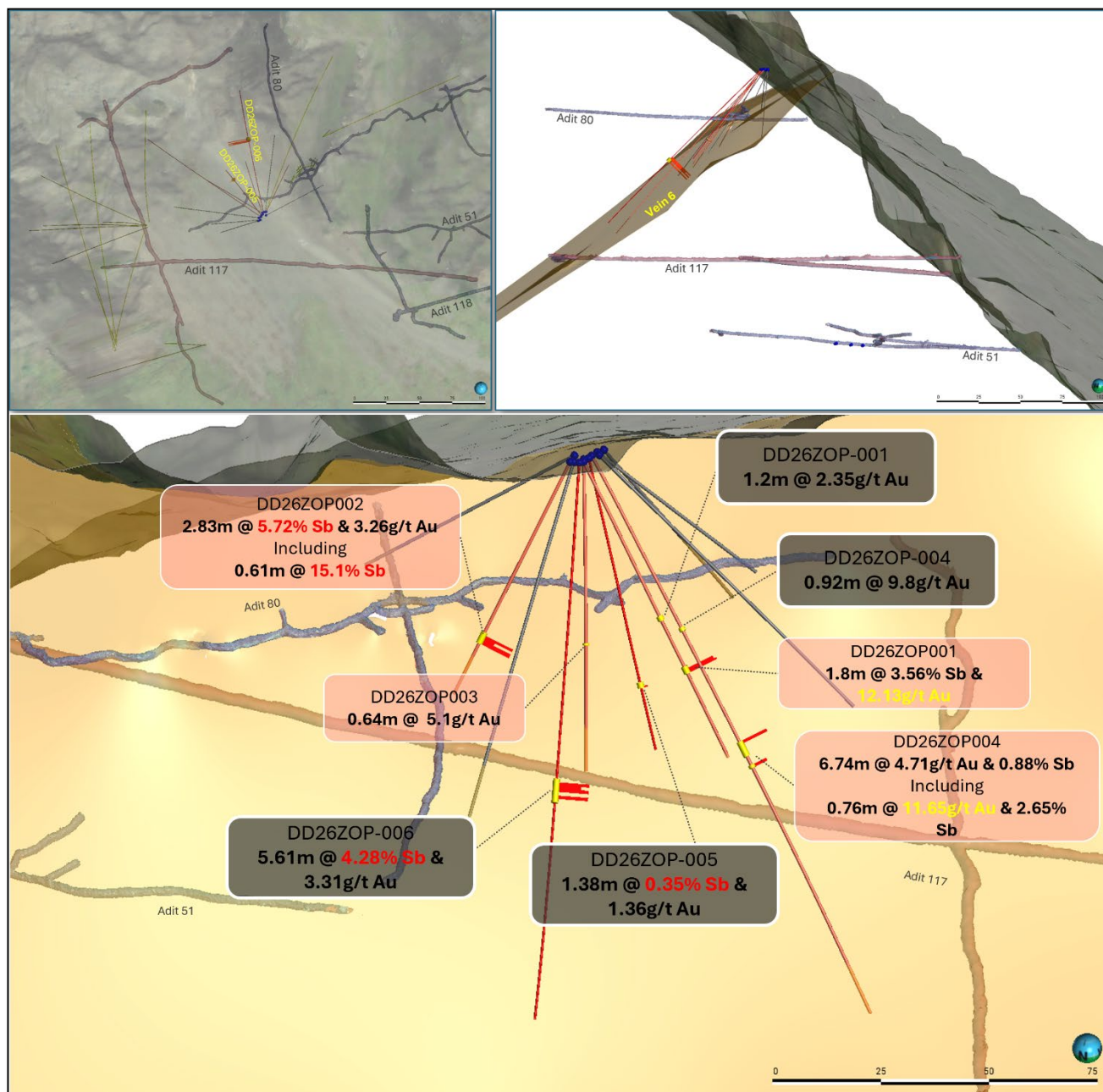
Figure 4 Surface Drillhole assay results showing significant mineralisation. Top Left - plan view of assayed surface drilled holes showing drill trace of 2025 drill holes (grey); Top Right – Cross section through area showing modelled vein profile, adits and drill holes; Bottom – Oblique view looking SE (out of mountain) at drill holes with detailed assay results from 2026 laboratory analysis.
