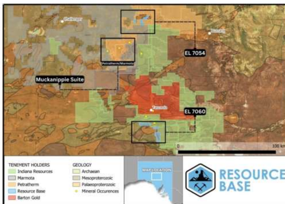
Figure 1: Location of EL7054 and EL7060 within the Gawler Craton
