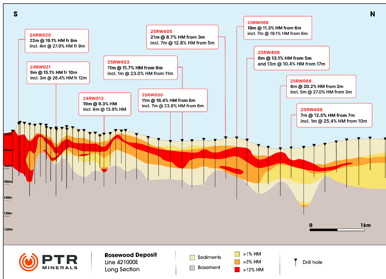
Figure 3: Rosewood S-N long section line 421000mE highlighting its high-grade and continuity.
