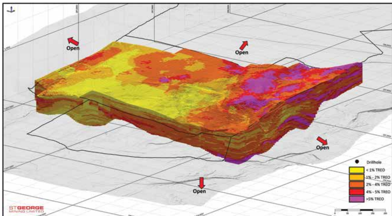
Figure 3: 3D perspective of Araxá MRE - Nb 2 O 5 grades (looking north-east)
