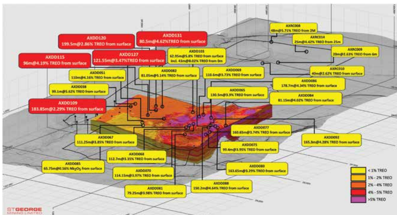
Figure 1: oblique section showing some of the diamond drill holes completed by St George. The drill holes identified by red labels were reported on 1 July 2026.
