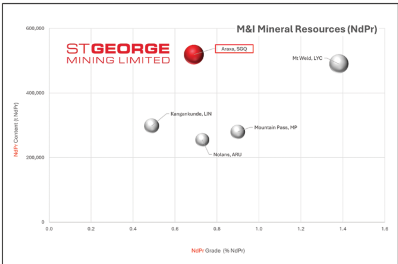
Figure 4: Comparison of contained NdPr oxides and grade within Measured & Indicated resources data of major hard-rock deposits in production or development. Source: Terra Studio.
