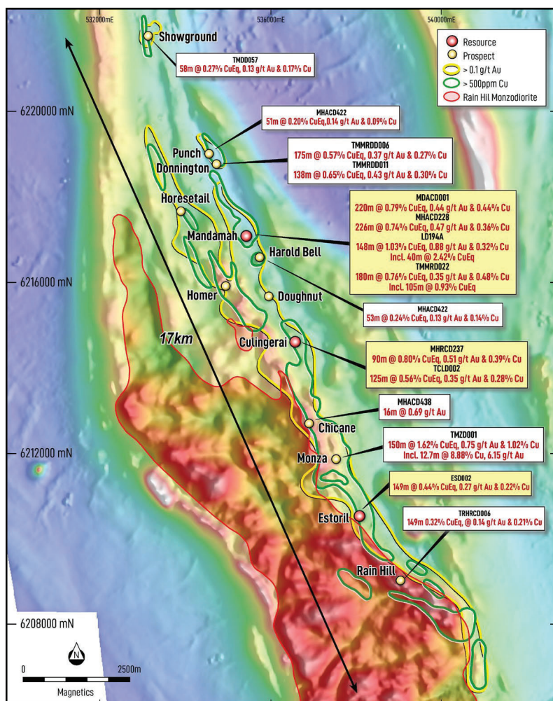
Figure 5: Central Zone resources and prospects over background reduced to pole aeromagnetic image highlighting a 17km strike.
