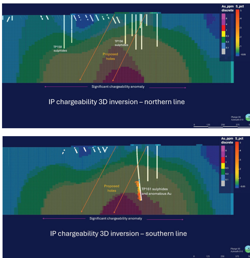
Figure 7: Cross section of the modelled IP data along IP line 1 (top) and IP line 2 (bottom) and proposed holes.
