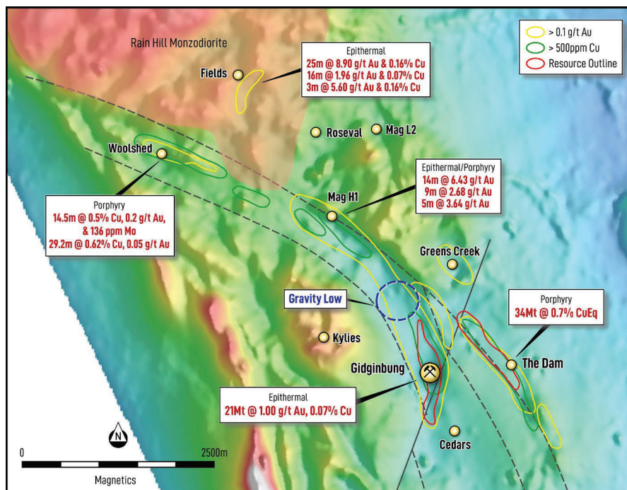
Figure 3: Southern Zone resources and prospects over background reduced to pole aeromagnetic image. Note the gravity low represents the Gidginbung North porphyry target. Gidginbung resource reported at a 0.5g/t Au cut off, Dam resource reported at a 0.4% CuEq cut off.
