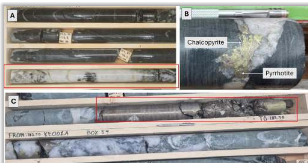
A) Quartz-carbonate veining, Killero Fault/Shear Zone (KE-001, 155m, ItQ Core); B) Chalcopyrite-pyrrhotite mineralisation (KE-001B, 37.9m); and C) Massive pyrrhotite and chalcopyrite in (KE-001A, 182.83 - 183.59m).
