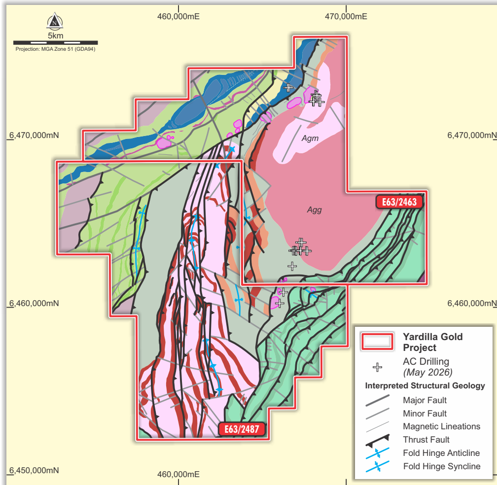
Bedrock interpretation map and Legend – Terra Resources
