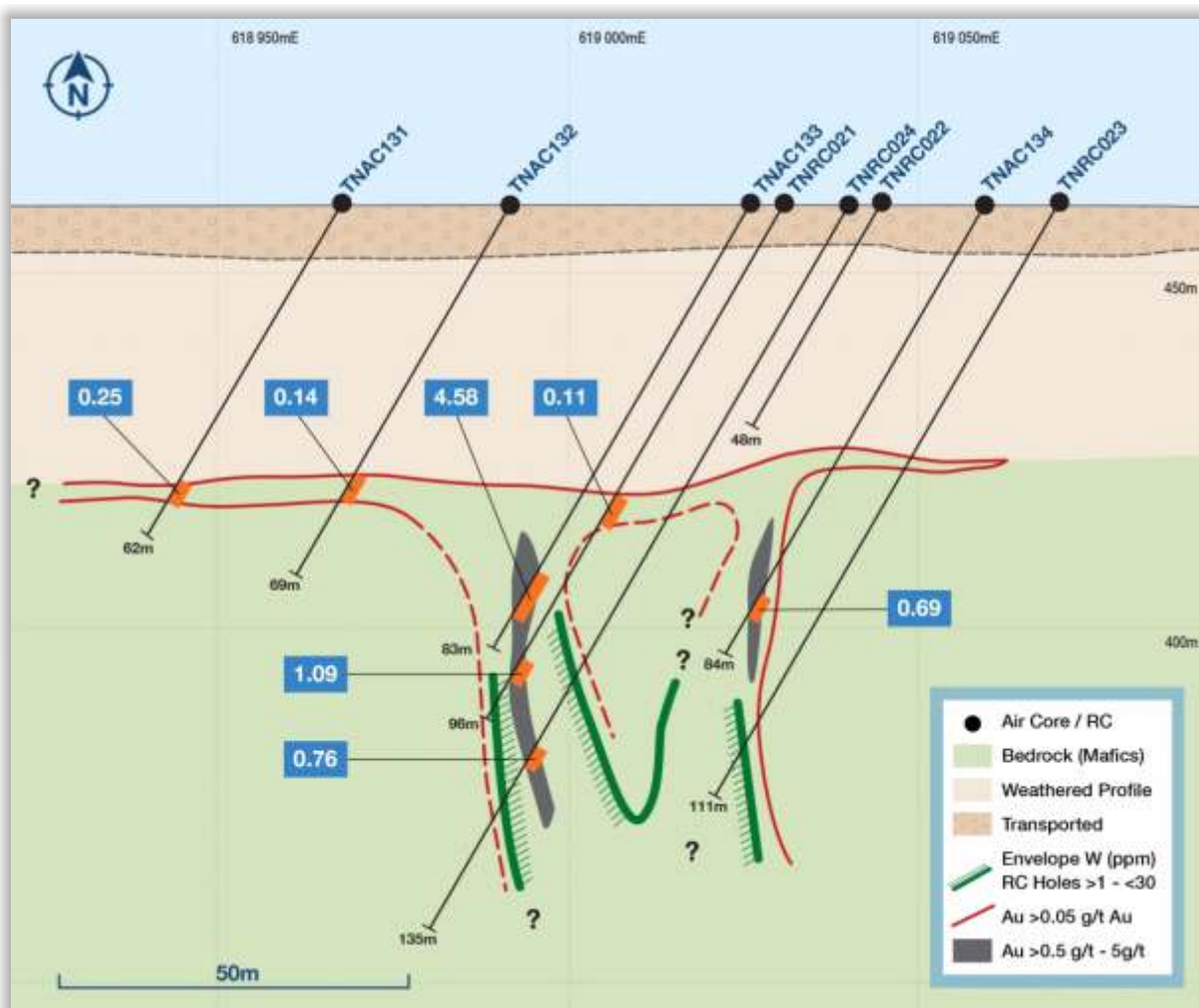
X-section 6972400mN an example of deeper targets along major NE trending structures at Tuckabianna North
