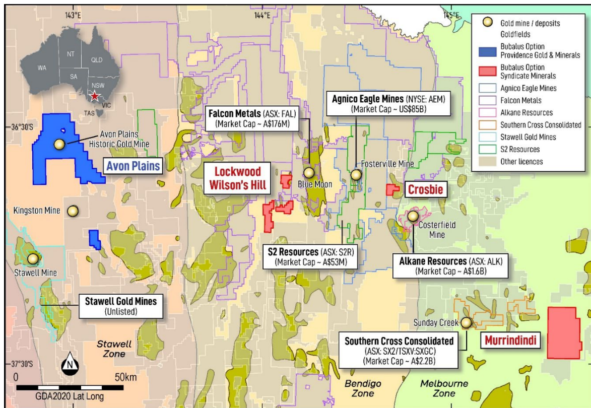
Figure 1: Location of key licences optioned by Bubalus during the period.
