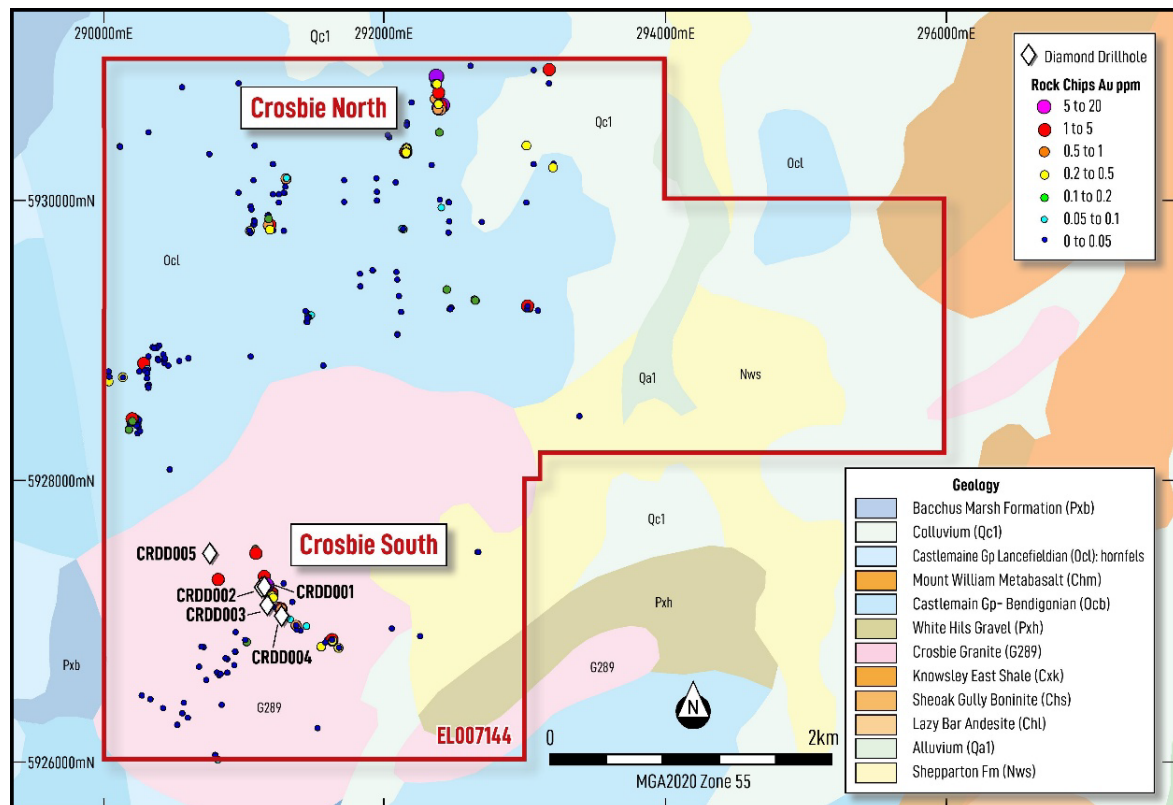
Figure 2: Crosbie Licence Geology, Surface sampling and Crosbie South Drilling.
