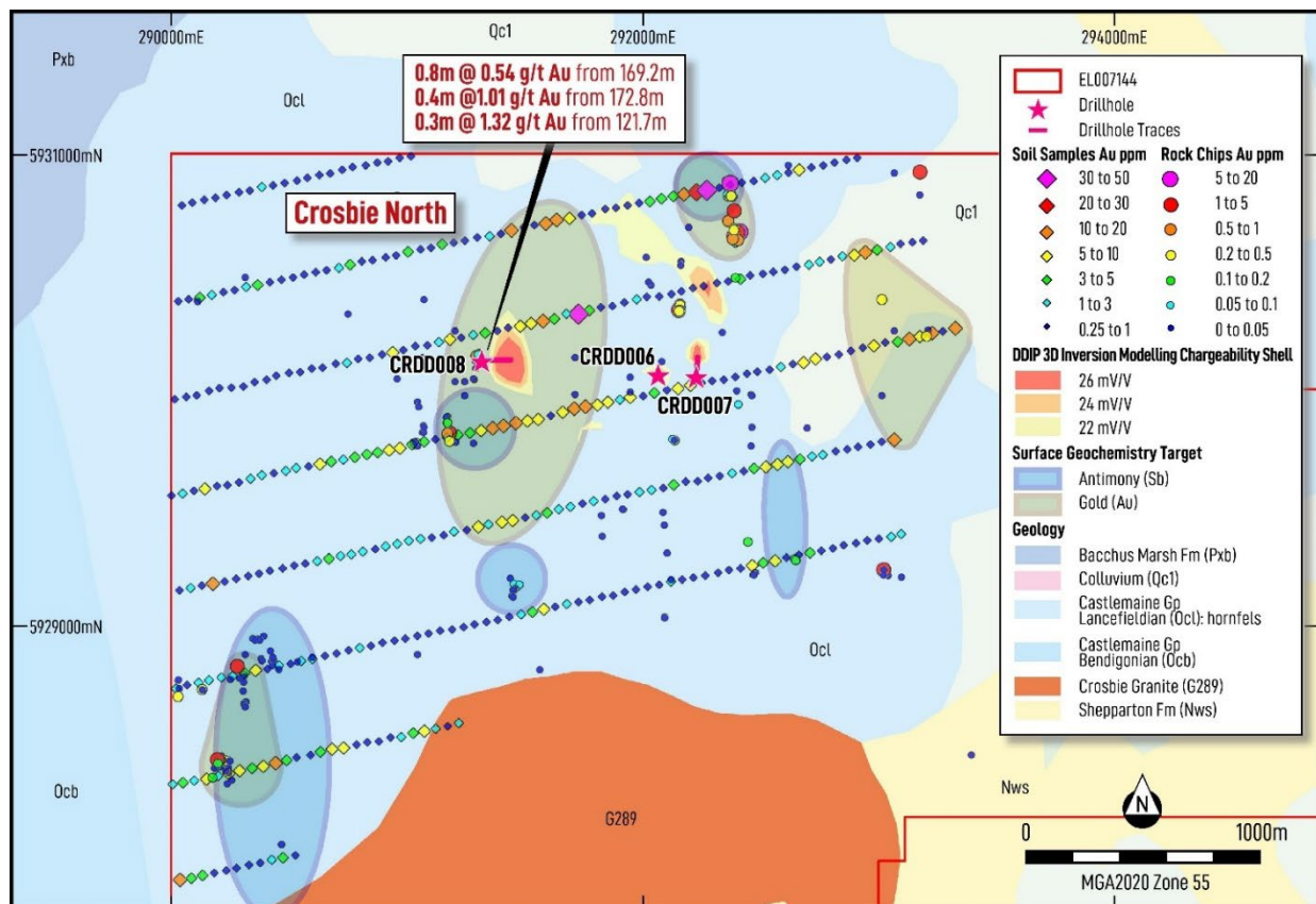
Figure 3: Crosbie North Geology, Surface sampling, Geophysics and Drilling.
