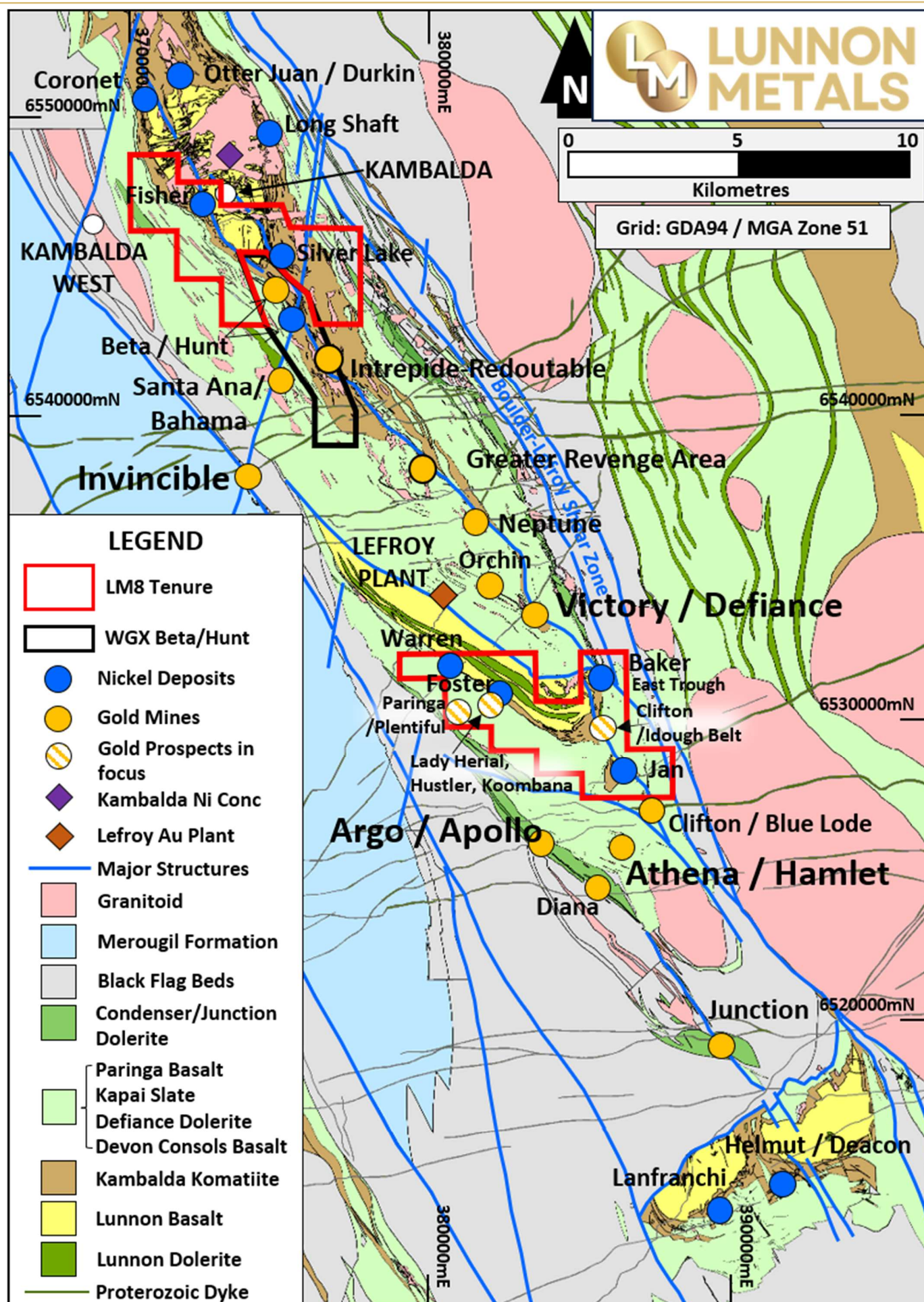
Figure 6: Location of the KGNP (red outlines) at the local Kambalda Nickel District / St Ives Gold Camp scale; showing surface geology and structure of this significant Australian gold camp.
