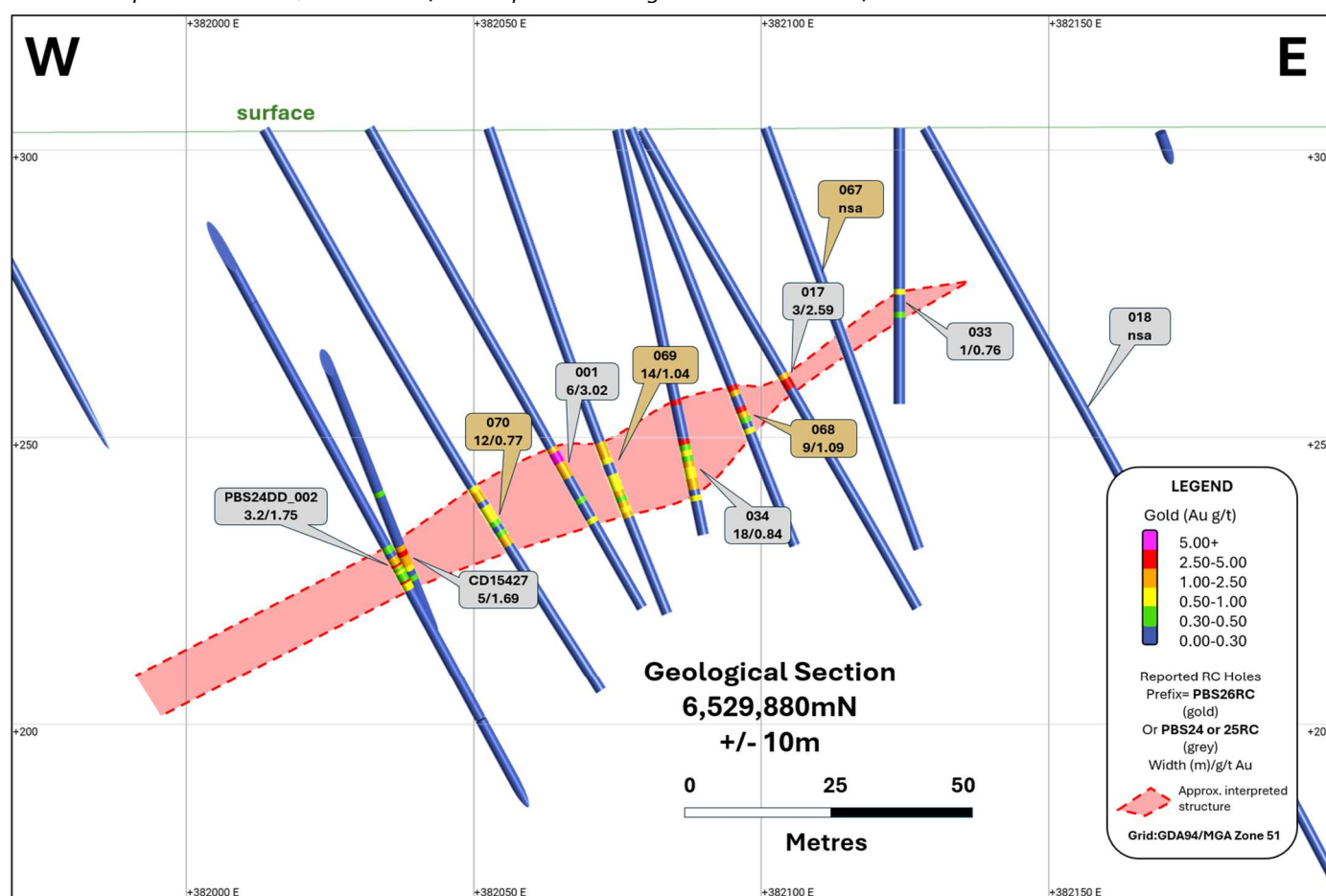
Figure 2: Typical Plentiful cross section at 6,529,880mN showing current and previous 3 results (further cross sections are included later in the report).
