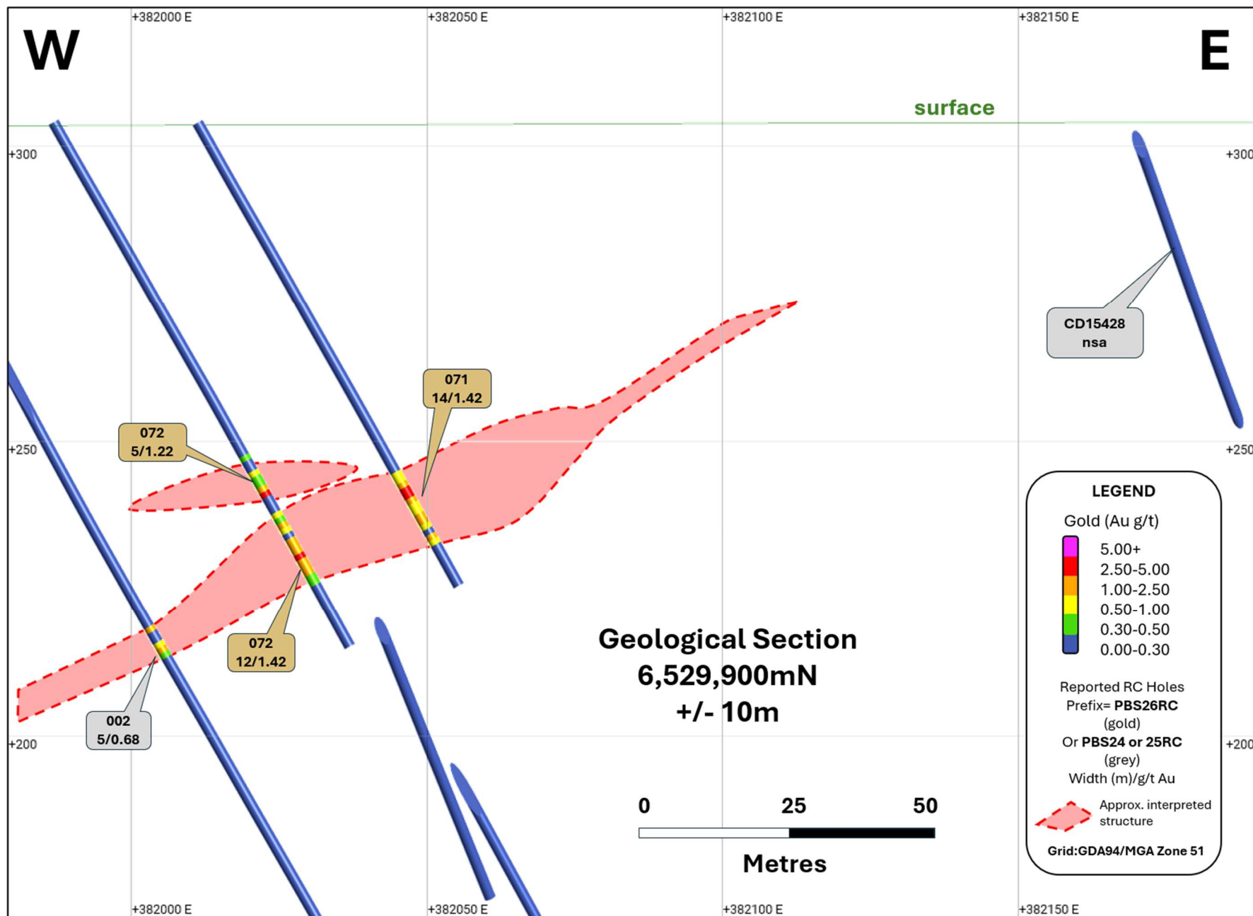
Figure 5: Cross section 6,529,900mN through today's and previous Plentiful RC results.
