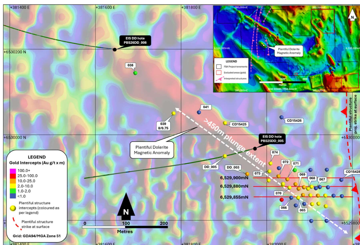
Figure 1: Plan view showing recent RC results (drill hole IDs 065 to 074), location of the cross sections reported and the now completed EIS deep drilling program, all against a geophysical magnetics background.
