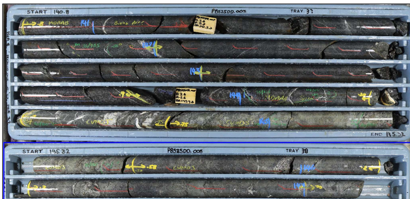
Figure 3: Altered shear complex of dolerite and quartz + carbonate veining with 1.9m @ 1.18 g/t Au at 142m in PBS25DD_005.
