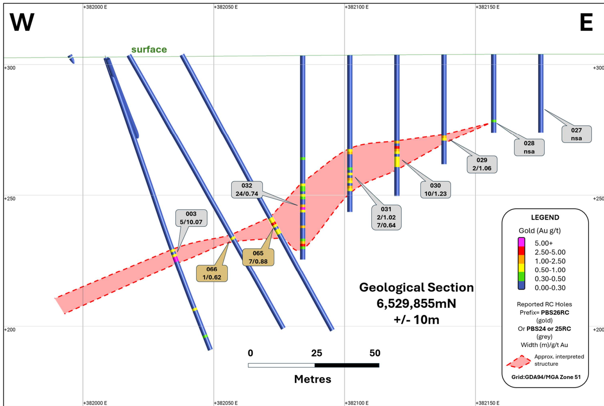
Figure 4: Cross section 6,529,855mN through today's and previous Plentiful RC results.
