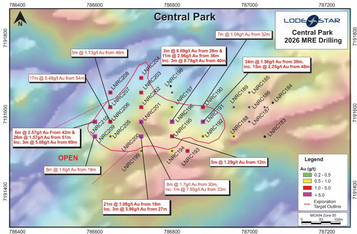
Figure 3: Plan view of Central Park 2026 drilling.
