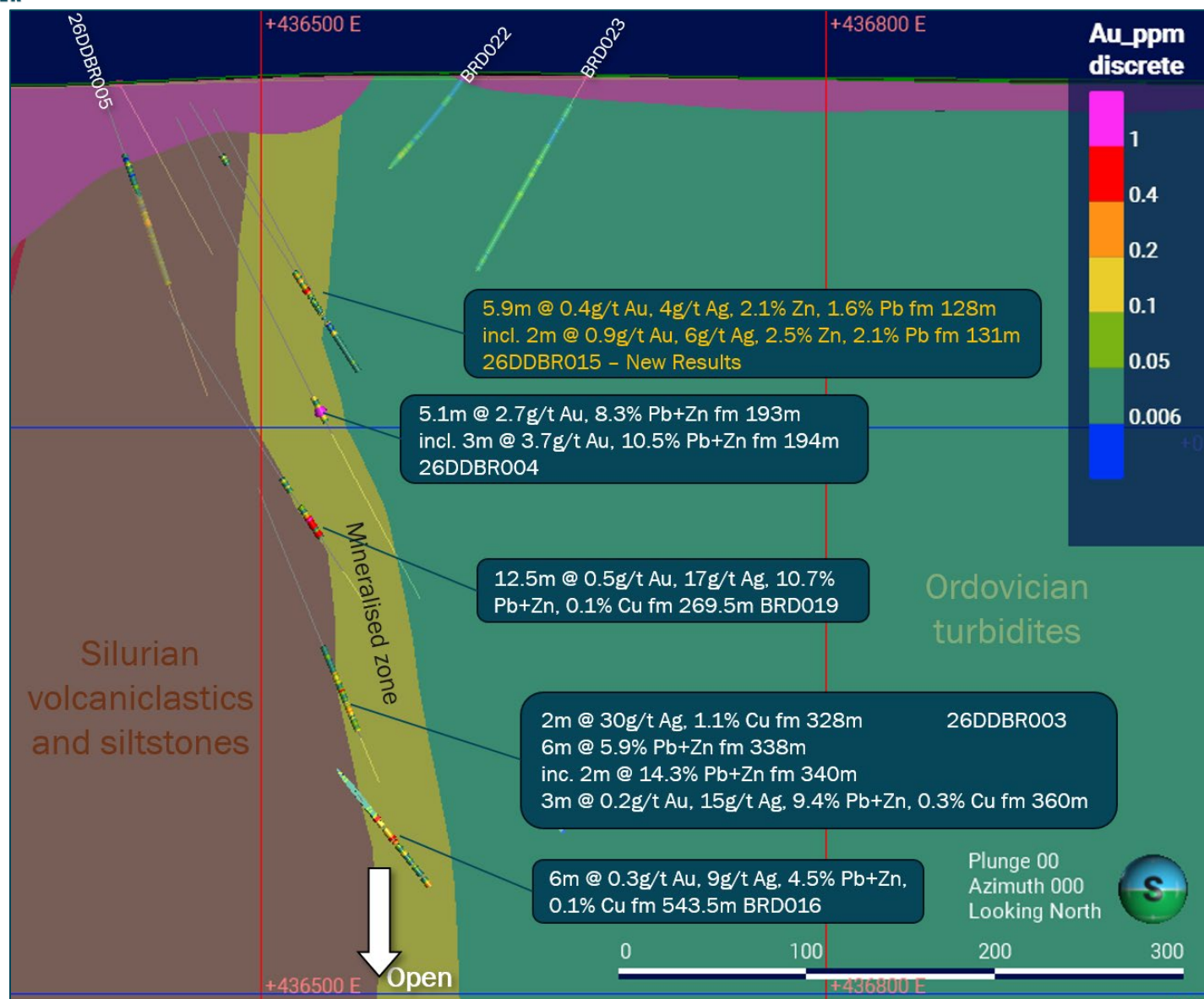
Figure 2: Cross section through 26DDBR015. (50m section).
