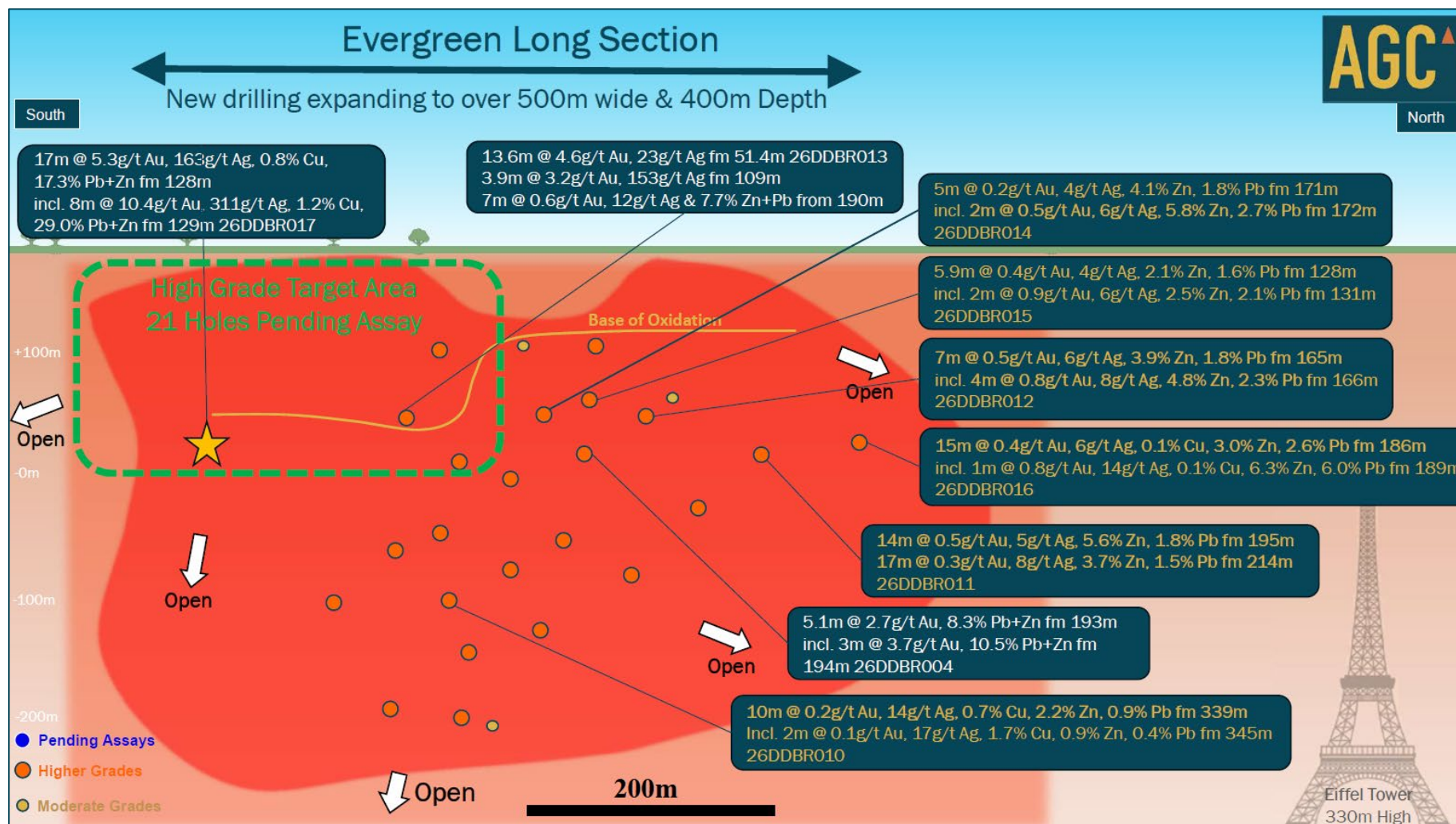
Figure 1: Evergreen long section showing significant drill intercepts, with new results in orange text.
