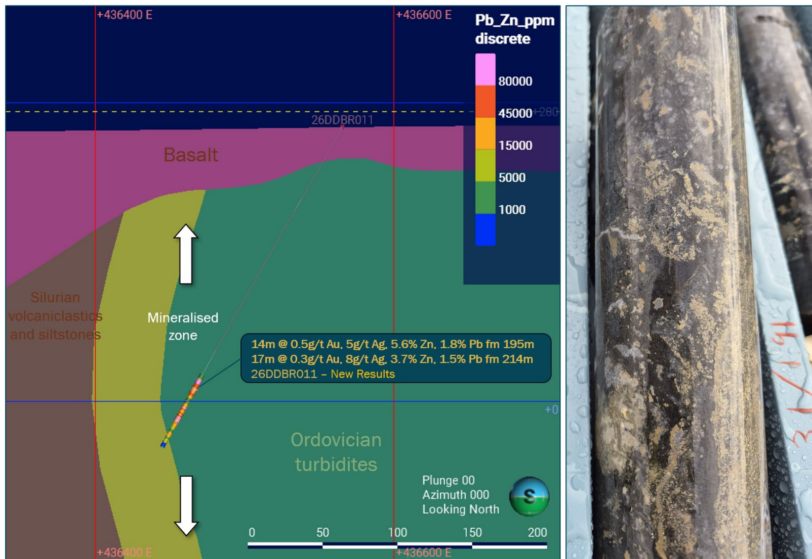
Figure 3: Cross section through the broad mineralised section in 26DDBR011. (50m section). 26DDBR011 high-grade drill core, sphalerite and pyrite (brown) replacing shell fossils
