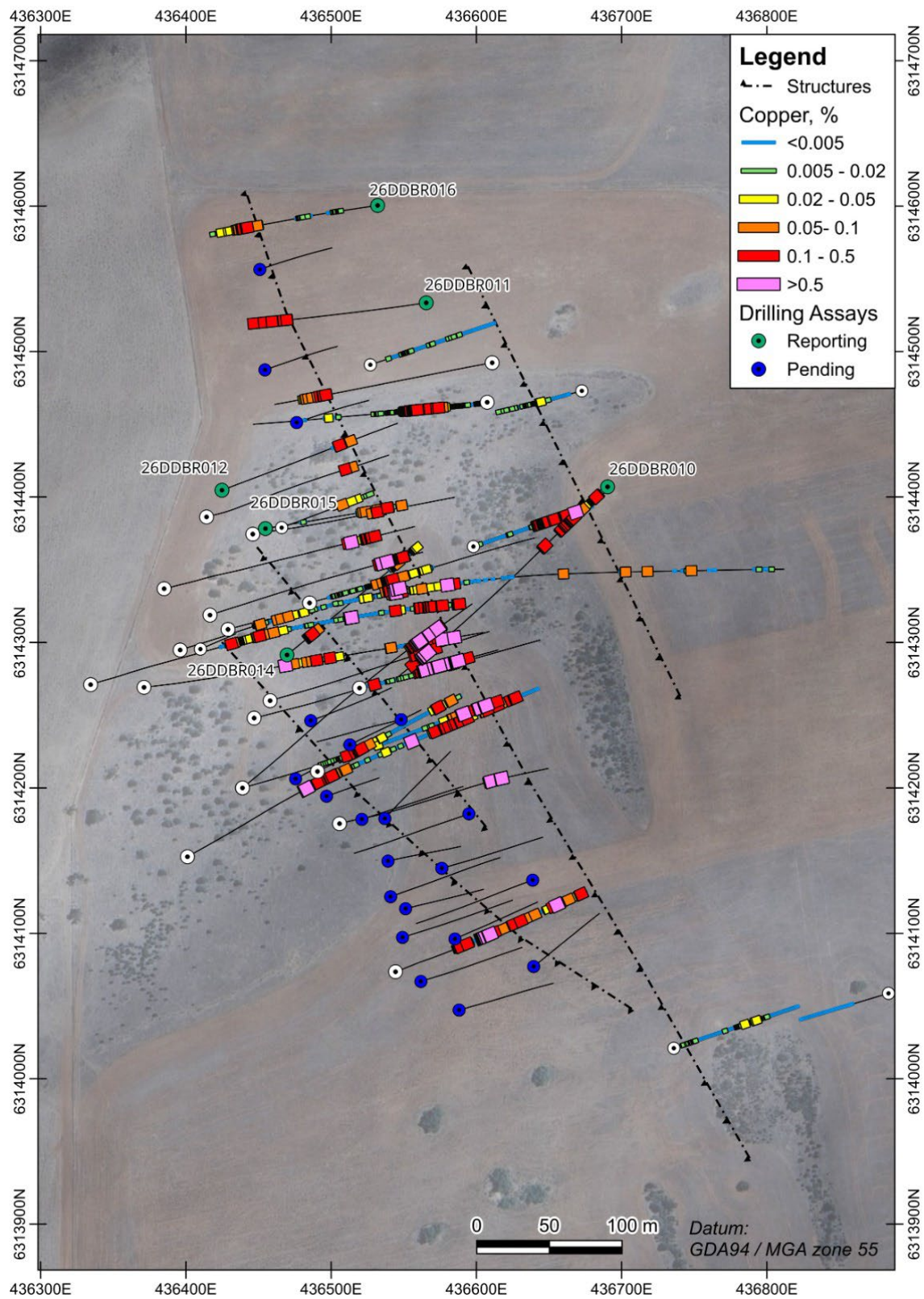
Figure 5: Plan map showing copper results at Evergreen with holes being reported with green collars, holes pending assays with blue collars.
