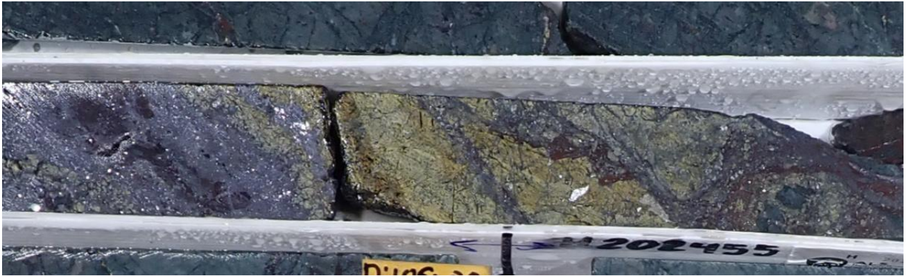
Figure 4. Cut core from GV-26-008 from ~107.3 to 104.7m down hole, showing massive galena (grey), low-iron sphalerite (pale yellow) and hematite (red-brown) mineralisation. This interval returned 1.0m at 76g/t Ag, 17.0% Zn & 14.6% Pb from 107m.
