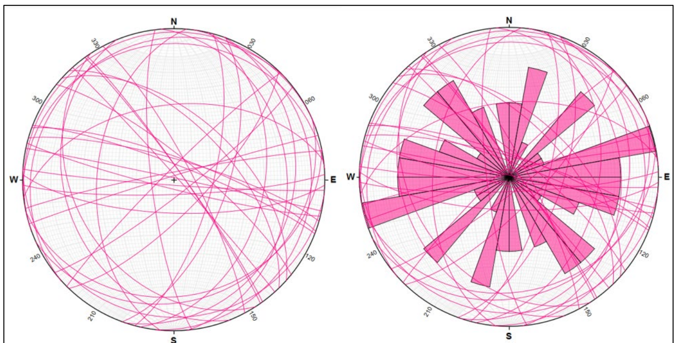
Figure 10: Stereonet (left) and rose diagram (right) of mapped felsic intrusions at Blue Lagoon.
