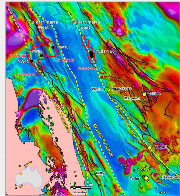
Pulkarrimarra: Paterson Province regional magnetic image with deposits
