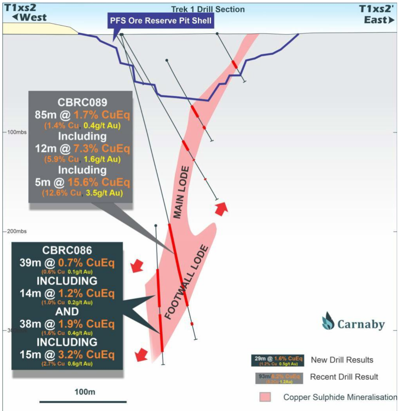
Figure 28: Trek 1 Cross Section showing recent Footwall Lode drill results
