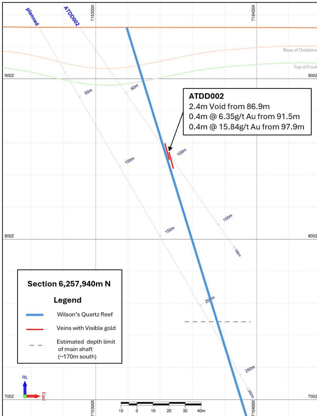
Figure 2. Cross Section 6,257,940mN showing ATDD002.
