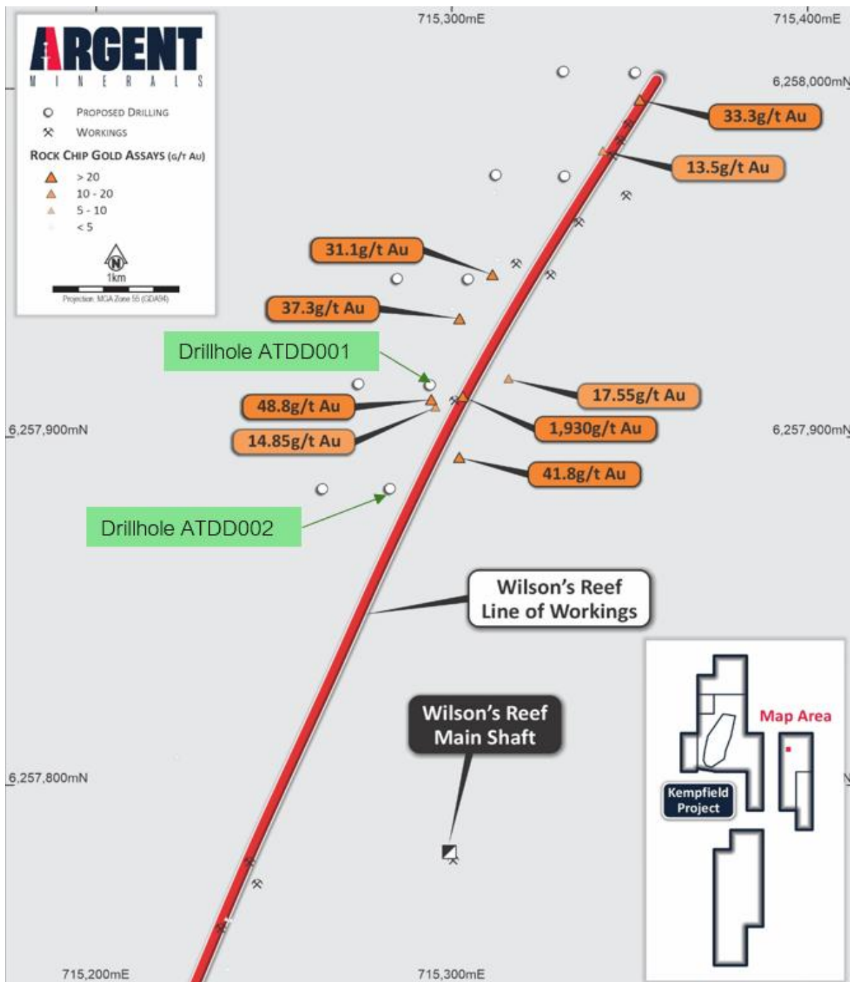
Figure 1. Plan of the Trunkey Creek mineralised corridor showing Phase 1 collar locations, completed drillholes ATDD001 and ATDD002, and the known historic workings.
