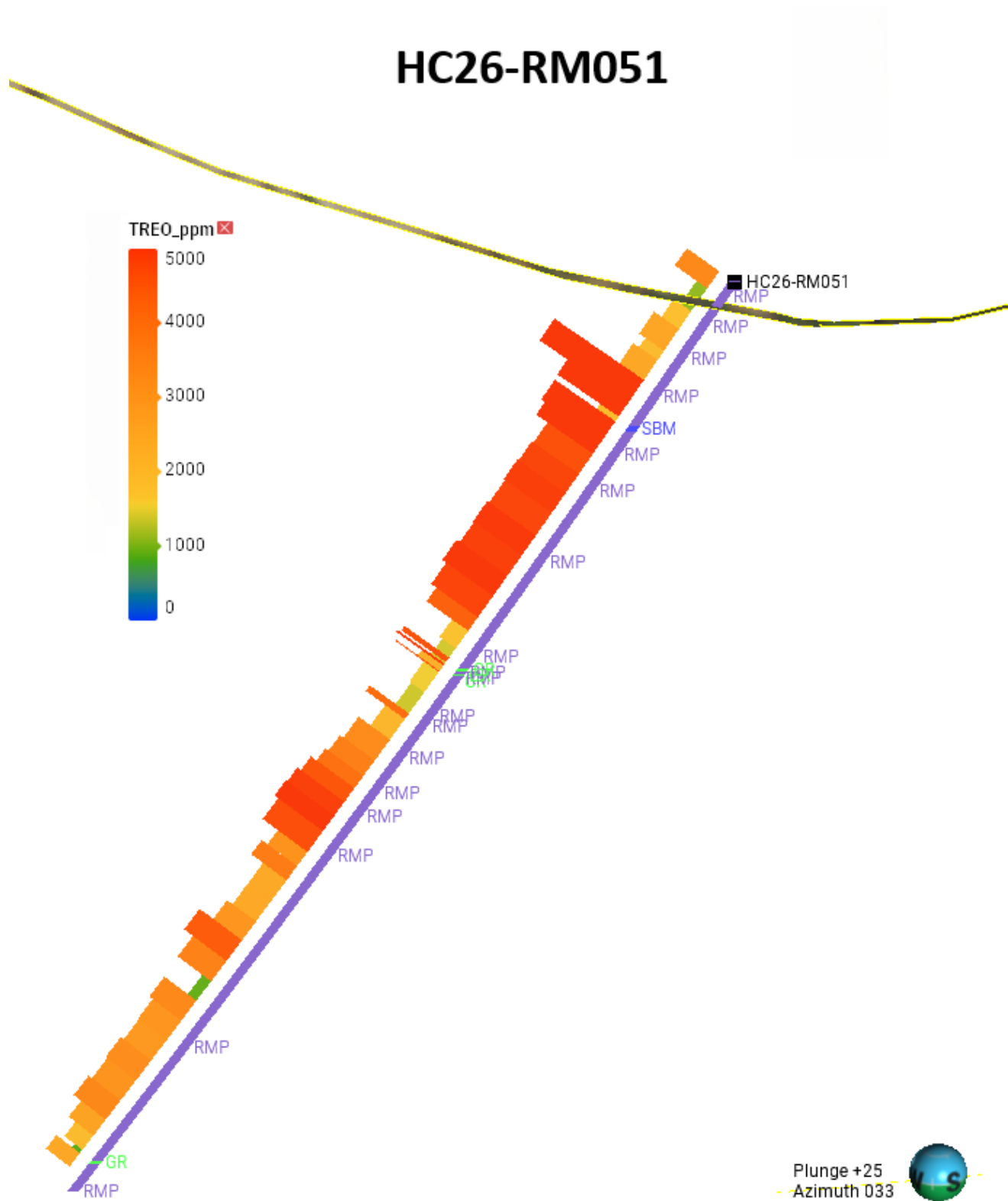
Figure 3 HC26-RM051 Cross Section Showing Down-Hole TREO Distribution
