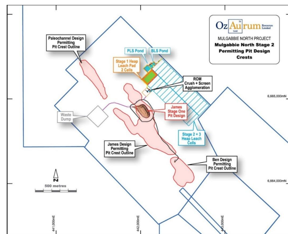
Figure 1: Stage 2 Design Permitting Pit Crest Outlines
