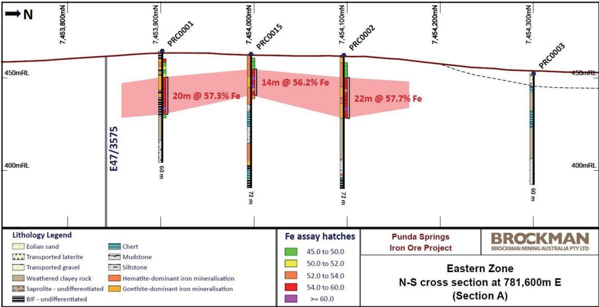
Figure 5 – Geology and drilling cross section 781600mE (Section A)
