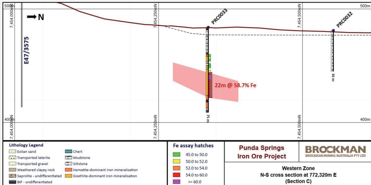
Figure 6 – Geology and drilling cross section 772320mE (Section C)
