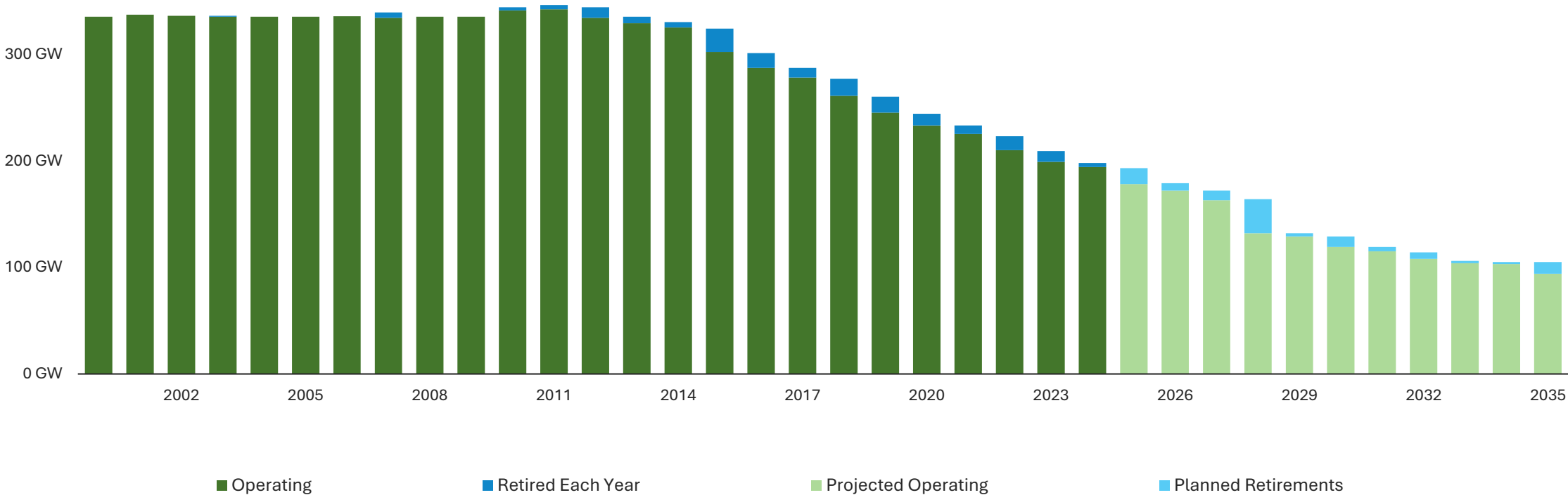
Coal-Fired Power Capacity in the U.S.
