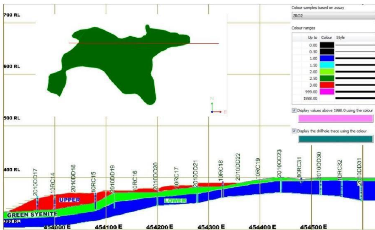
Figure 18: A typical cross section from Tanbreez Hill - with Upper (red) and Lower (blue) blocks and interstitial syenite (green).
