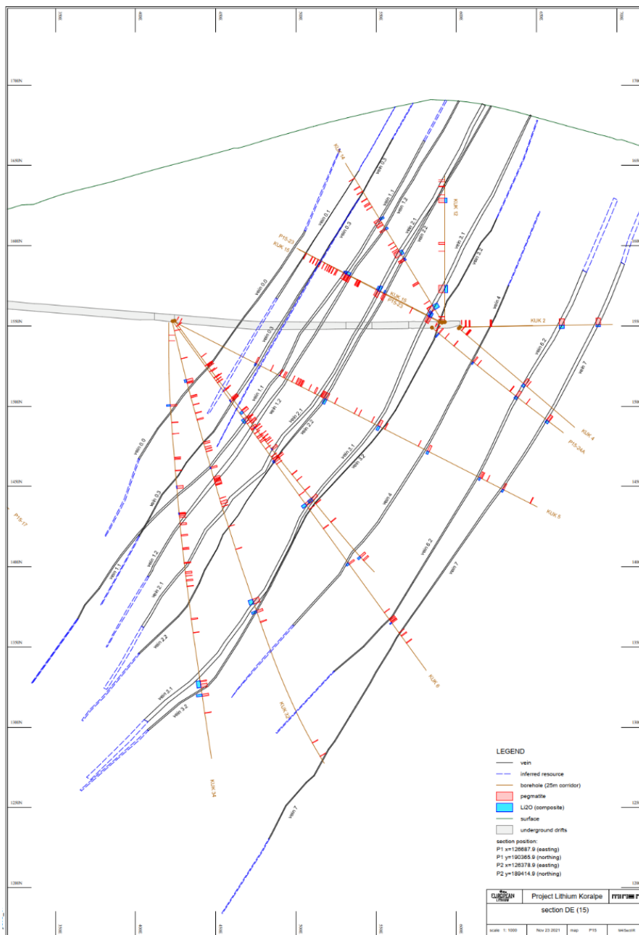
Figure 35: Cross section showing underground drillholes and the interpreted pegmatite model with Inferred mineral resource extensions in blue
