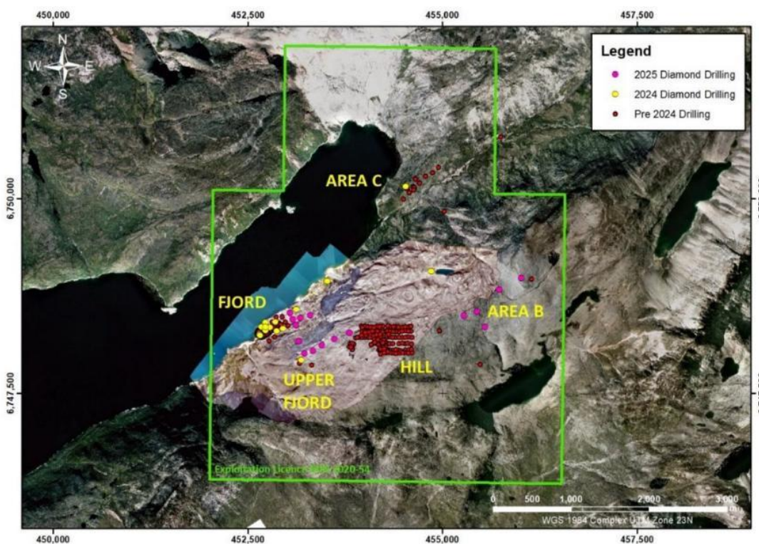
Figure 10: Project Drilling showing historical drilling and CRML's 2024 and 2025 drillhole locations
