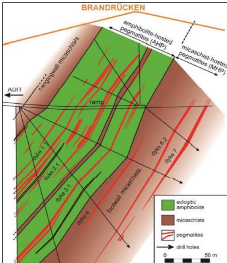
Figure 31: Typical Cross Section Showing AH and MH Pegmatites
