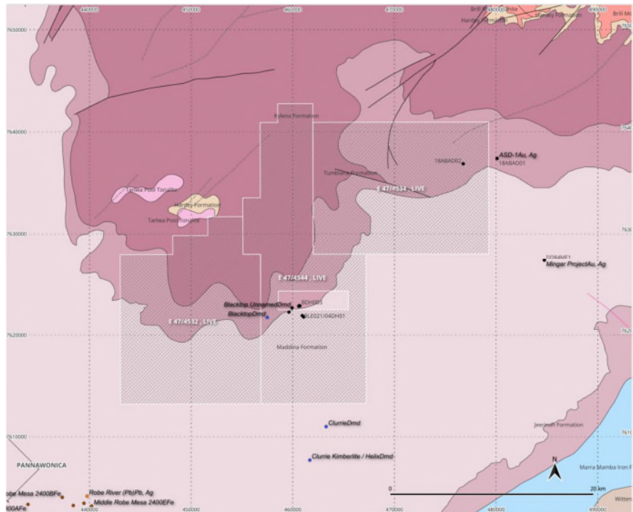
Geology of Munni Munni South tenure. Source: VRM compiled data sourced from DMPE.
