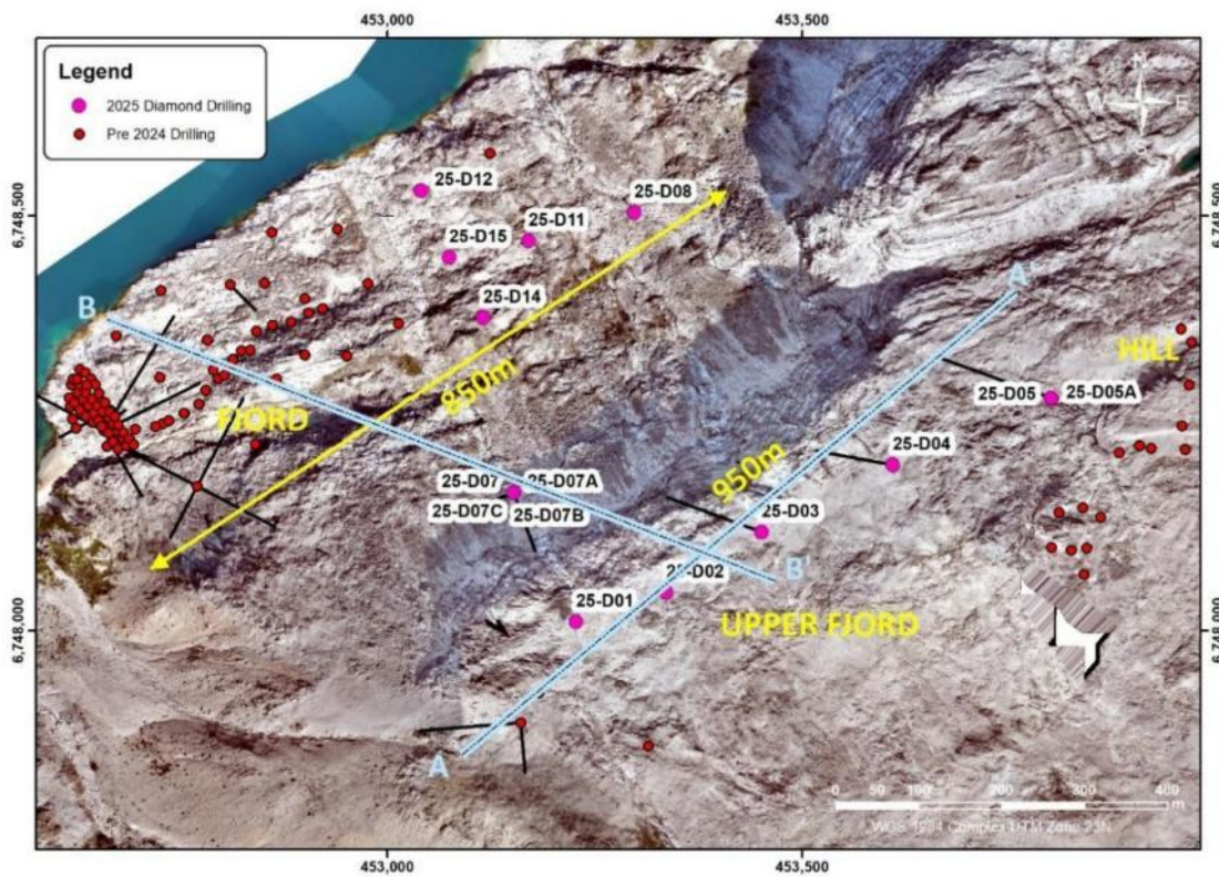
Figure 11: Drillhole locations at Fjord deposit showing most recent 2025 drillhole locations in pink Source: EUR ASX Announcement, 10 February 2026
