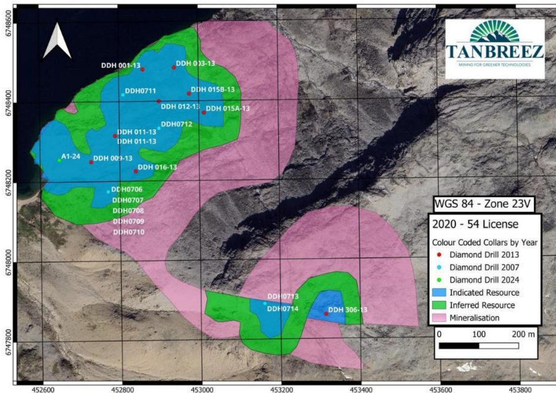
Figure 16: Location of selected drill holes in relation to the Indicated and Inferred MRE outlines interpreted by VRM to be the Fjord deposit and interpreted mineralised kakortokite (pink)
