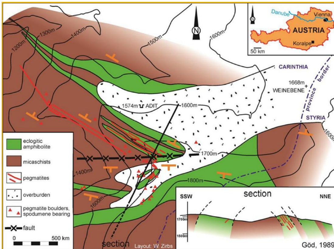
Figure 29: Geology of Wolfsberg Project (after Göd, 1989).
