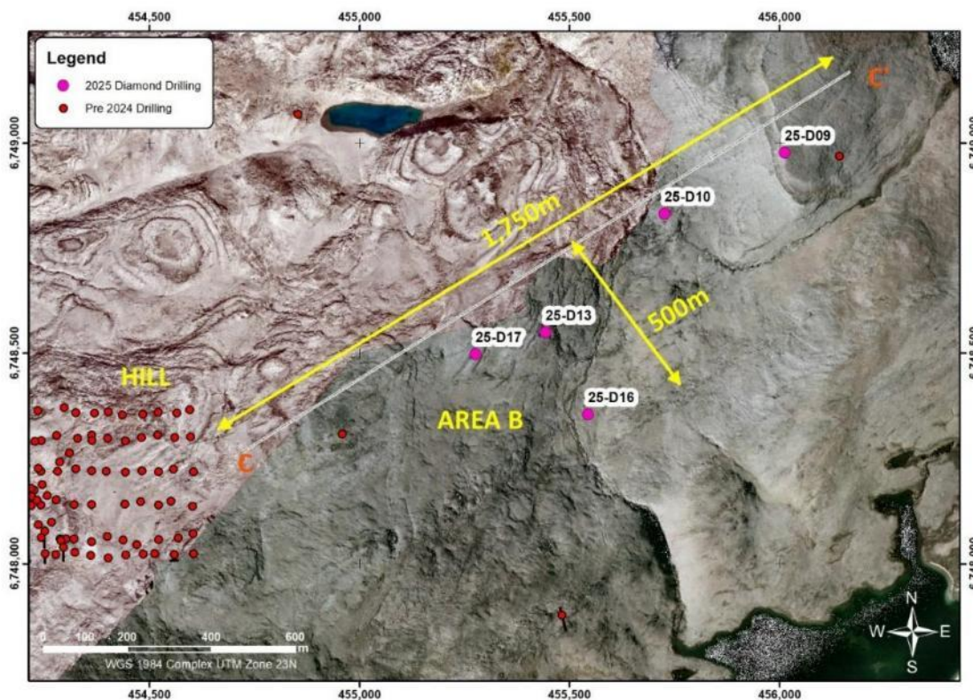
Figure 14: Drillhole locations at Area B prospect showing 2025 drillhole locations in pink
