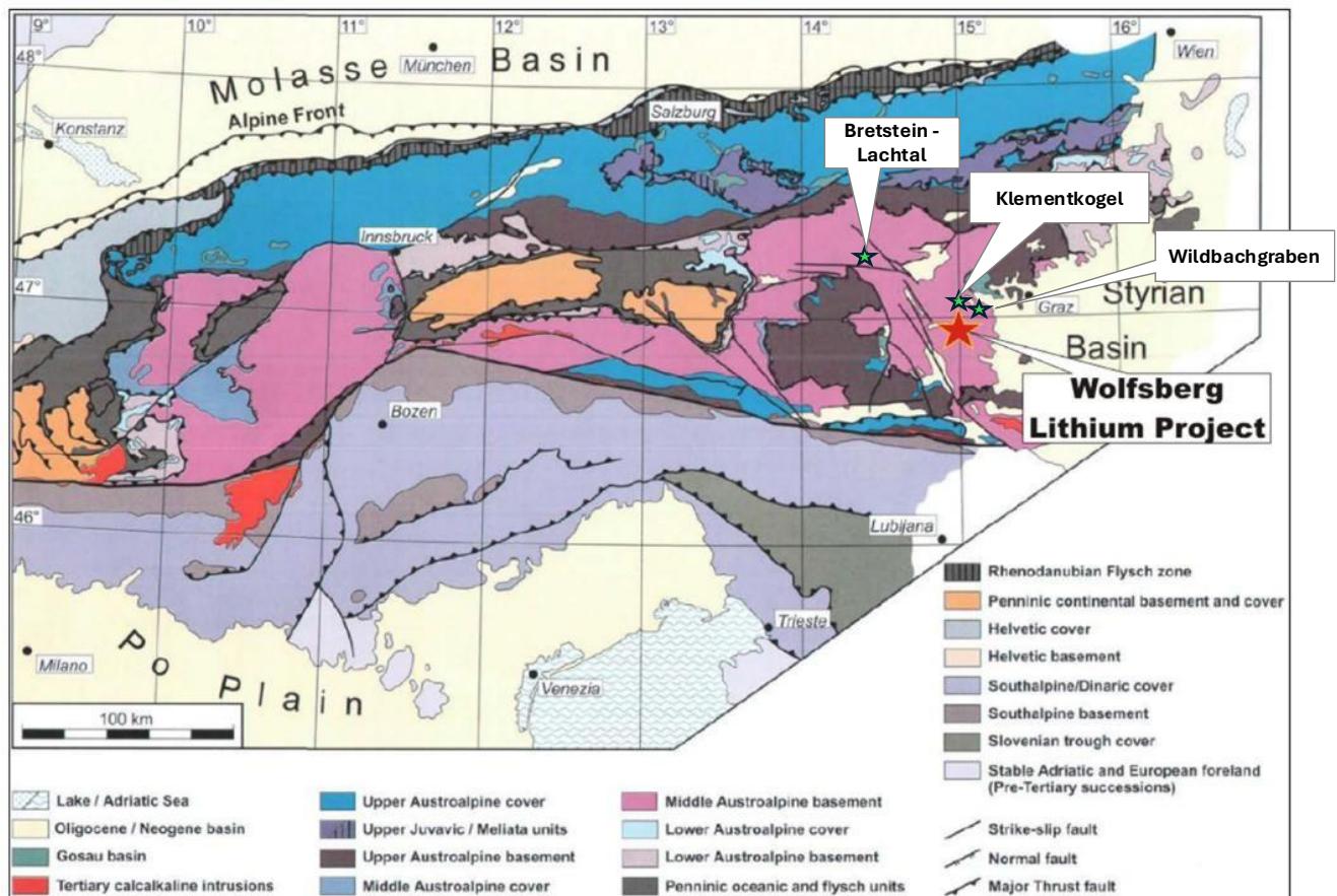
Figure 26: Geological map of the Austrian Region (from Neubauer and Hock, 1999). Project locations are approximate.
