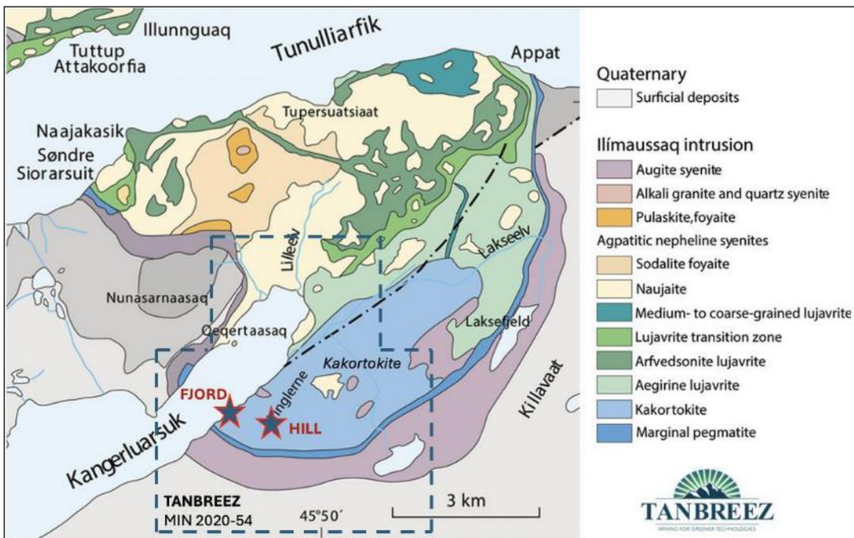
Figure 7: Regional Geology showing the location of Tanbreez Fjord and the Tanbreez Hill prospects
