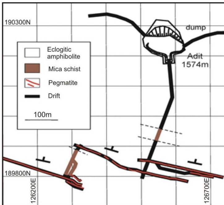
Figure 33: Wolfsberg plan view of underground workings
