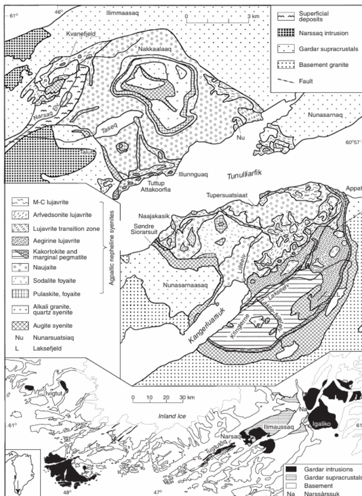
Figure 6: Regional geology showing the Ilímaussaq complex and Gardar intrusions. Tanbreez REE deposit is at Kringlerne.
