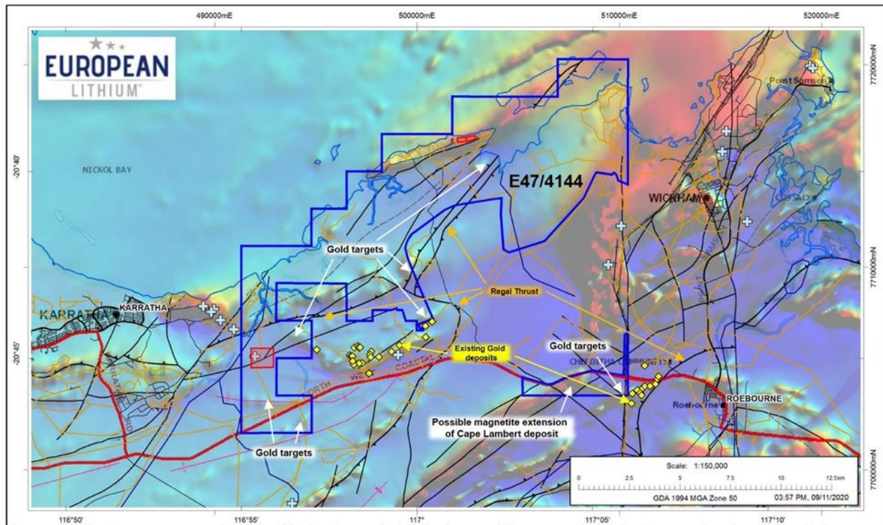
Figure 51: Regional magnetic imaging in the area of E47/4144
