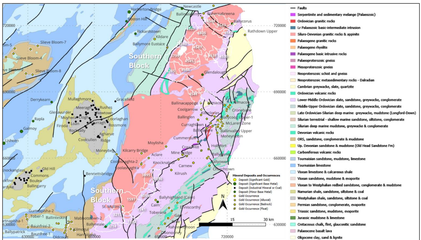
Figure 45: Regional geology of Leinster project, showing project tenure in white
