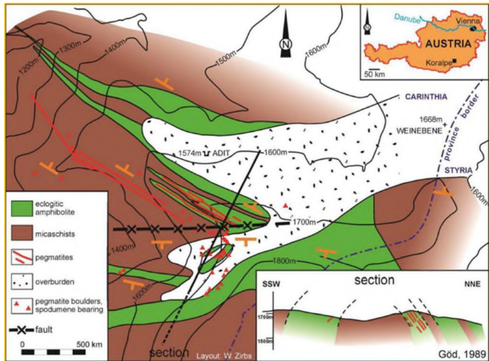
Figure 8: Geology of Wolfsberg Lithium Project (after God, 1989) (Source: EUR ASX Announcement, Prospectus 21 June 2016)
