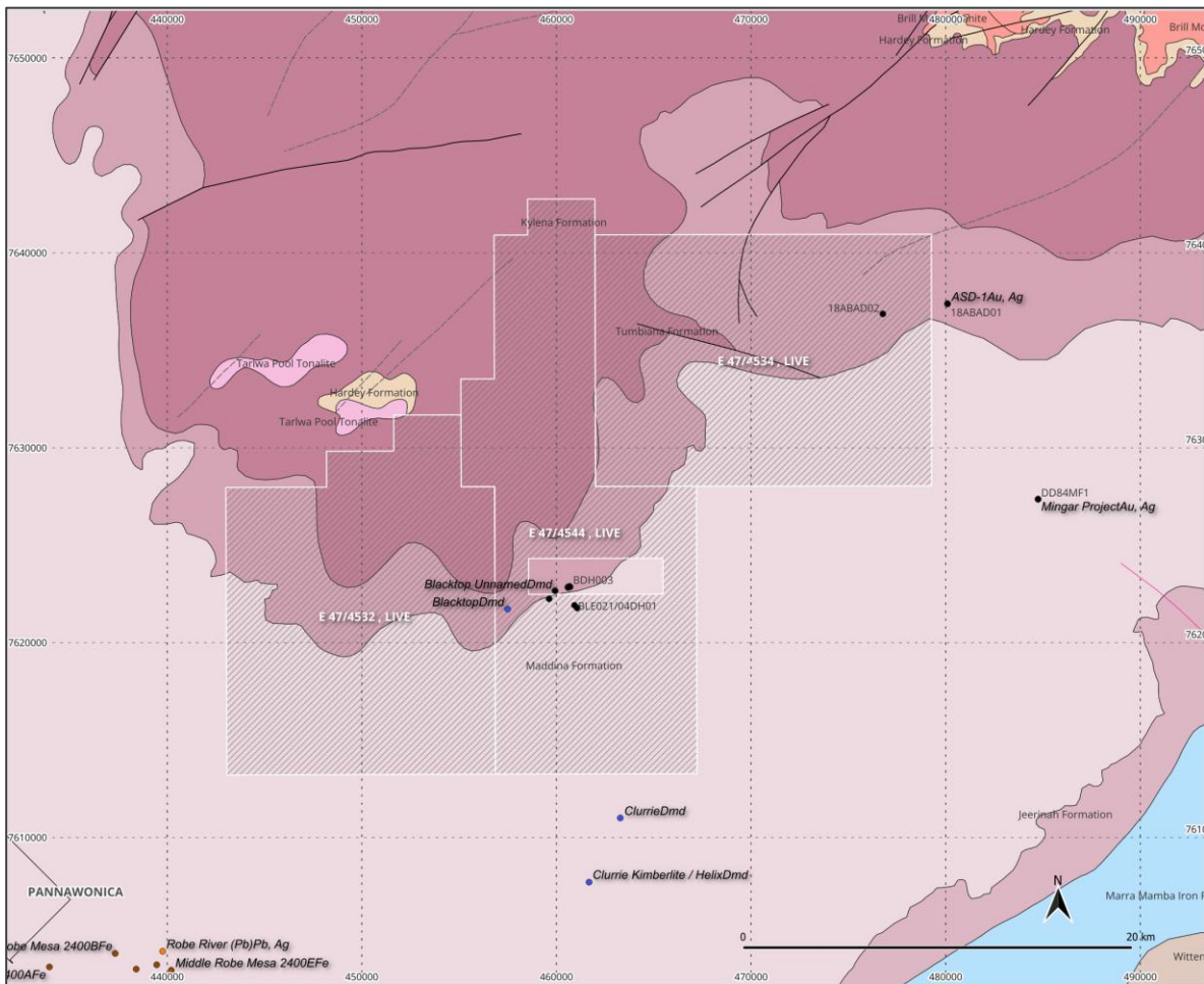
Figure 49: Geology of Munni Munni South tenure
