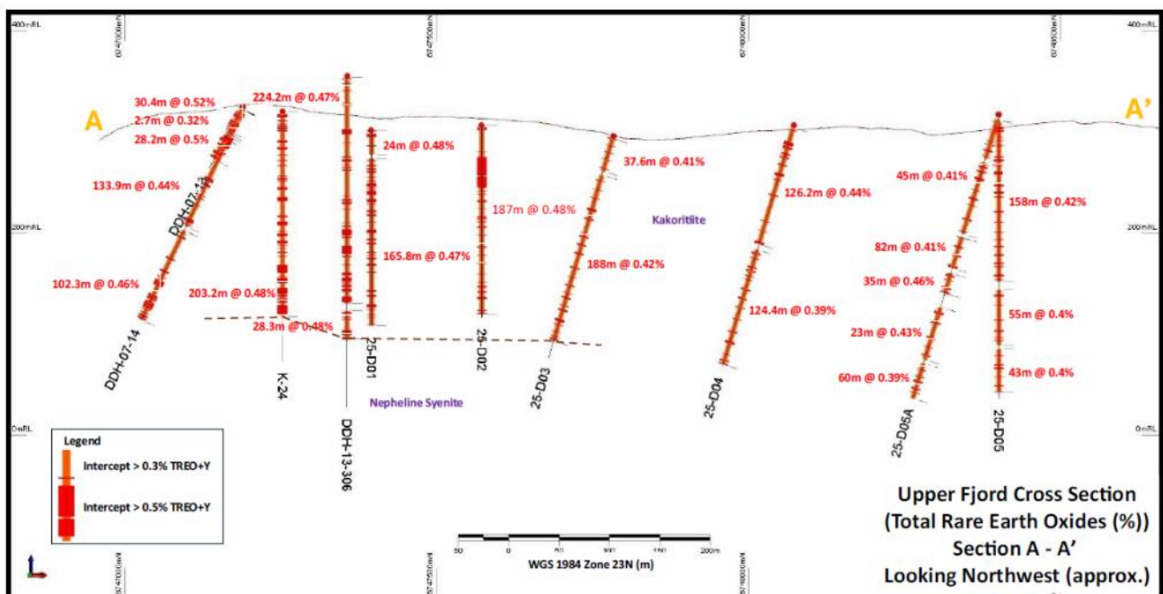
Figure 12: Upper Fjord Cross Section (refer Figure 11 for location) Source: EUR ASX Announcement, 15 January 2026
