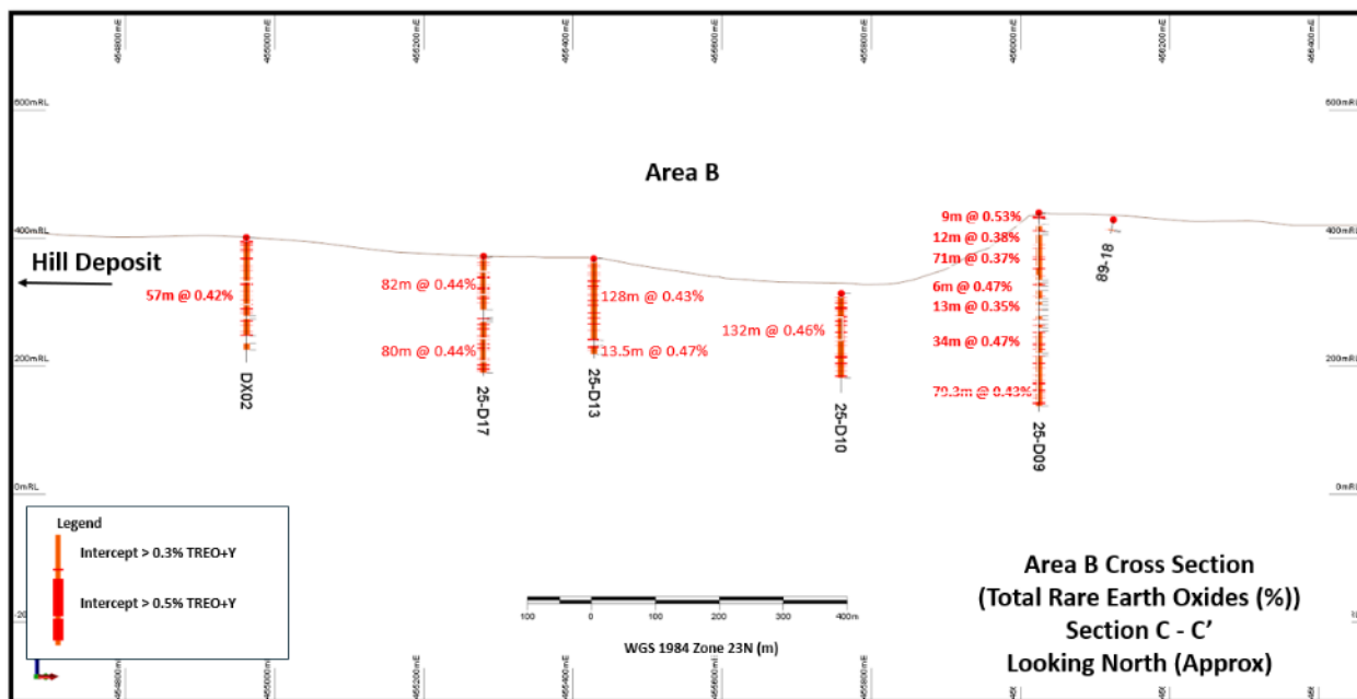
Figure 15: Cross section at Area B prospect (refer Figure 14 for location)
