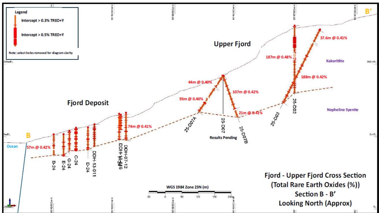
Figure 13: Fjord to Upper Fjord Section showing TREO mineralisation (refer Figure 11 for location)
