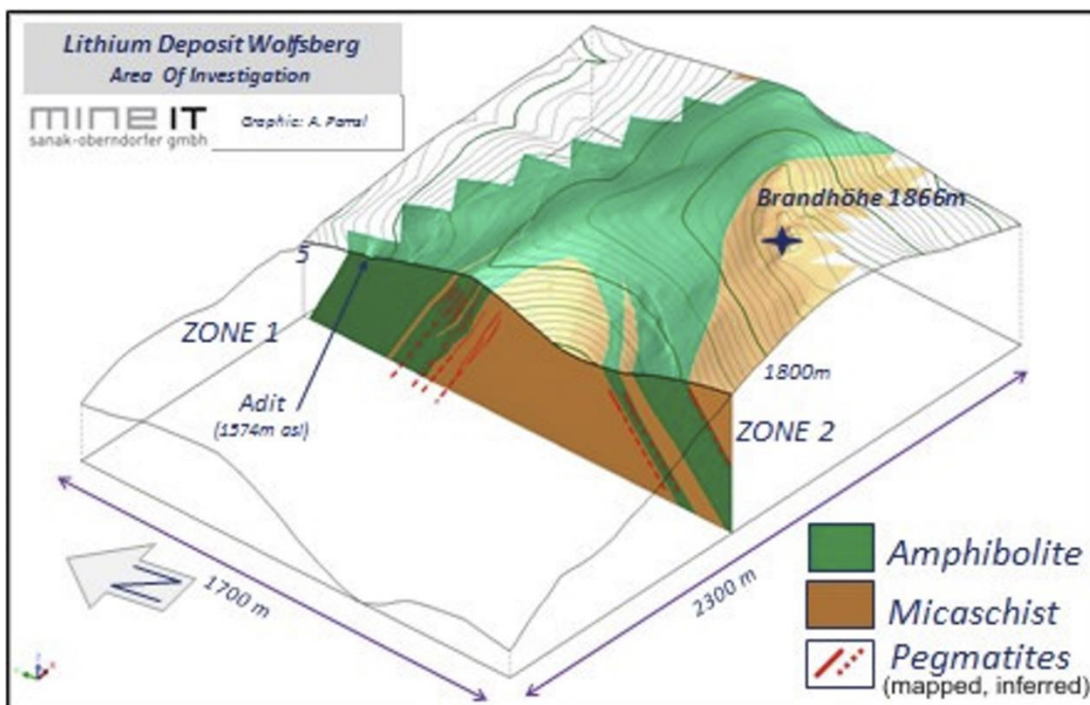
Figure 30: Three-dimensional schematic of Wolfsberg project
