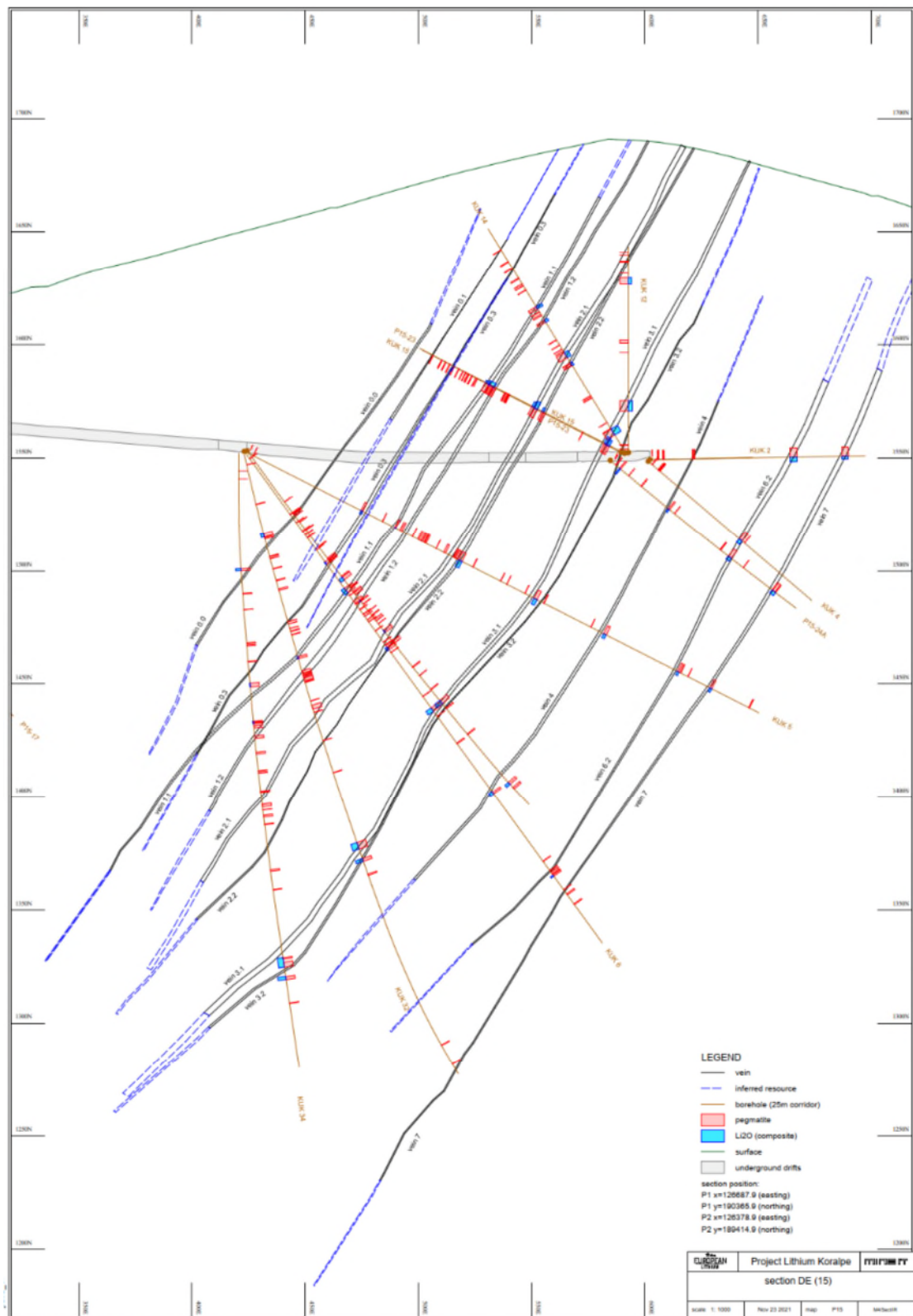
Figure 9: Cross section showing underground drillholes and the interpreted pegmatite model with Inferred mineral resource extensions in blue (Source: EUR ASX Announcement, 1 December 2021)
