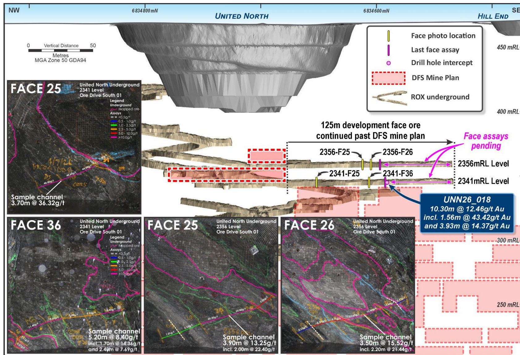
Figure 4 – United North 2356mRL & 2341mRL ore drive development vs. DFS Mine Plan
