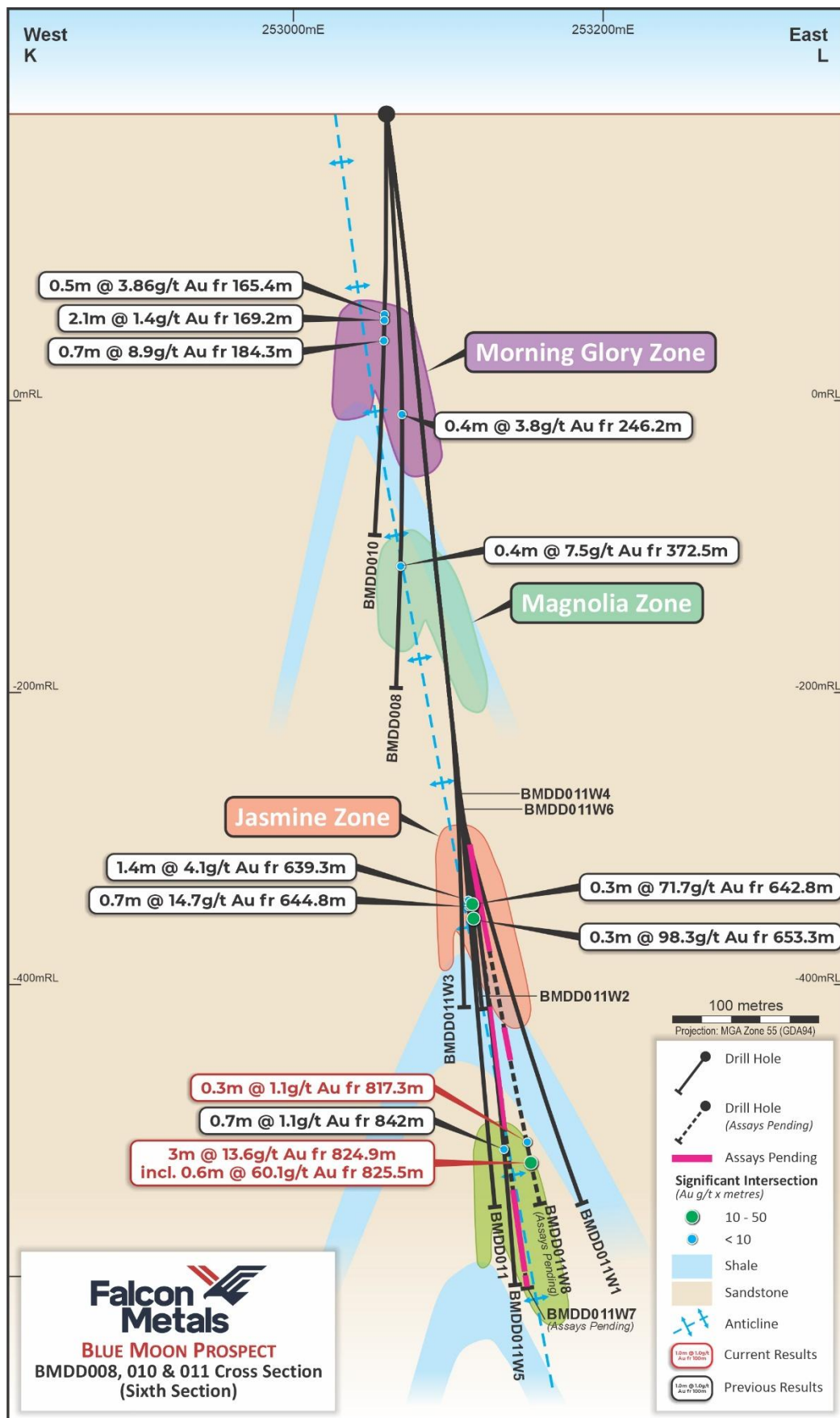
Figure 8 BMDD008, 010 & 011 section - Schematic cross section looking north with wedge BMDD011W05 still in progress
