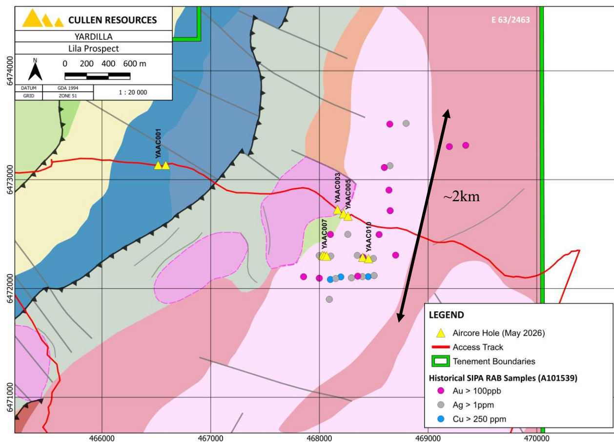
Fig. 7. Lila target area defined by combined Au-Cu-Ag anomalies in historical RAB (see following x-sections and plots).
