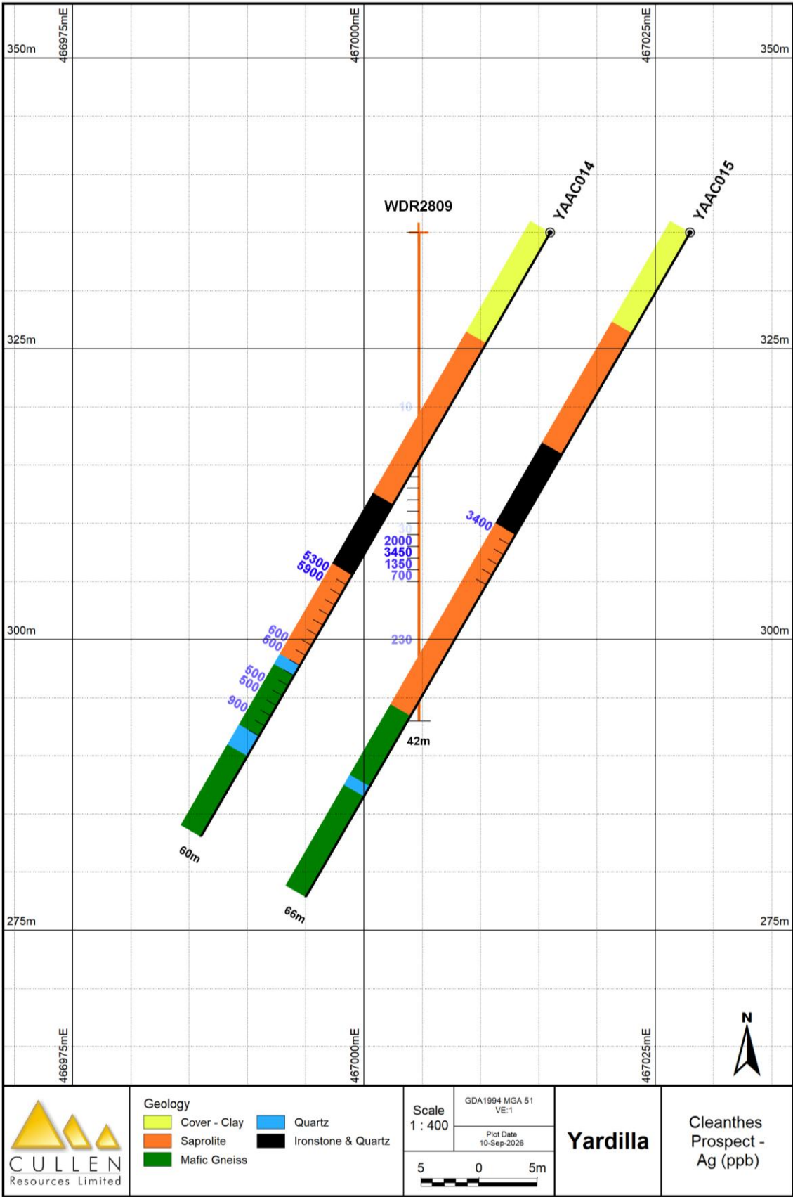
Fig 4. Anomalous drill intersections, Cleanthes prospect, Ag.
