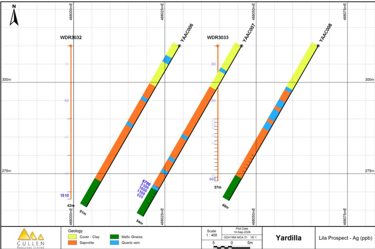
Fig. 9. Lila x sections for Ag (note holes YAC6 and 8 not resampled for Ag and Cu)
