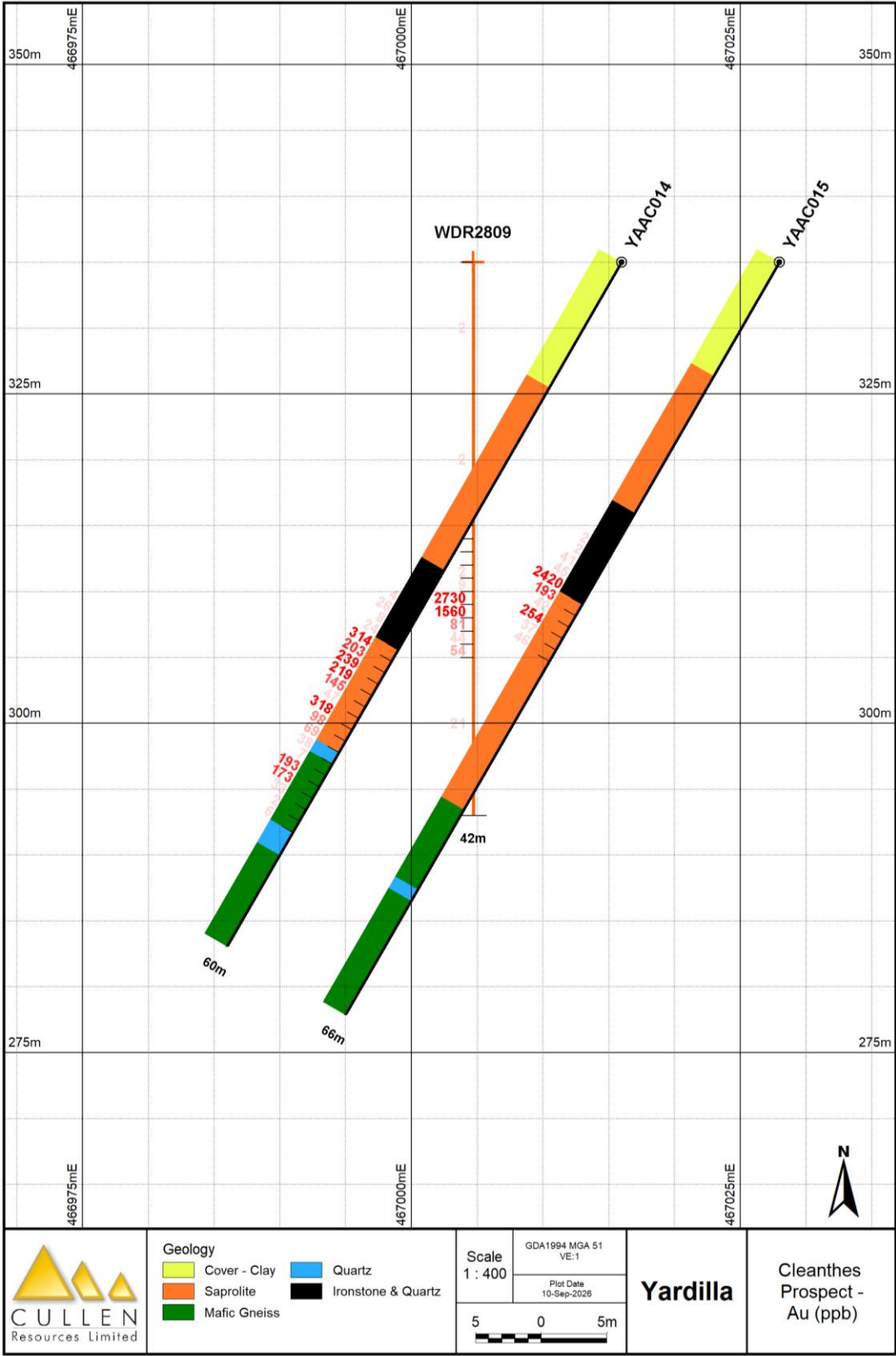
Fig 3. Anomalous drill intersections, Cleanthes prospect, Au. (WDR series drillholes are historical)
