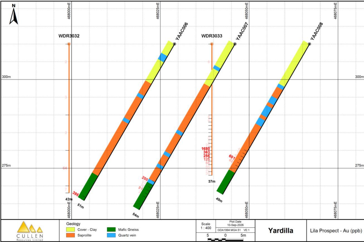
Fig. 8. Anomalous drill intersections, Lila prospect, Au
