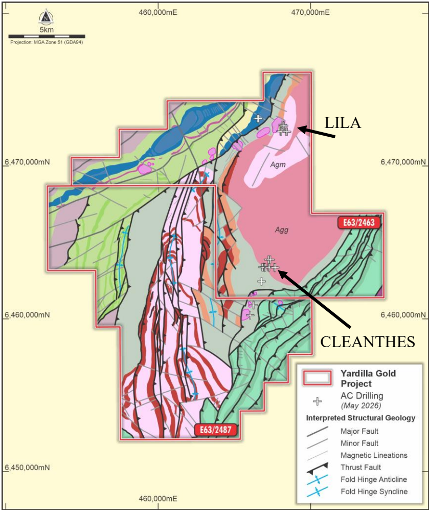
Fig. 2 Bedrock Interpretation Map with May air core drilling program locations
