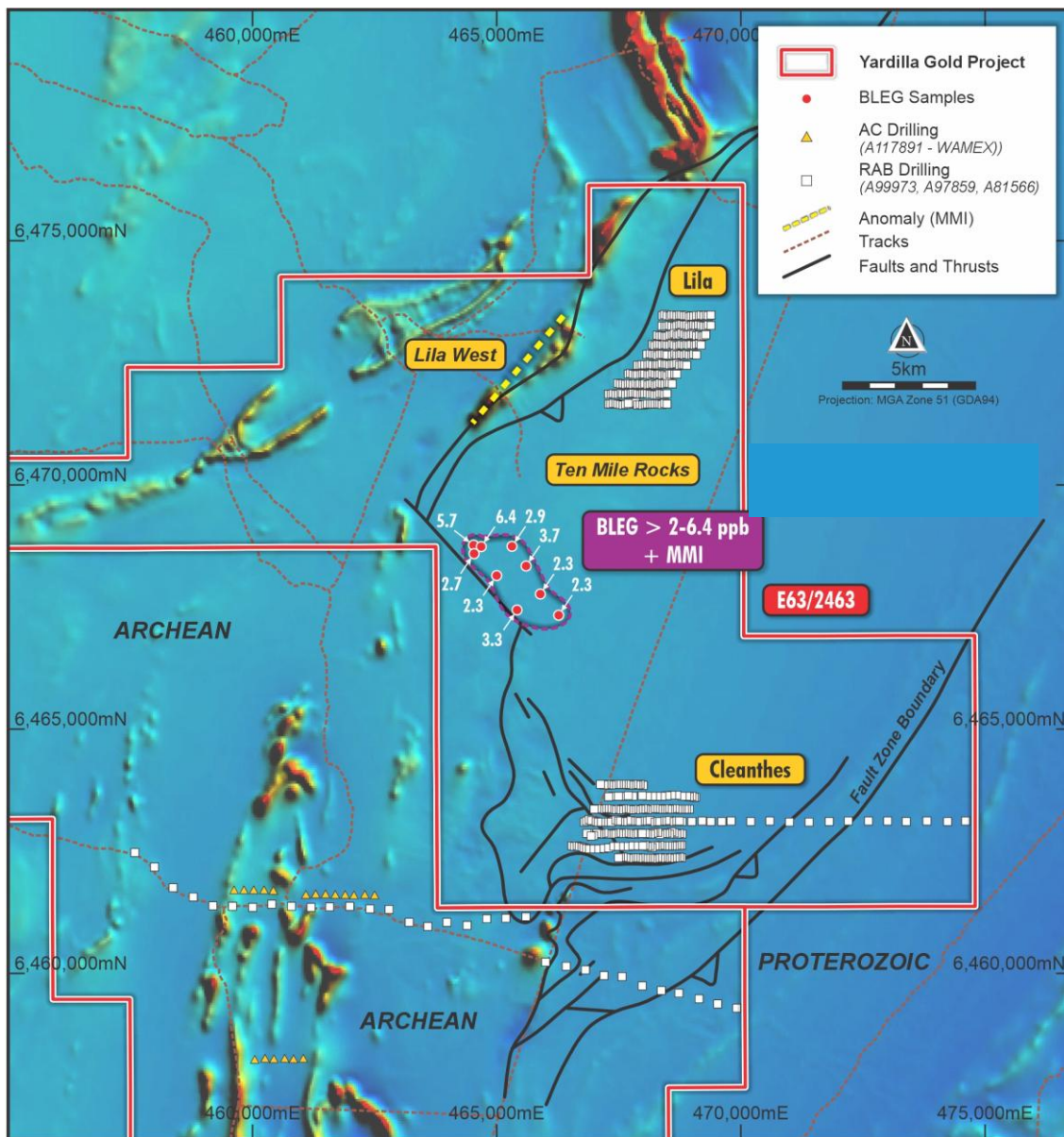
Fig. 11. Mag image underlines focus of soil anomalies along an interpreted fault/thrust system.
