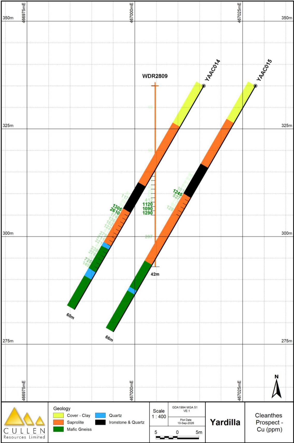
Fig 5. Anomalous drill intersections, Cleanthes prospect, Cu
