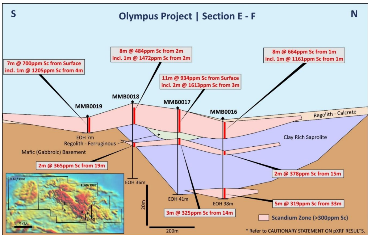
Figure 5: Olympus RAB Line E-F highlighting scandium intersections.
