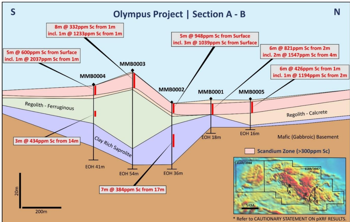
Figure 4: Olympus RAB Line A-B highlighting scandium intersections
