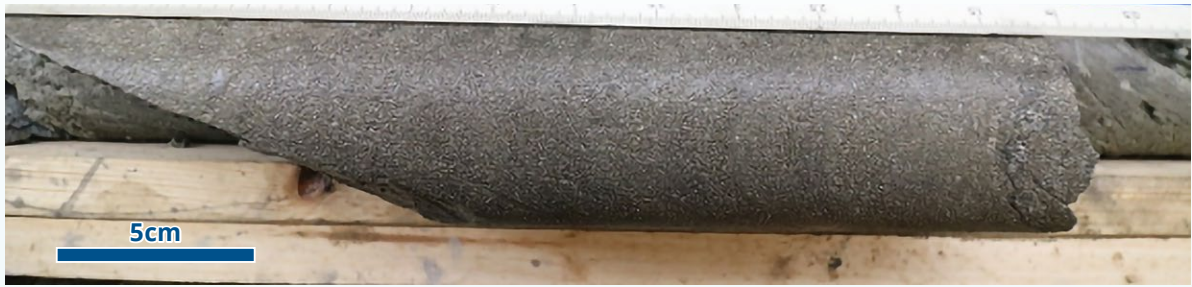
Figure 3: Example of massive sulfide from the Fuego Prospect (K26-571, 61.8-62.0m downhole). The interval from 61.0 to 62.0m returned assays of 126g/t Ag, 5.5% Zn, 0.9g/t Au, 0.1% Cu, 3.8% Pb.
