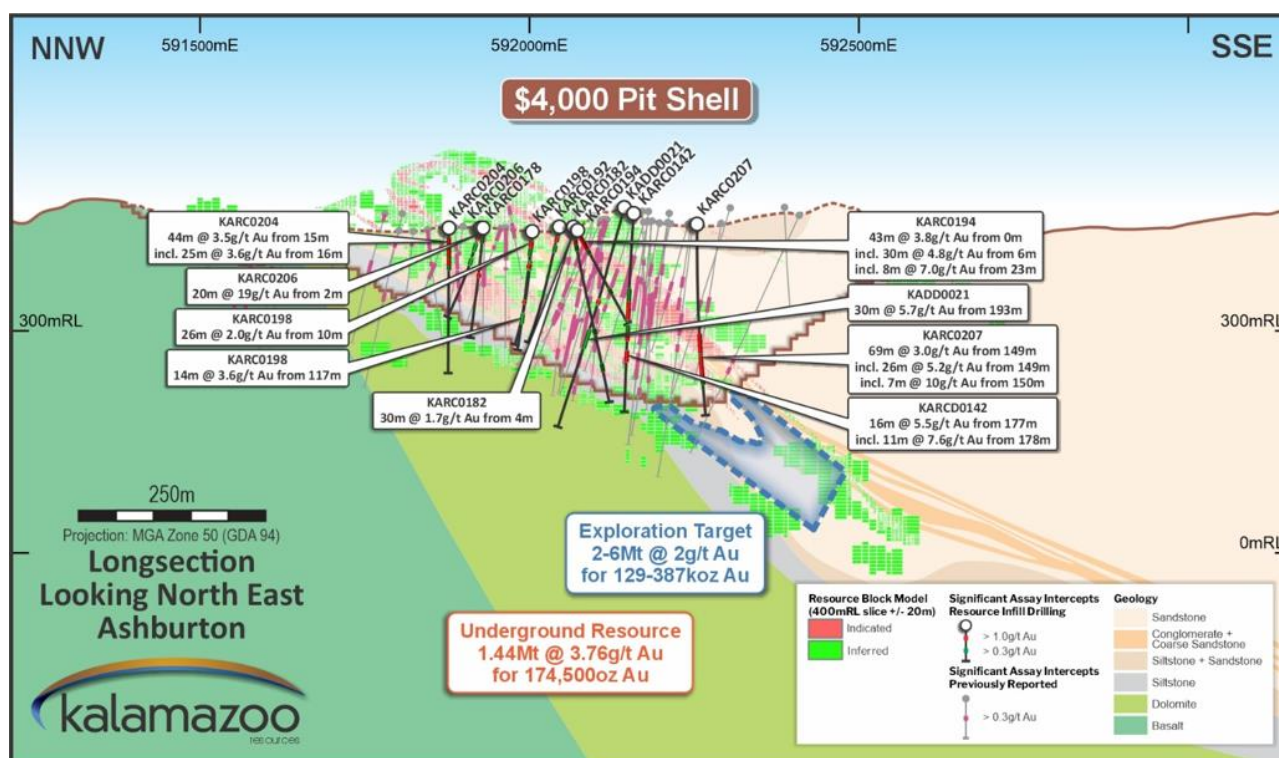
Figure 7: Mt Olympus long section showing drill traces and significant assay intercepts from recent Resource Infill drilling. Current Mineral Resource outlines (red and green) and the Scoping Study AUD$4,000/oz pit shell design (brown outline) are shown. For clarity, only intercepts exceeding 50 gram-metres (Au grade × downhole length) are labelled; complete significant assay results are provided in relevant ASX announcements 10 .
