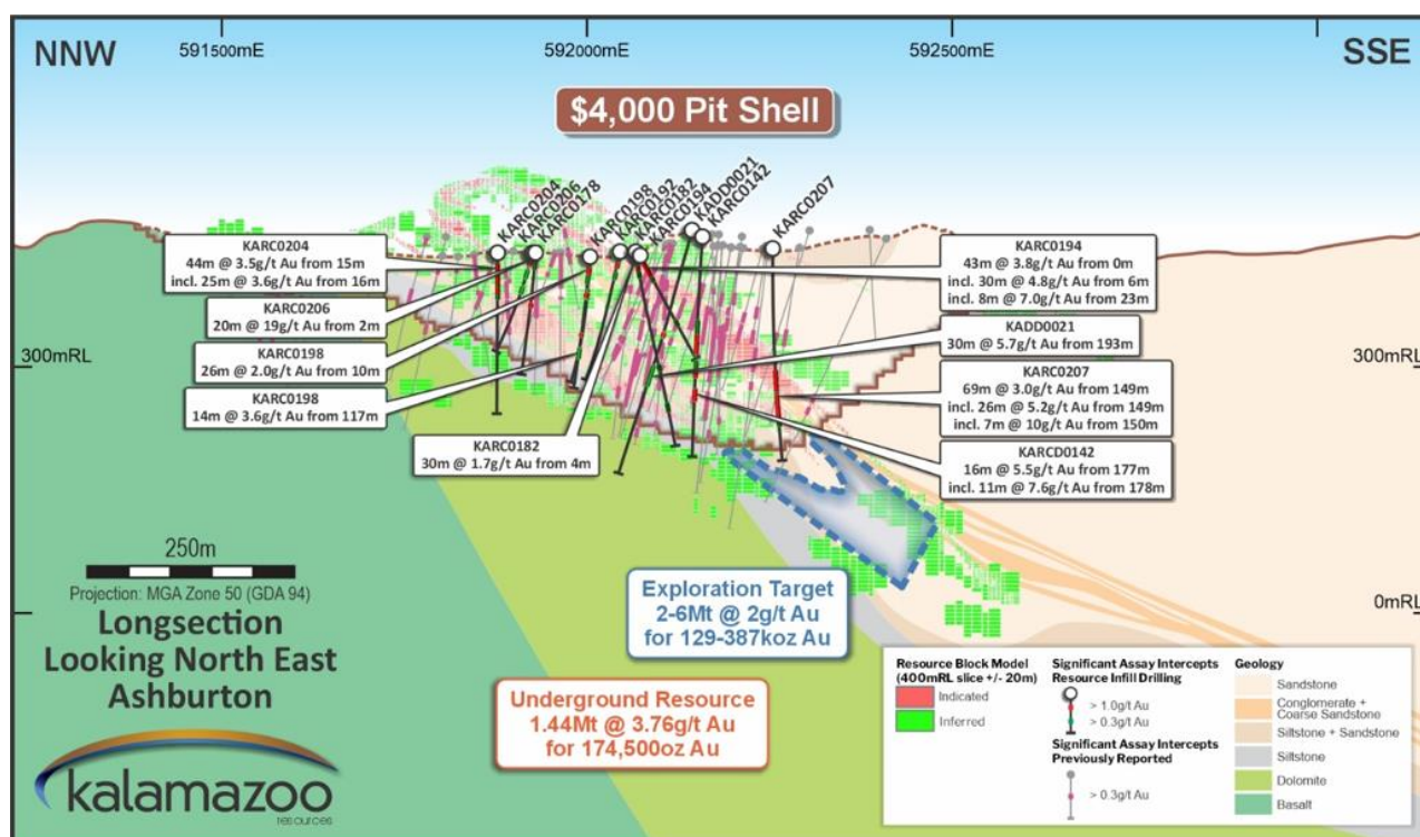
Figure 8: Long section, showing the extent of the current underground resource, and underground growth target, which has been previously reported. The current resource infill drilling program will infill the Indicated and Inferred Mineral Resource, and test the limits of the AUD$4,000 pit shell, where strong mineralisation has been observed in recent growth and historic drilling. The Underground Mineral Resource and Underground Exploration Target have been reported previously
