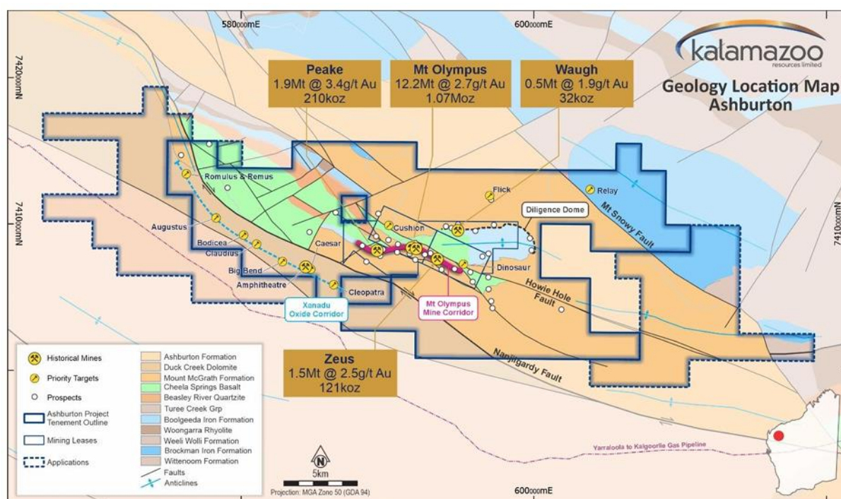
Figure 3: Ashburton Gold Project (blue polygons) geology map showing the location of historical mines, prospects and gold resource estimates and extents of recent tenement applications, which would encompass an expanded footprint of 519km 2 of 100% KZR controlled tenure across the highly prospective Ashburton region
