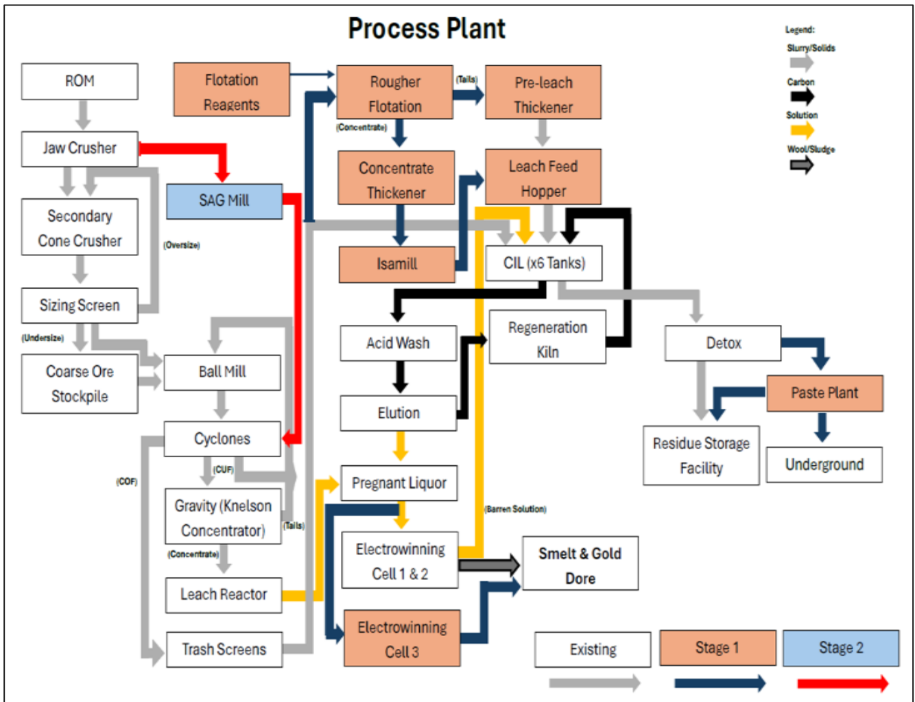
Figure 13-1: Process flowsheet interpreted from Scoping Study engineering
