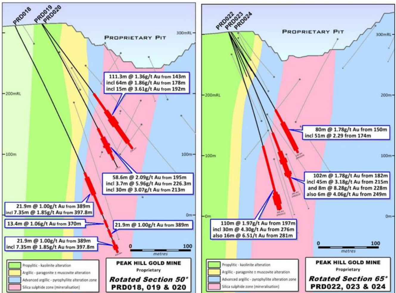
Figure 9-8: Drill sections, Peak Hill 2019 drilling
