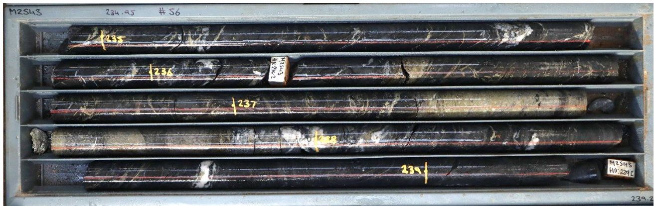
Figure 6. MZS43 237.3 – 238.1m. 0.8m of pyrite-arsenopyrite-tetrahedrite-quartz (Montezuma Lode second intercept).
