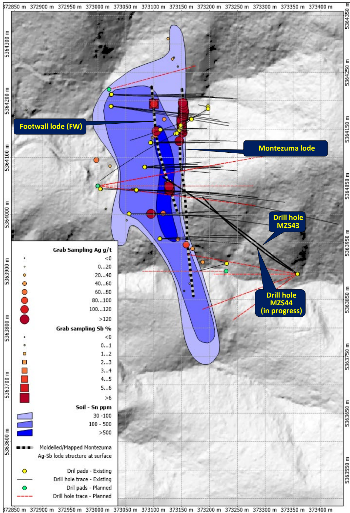
Figure 2 Montezuma Silver & Antimony Project – tin soil anomaly, completed and planned drilling
