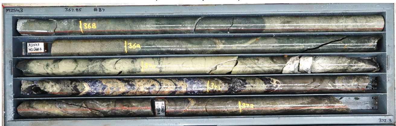
Figure 7. MZS43 370.5 – 372.7m. 2.2m of coarse galena-sphalerite-siderite and pyrite-arsenopyrite-tetrahedrite (Maestries Replacement).
