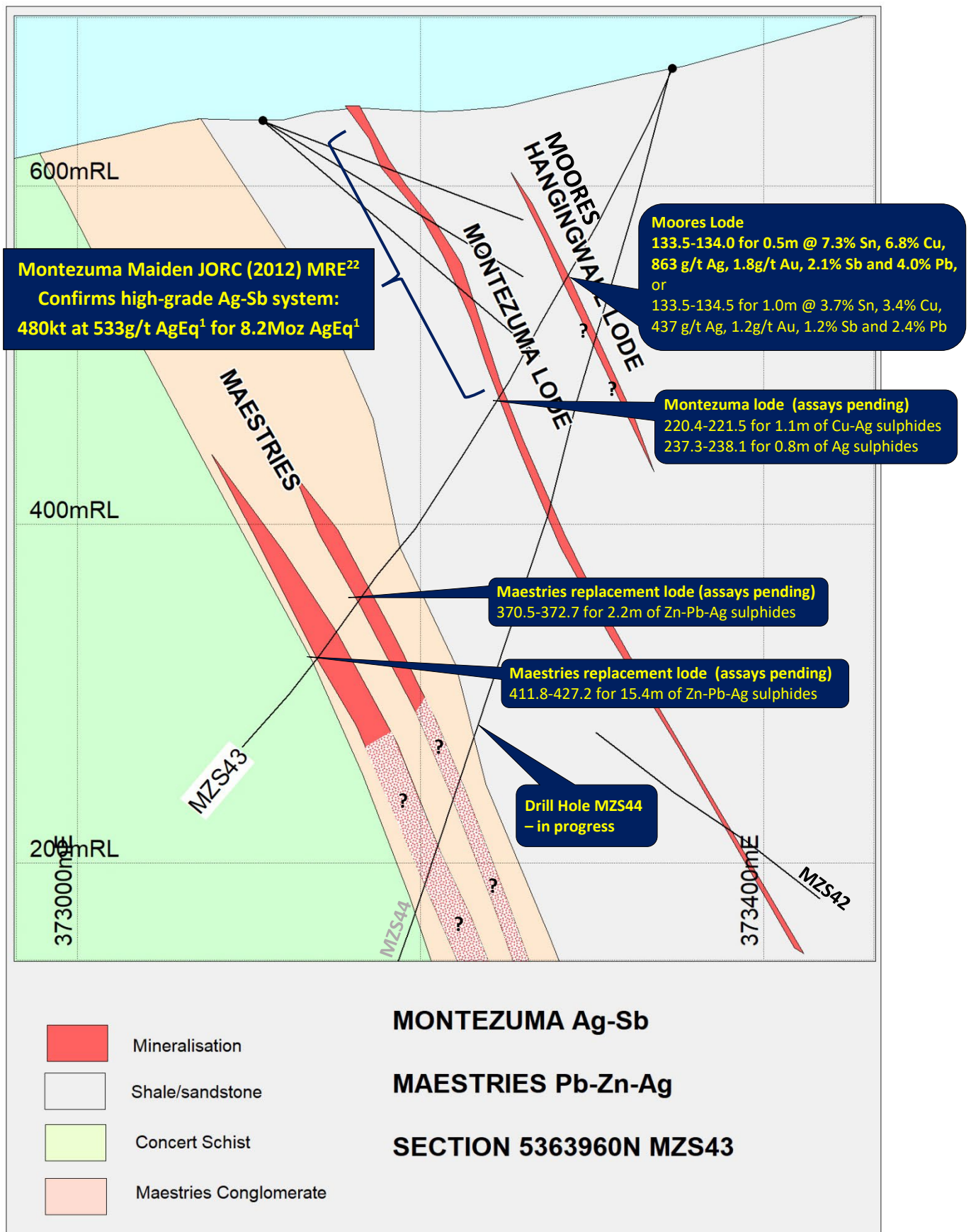
Figure 3 Schematic cross section 5363960N, MZS43 with mineralised intercepts
