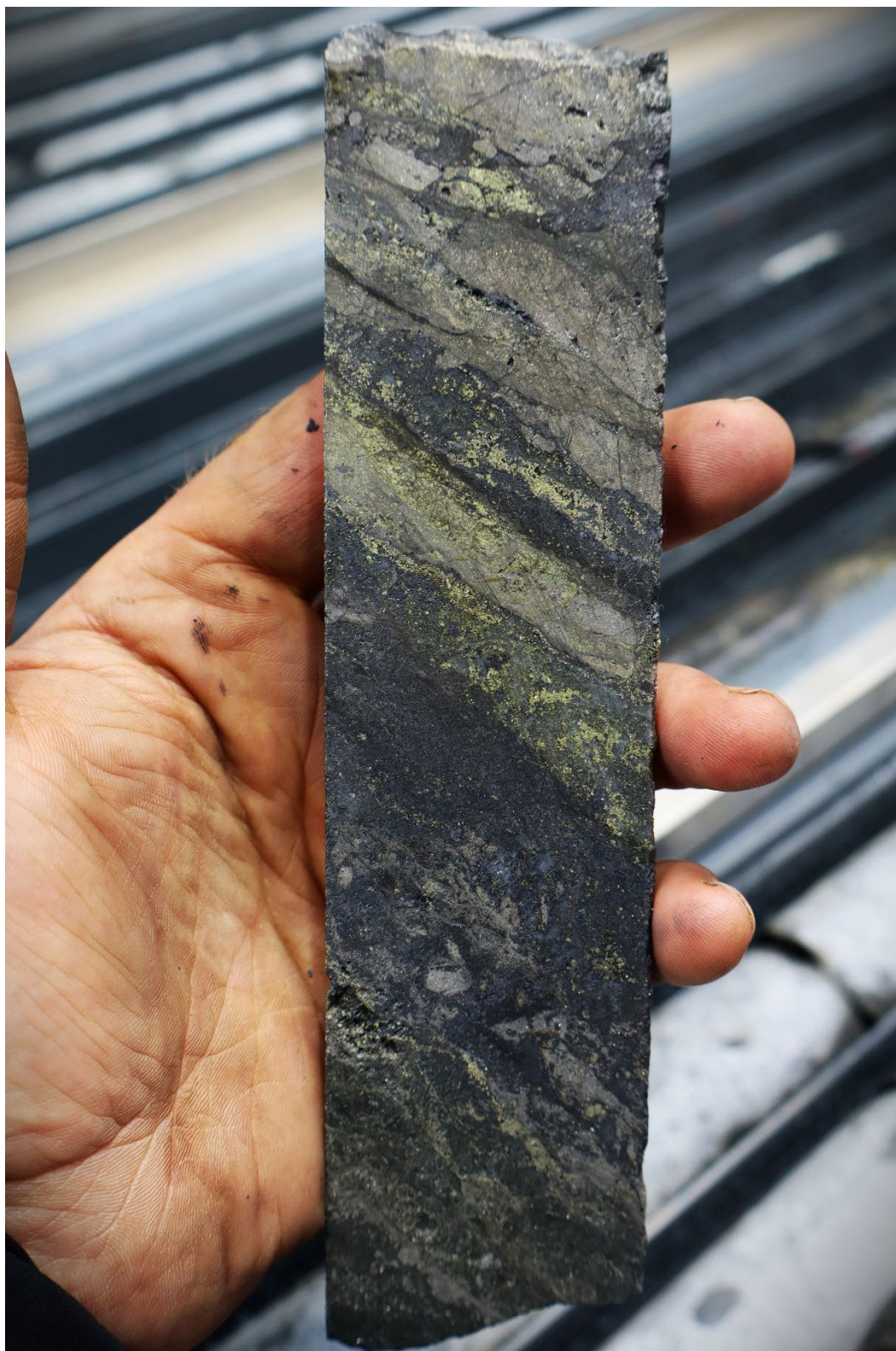
Figure 1 Montezuma hanging wall Moores Lode mineralisation in MZS43
