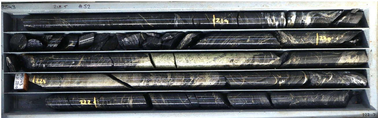
Figure 5. MZS43 220.4 – 221.5m. 1.1m of chalcopyrite-pyrite-arsenopyrite-tetrahedrite (Montezuma Lode first intercept).
