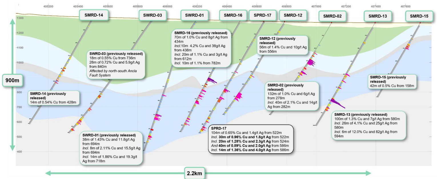
Figure 6: Cross Section Looking North – Pampa Medina 7,440,800 N
