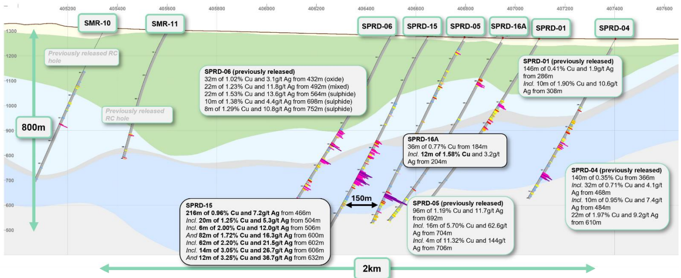
Figure 5: Cross Section Looking North – Pampa Medina 7,440,950 N
