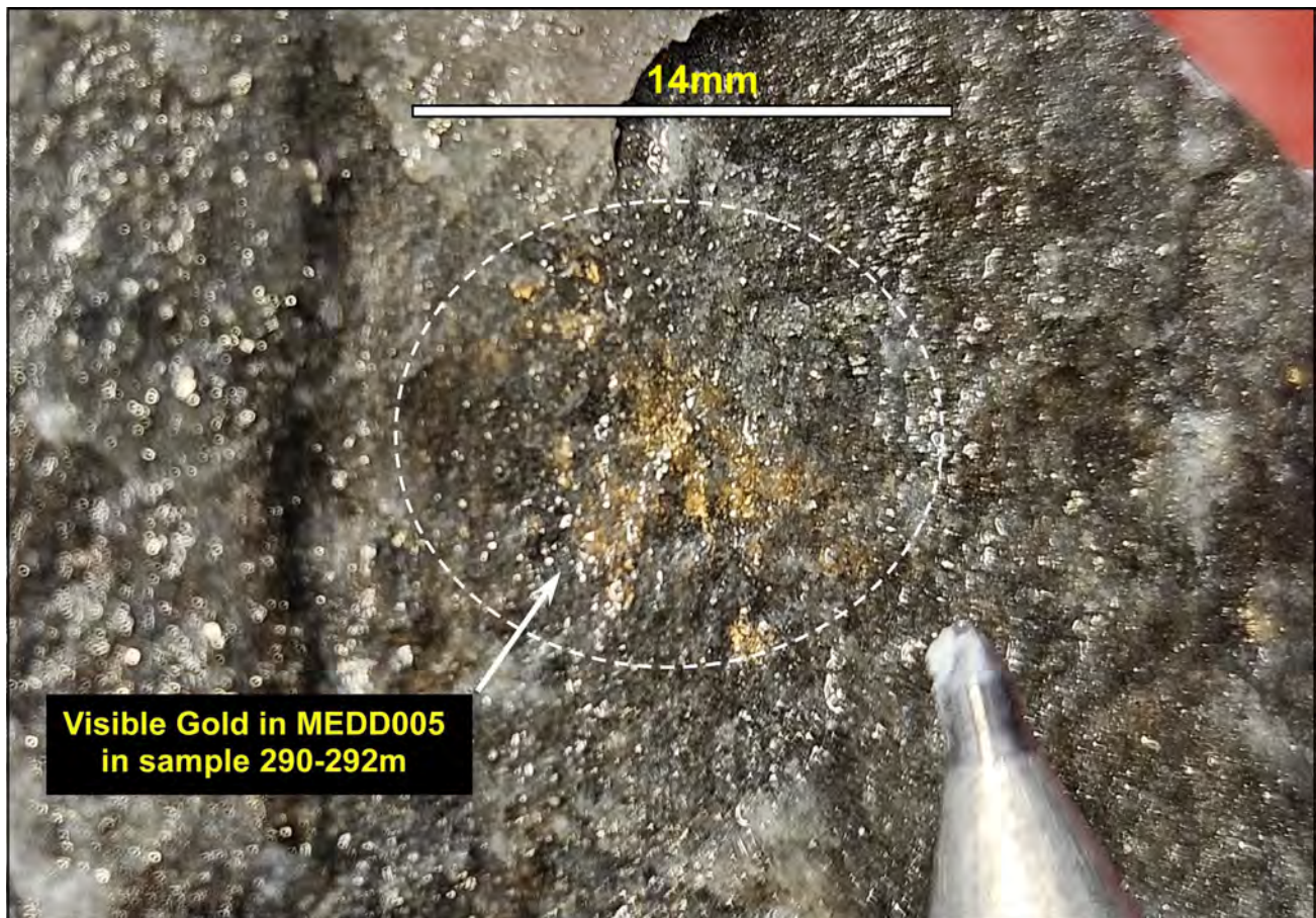
Image 1: Native gold observed along a fracture near the bottom of MEDD005 between 290m and 292m downhole. The broader interval, containing the other half core to this sample, assayed 9.35m @ 17.23 g/t Au-Eq 2 . The gold occurs as fine disseminations along a fracture surface that cuts volcanosedimentary wallrocks to the Melonal porphyry system. Minerals in this interval include native gold (trace quantities <0.01%), chlorite (~10%), anhydrite (~4%) and local andradite garnet (~2%). The remaining mineralogy comprises quartz (~15%) and feldspar (~50%) in siliciclastic, volcanic-derived, finely-bedded tuffaceous sediments. A 20m interval near the bottom of MEDD005 has been re-sampled for repeat assay. Visual estimates of mineral abundance should never be considered a proxy or substitute for laboratory analyses where concentrations or grades are the factor of principal economic interest. Visual estimates also potentially provide no information regarding impurities or deleterious physical properties relevant to valuations.
