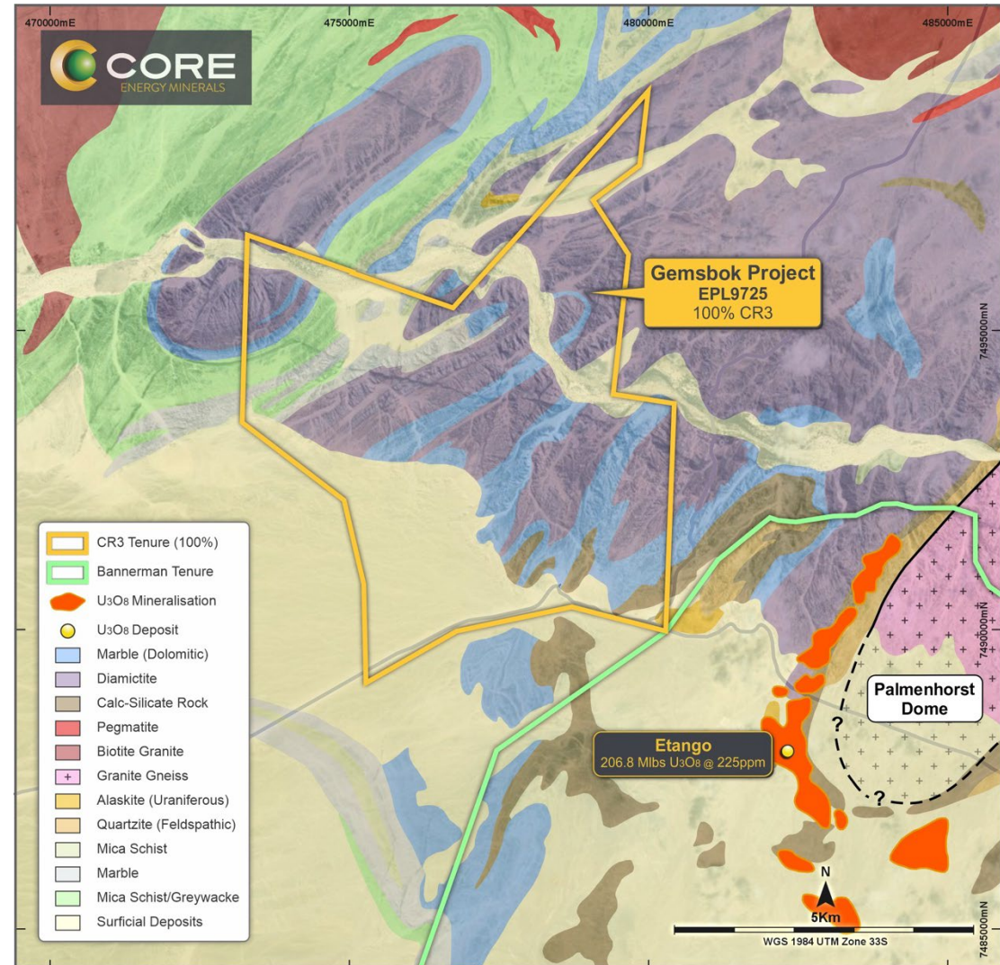
Gemsbok Project with regional geology and neighbouring uranium deposits
