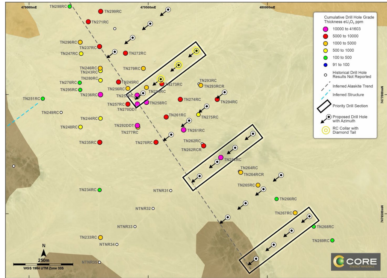
Barking Gecko Prospect: CR3 proposed drill collar plan
