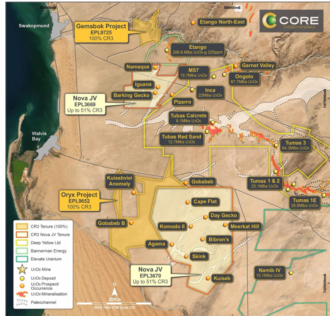
Gemsbok and Oryx locations (100% CR3)
