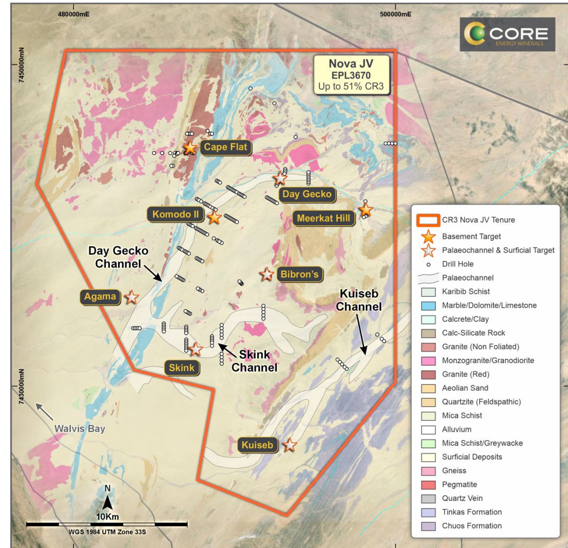
Nova Uranium Project, Additional Targets
