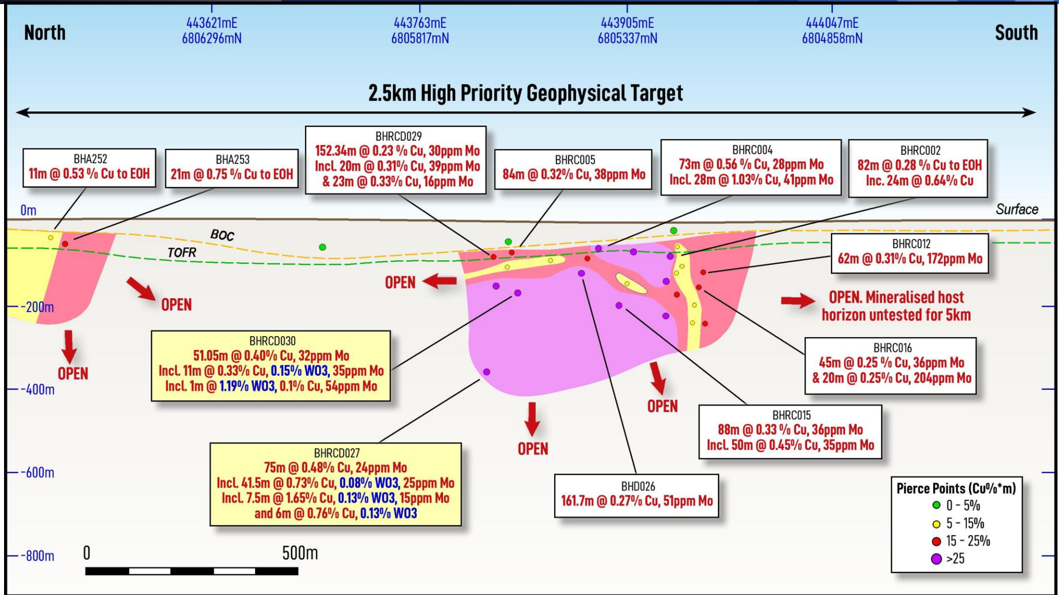
Figure 5 -North-south longsection showing interpreted Cu%Xmeter grade contouring (same yellow, red, purple as per drill hole legend), the 500mX400m extent of known Cu-W-Mo mineralisation identified in previous drilling (centre), the shallow historical aircore drilling located 1km to the north, and the full extent of the 2.5km priority geophysical target.
