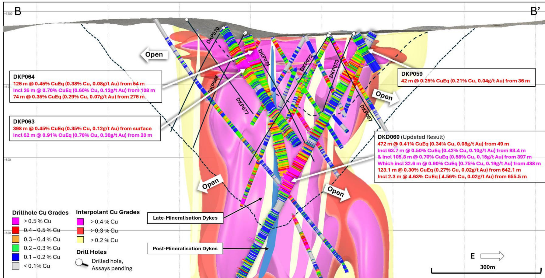
Figure 4. Cross section slice (B – B') showing recent drill hole results DKP063, DKP064, DKP059 and DKD060 ( \pm 75\text{m} clipping) and updated +0.2% copper (yellow), +0.3% copper (red), +0.4% copper (magenta) mineralisation interpolants. Returned Cu grades shown on hole traces, drilled holes with pending assays are shown in black. Conceptual open pit shells 1 displayed for $US3.50/lb Cu (short dash) and $US6.00/lb Cu (long dash) displayed as dashed lines. Results reported including CuEq 2 .
