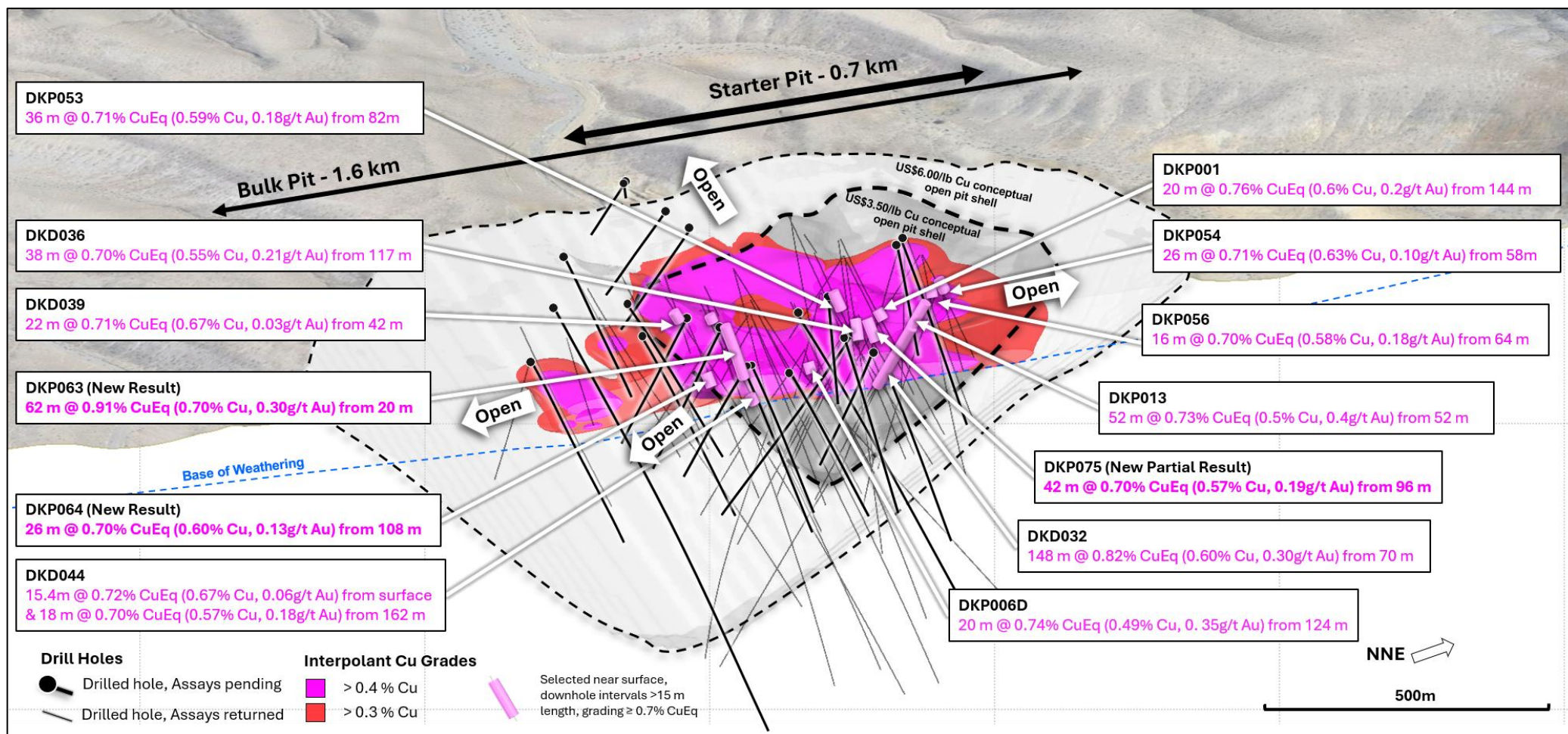
Figure 6. Oblique slice towards NW (Azi 325°, Plunge+26°). 0.3% and 0.4% Cu interpolants displayed for oxide and transitional material, sliced along NNE orientation with the front removed. US$3.50/lb Cu conceptual open pit shell displayed in dark grey; US$6.00/lb Cu conceptual open pit shell displayed in light grey 1 . Base of weathering shown as dashed blue line. Results reported including CuEq 2 .
