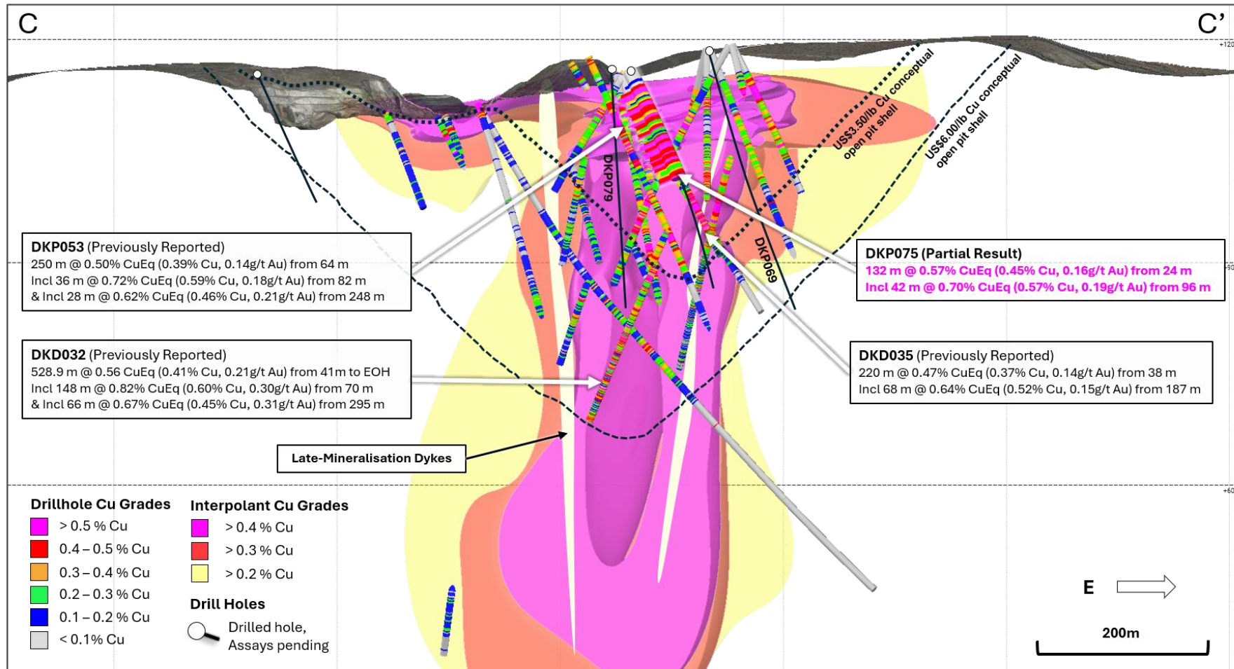
Figure 5. Cross section slice (C – C') showing partial drill hole results DKP075 ( \pm 75\text{m} clipping) and updated +0.2% copper (yellow), +0.3% copper (red), +0.4% copper (magenta) mineralisation interpolants. Returned Cu grades shown on hole traces, drilled holes with pending assays are shown in black. Conceptual open pit shells 1 displayed for $US3.50/lb Cu (short dash) and $US6.00/lb Cu (long dash) displayed as dashed lines. Results reported including CuEq 2 .
