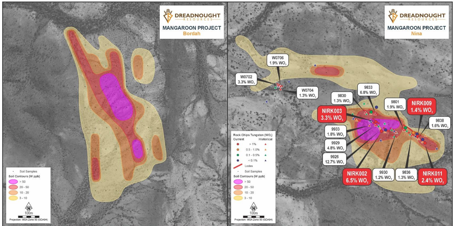
Figure 3: Plan view maps at the same scale comparing the tungsten-in-soil anomaly at Bordah (left) to Nina (right) with the Nina map showing the location of historical and Dreadnought rock chips across the “high-grade” zone.
