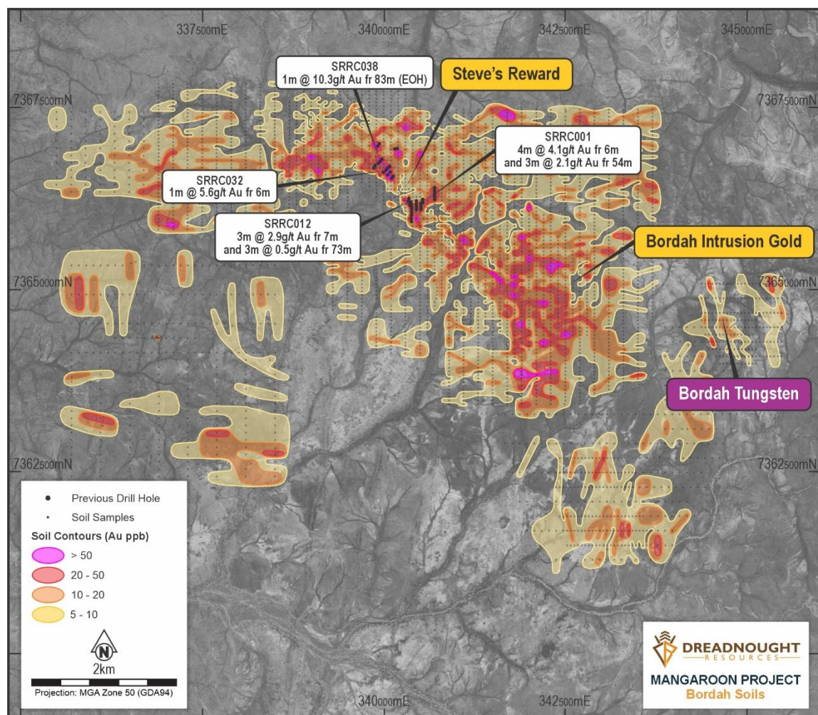
Figure 1: Plan view image of Bordah soils showing the soil sample points and contoured gold-in-soil anomalism in relation to key targets and previous drilling undertaken by Dreadnought.
