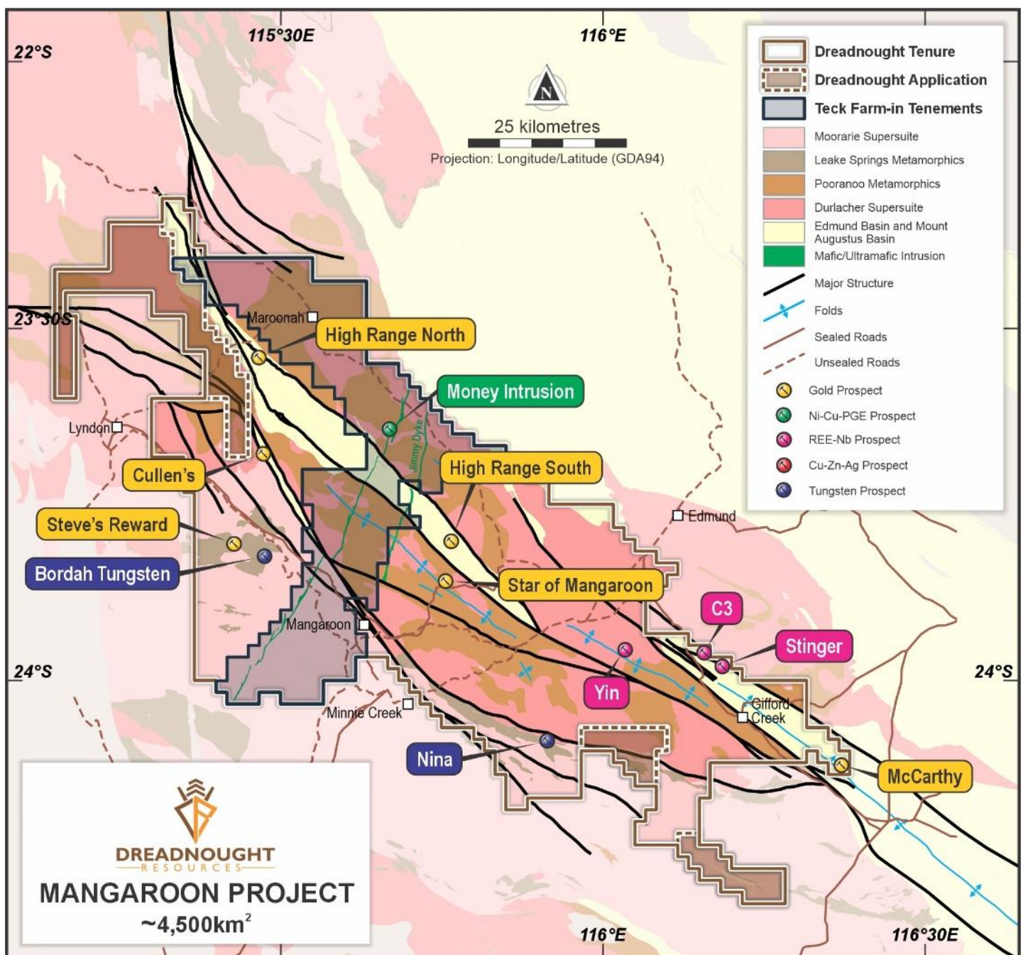
Figure 4: Plan view map of Mangaroon showing the location of major prospects and the Money Intrusion JV.
