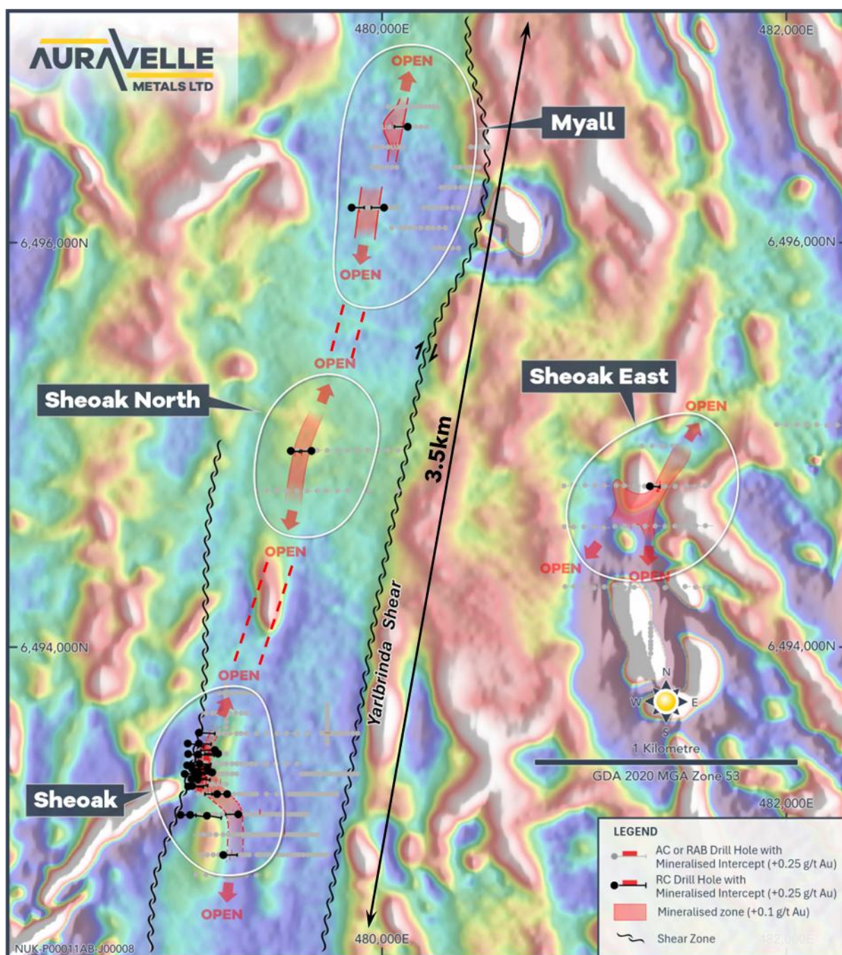
Figure 2: Myall to Sheoak Prospects – Sheoak Anomalous Gold Trend from Drilling over Magnetics 3
