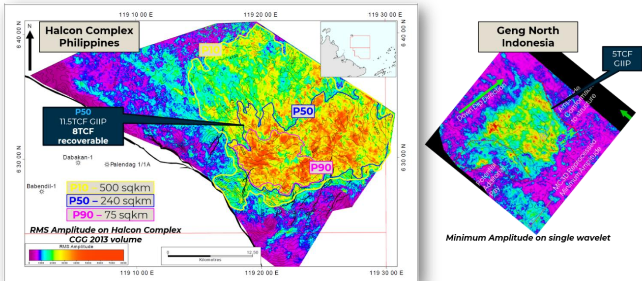
Figure 3 - Seismic amplitude comparisons between recent Geng North discovery made in Kutei basin of Indonesia by ENI and undrilled Halcon prospect in the Philippines, that is the subject of this ASX release. Two maps are at same scale. Image of Geng North is from public source data (Pei et al., 2025, Chasing the Geng North Play, enhancing direct hydrocarbon indicators through 3D seismic reprocessing in the Makassar Straits, 49th Annual IPA convention paper IPA25-G-177)
