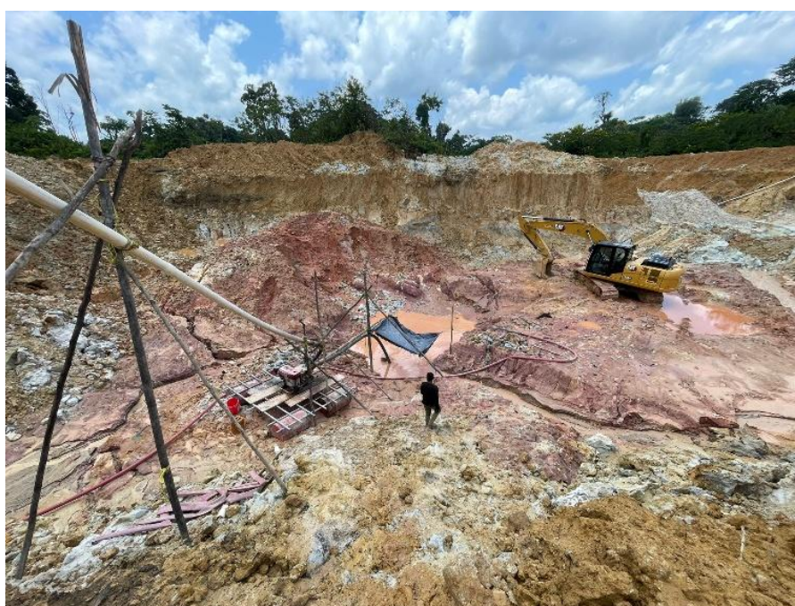
Figure 2: Active workings recovering gold from alluvial and saprolite sources.
