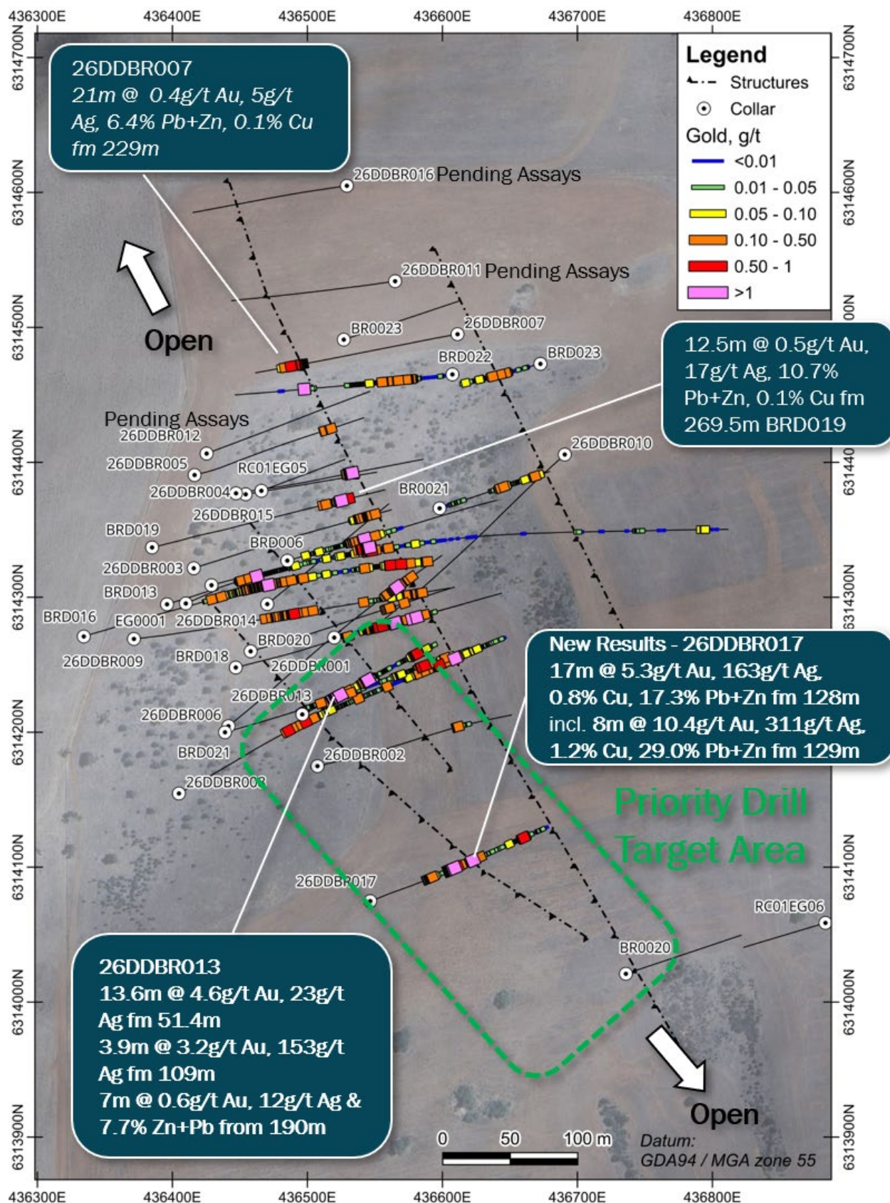
Figure 3: Plan map of current drilling results at Evergreen.
