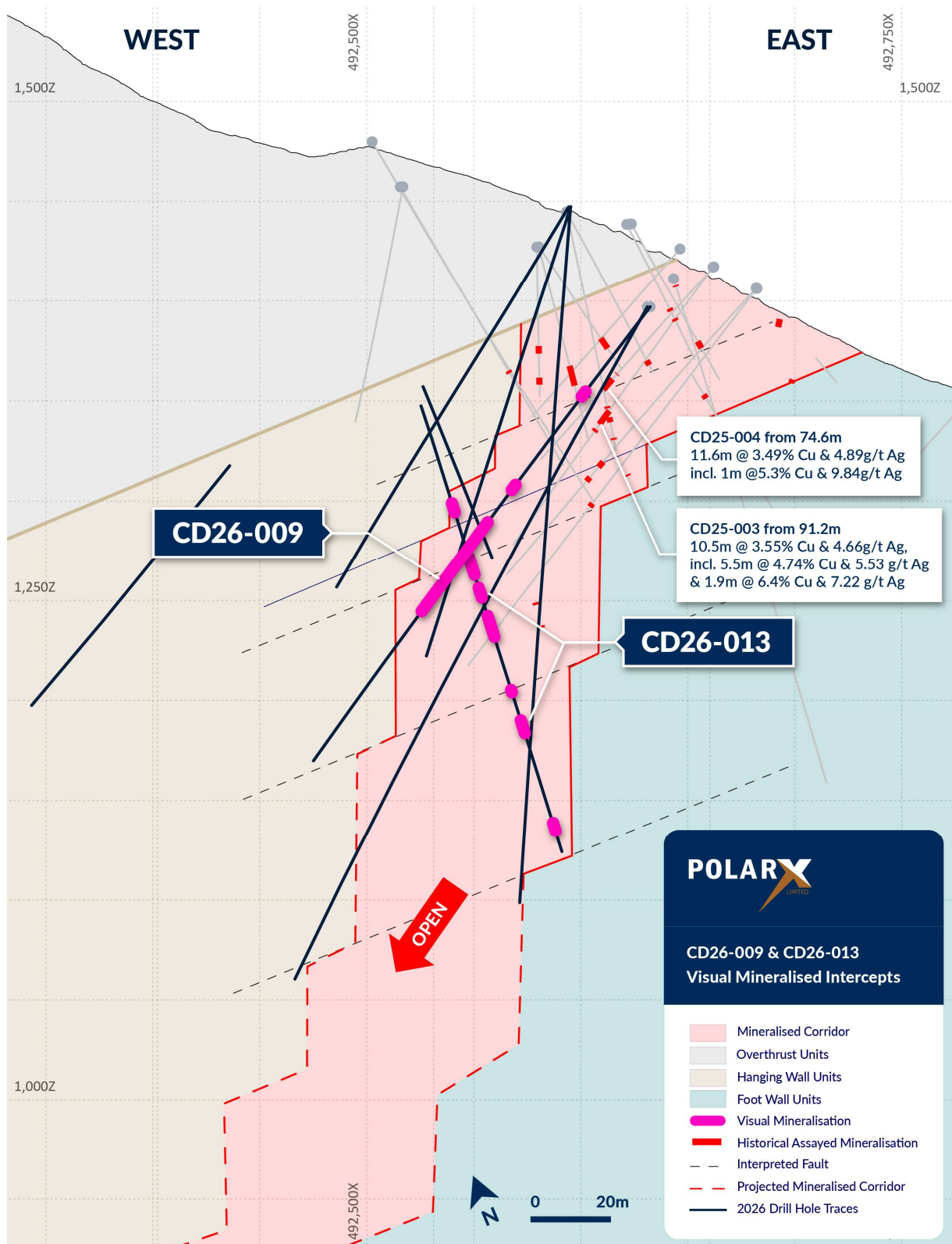
Figure 9. Cross section (286°) for holes CD26-009 and CD26-013 mineralised visual intercepts. The down dip mineralised extents remain open at depth and further to the west.
