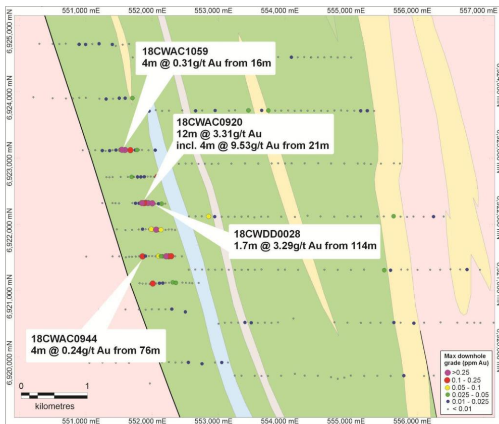
Figure 2: Bloodwood prospect – historical drill hole locations coloured by maximum downhole gold grade, with significant intercepts annotated. Gold anomalism is coherent over approximately 5km of strike.
