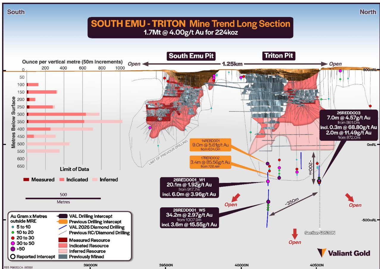
Figure 2: South Emu-Triton Schematic Long Section (facing west) displaying Mineral Resource inventory (MRE) 1 with ounce per vertical metre breakdown, previously mined volumes and Gram.Metre intersections outside the MRE.
