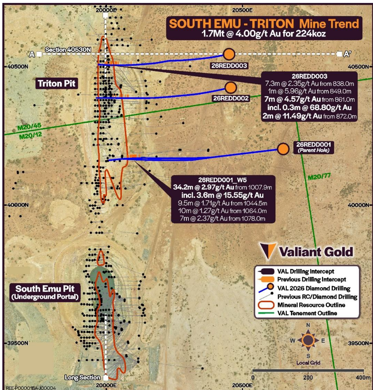
Figure 3: South Emu-Triton Plan view map, displaying MRE Outline 1 , previous drilling, South Emu-Triton pits and Valiant recent drill traces. Presented schematic long section and cross section location is labelled.
