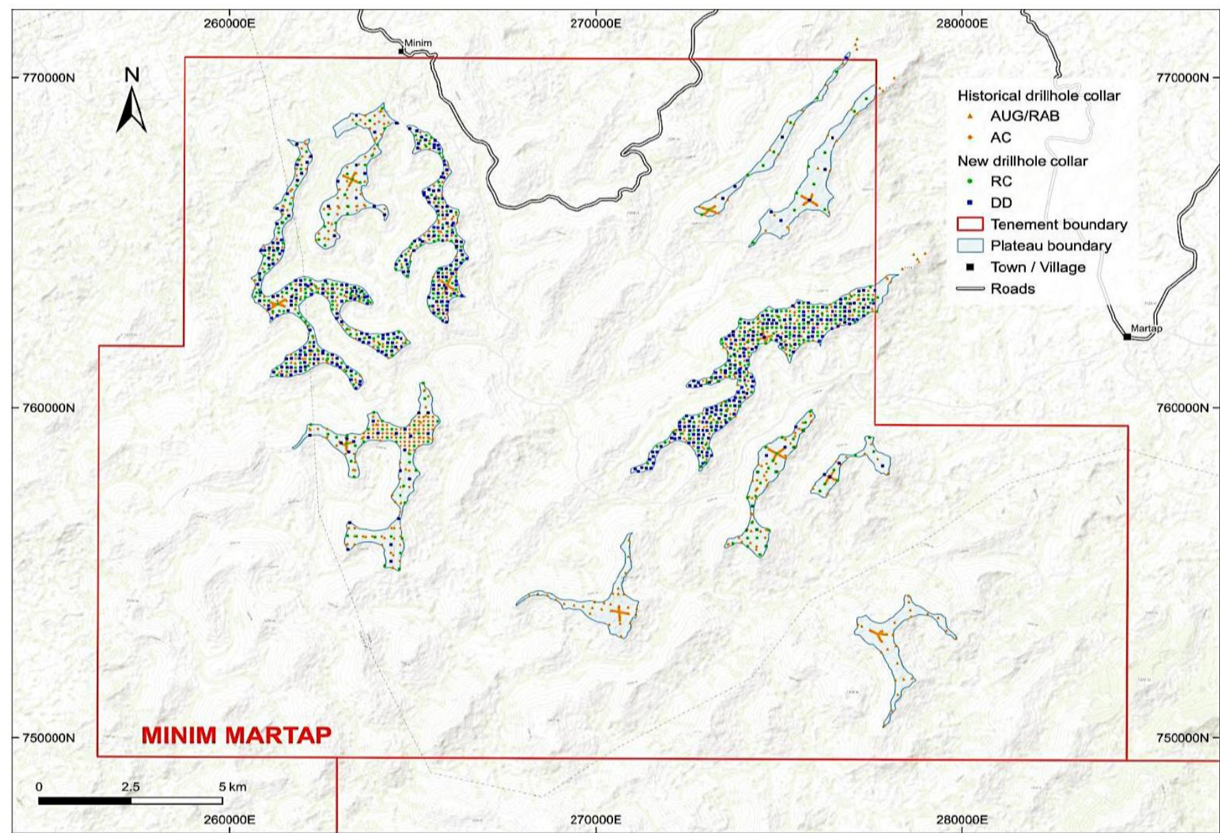
Figure 5-1: Drill hole locations - Minim Martap licence
