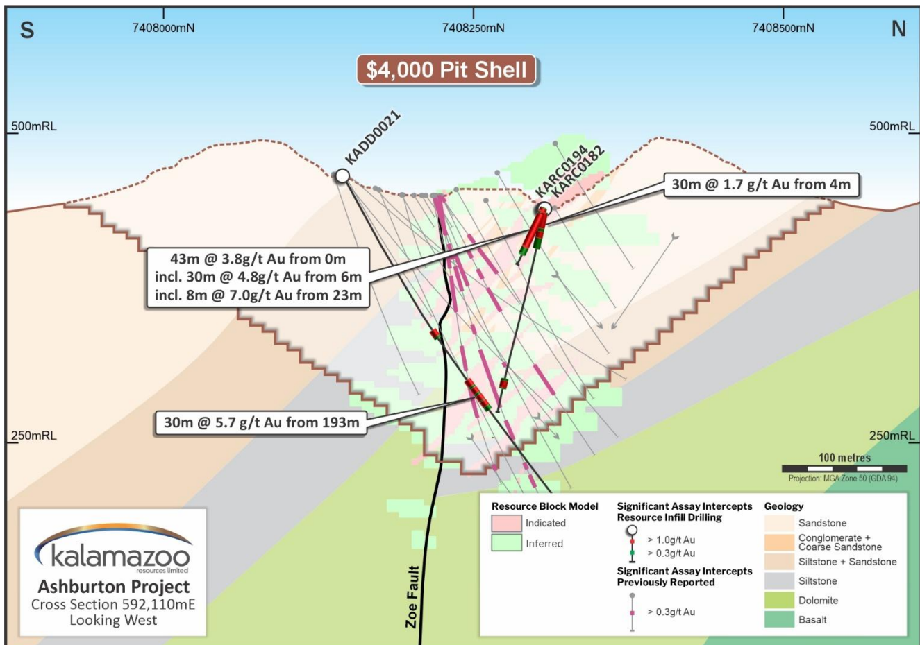
Figure 5: Mt Olympus cross section 592110mE looking west and centred on drill hole KADD0021 section showing drill traces and significant assay intercepts from recent Resource Definition Drilling. Current Mineral Resource outlines (red and green) and the Scoping Study AUD$4,000/oz pit shell design (brown outline) are shown.
